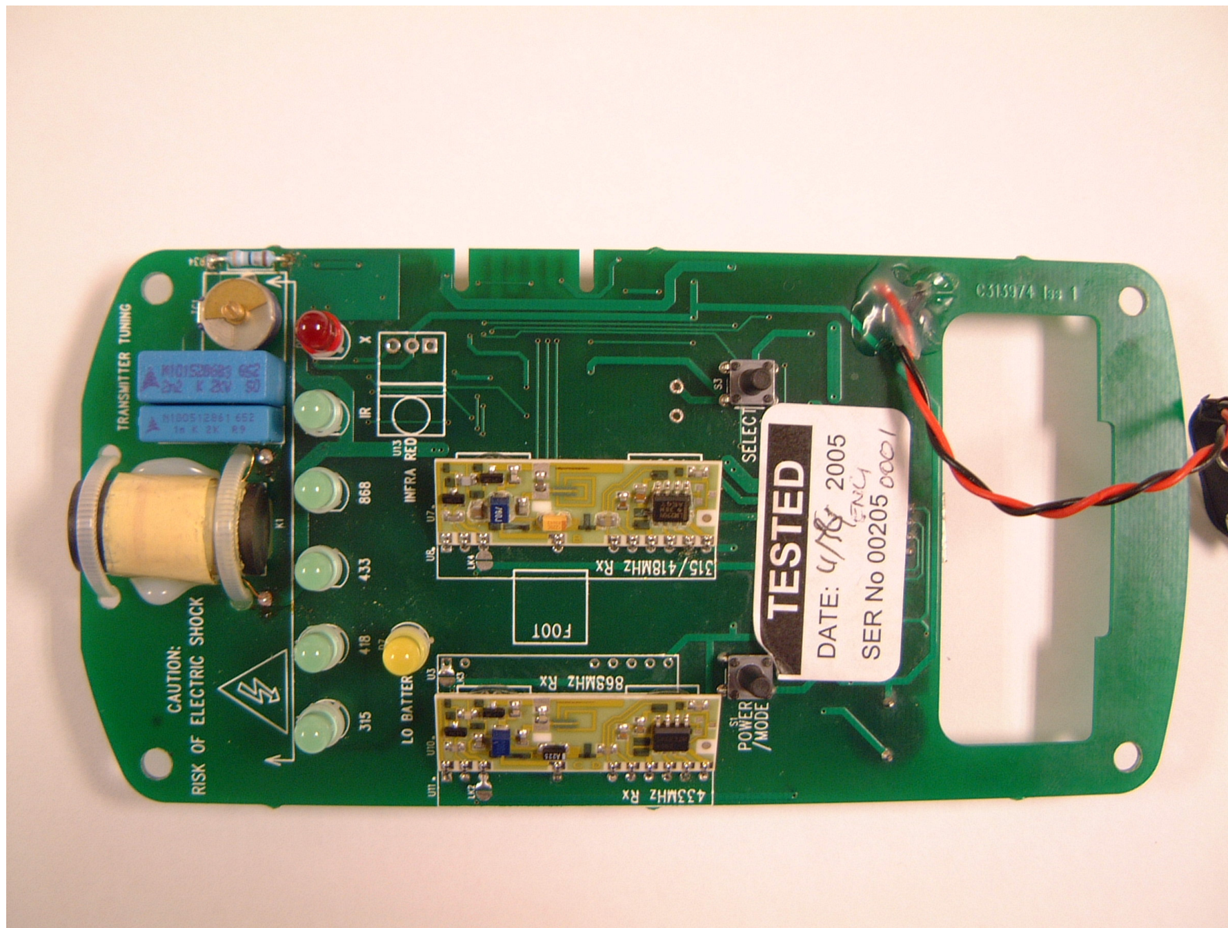
OmiDetect 100 Internal Photograph – PCB Front
