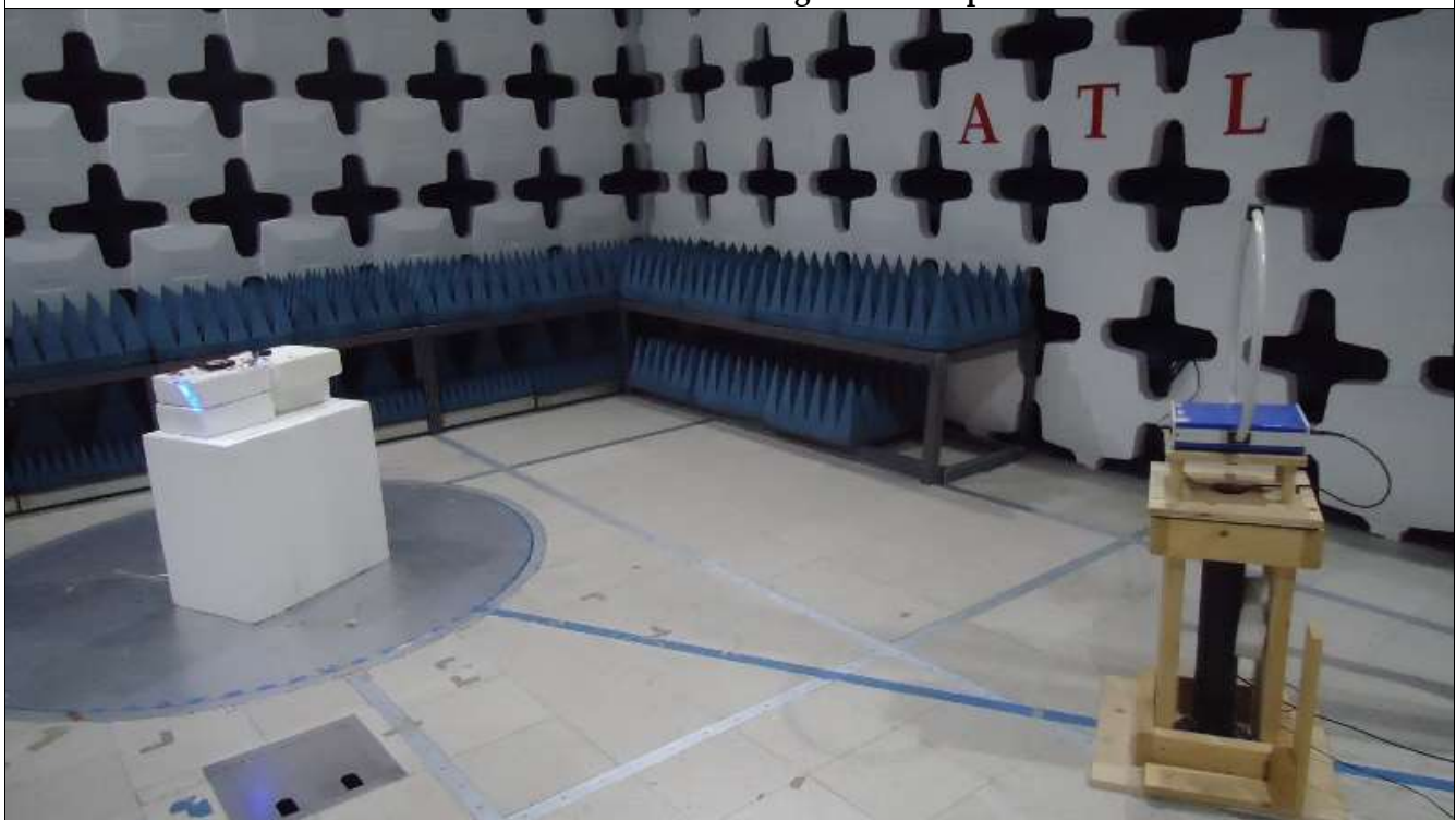
Transmitter Fundamental Field Strength Test Setup - Side View
