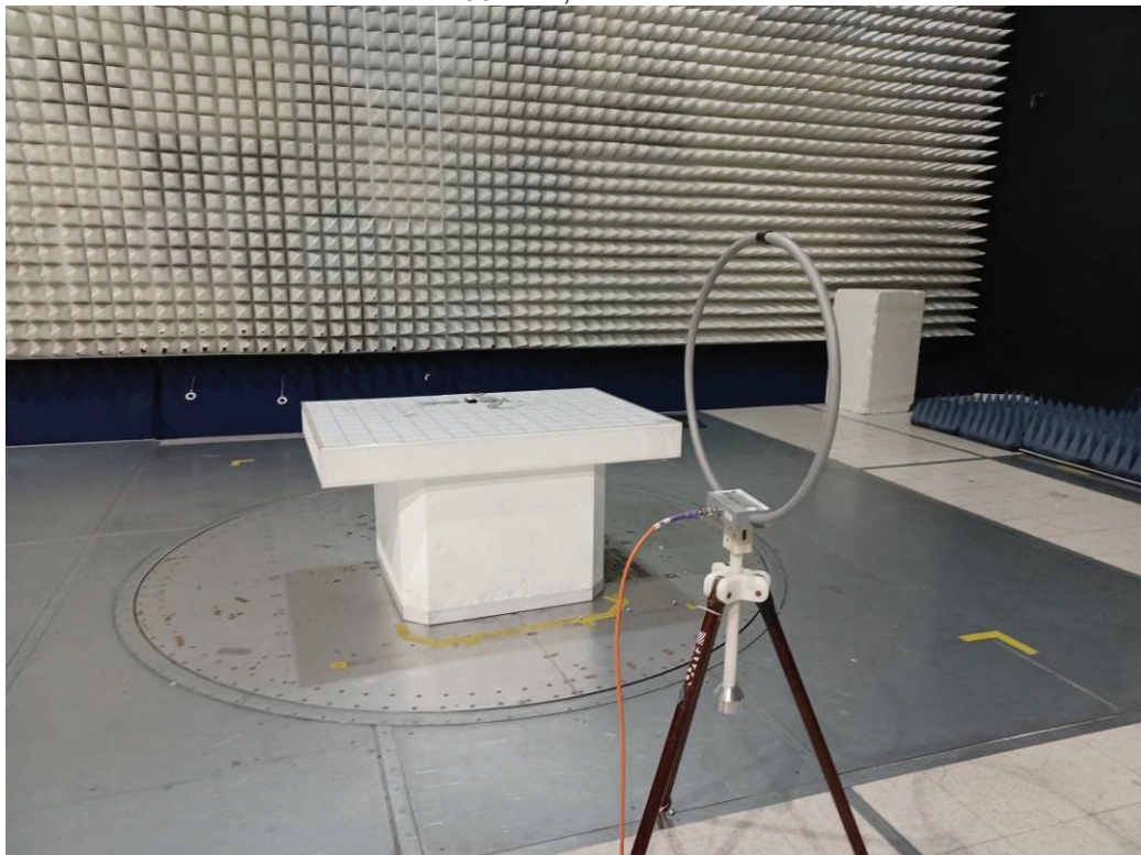
Below 30 MHz, Y-Axis Antenna
