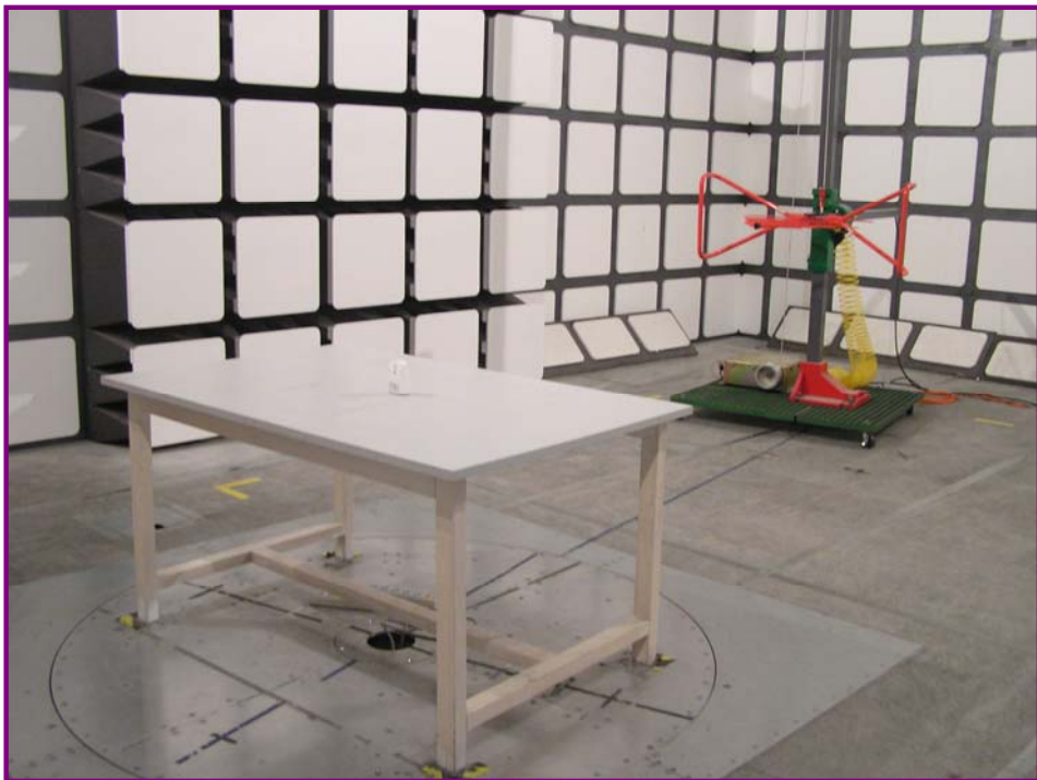
Radiated Emission – Rear View (30-1000MHz)
