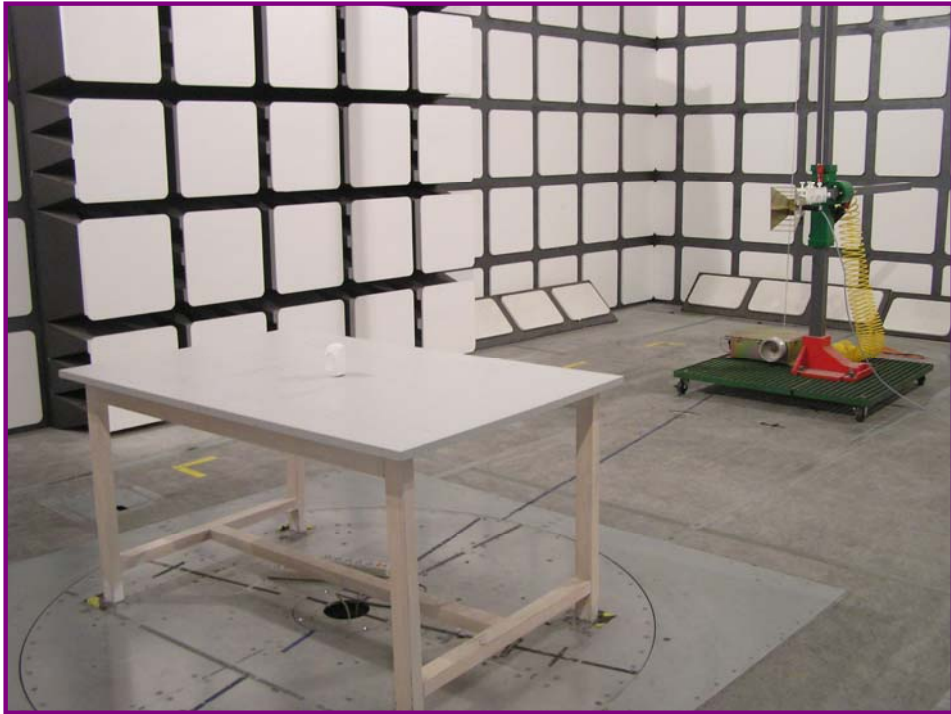
Radiated Emission - Front View (Above 1000MHz)
