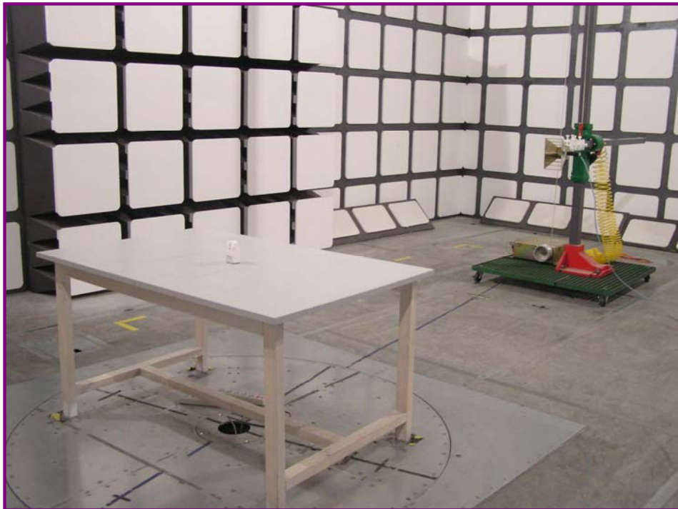
Radiated Emission - Rear View (Above 1000MHz)
