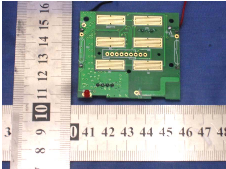
PCB-Back View
