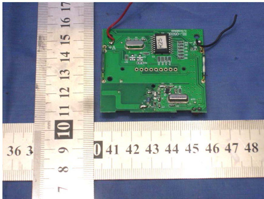
PCB-Front View
