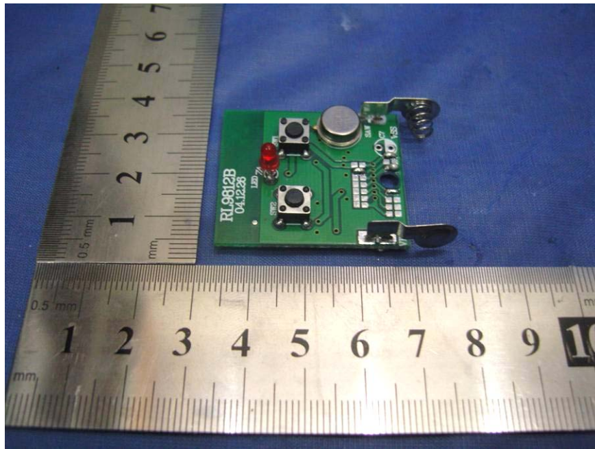
PCB-Back View
