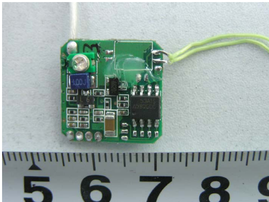
EUT- RF PCB Top view
