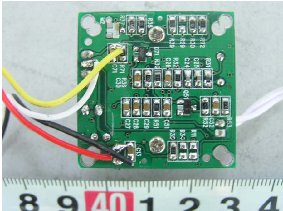
EUT- Digital PCB Bottom View
