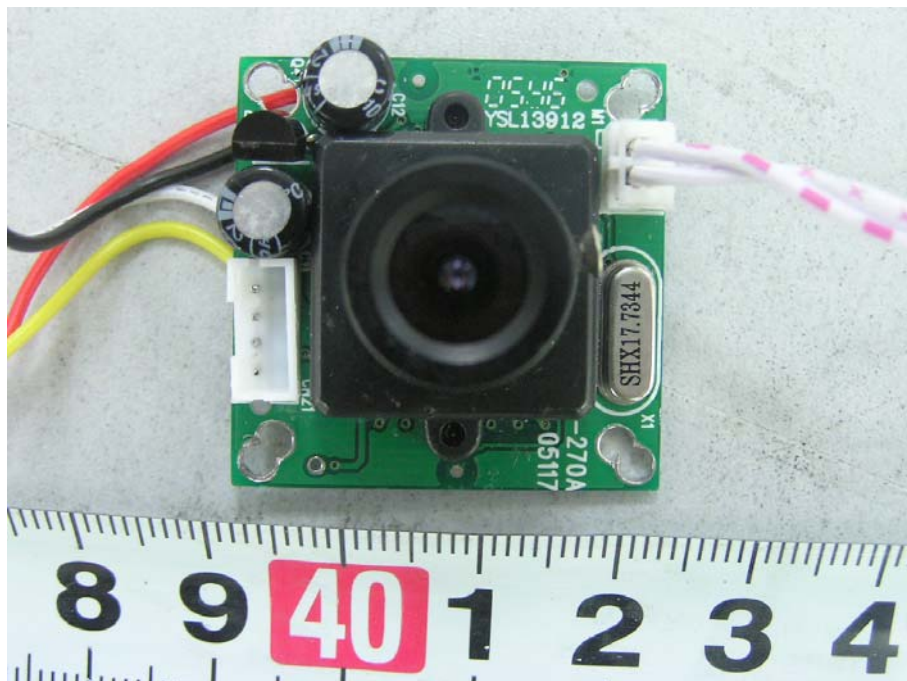
EUT- Digital PCB Top View
