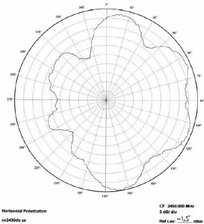
Figure 6. XZ Plane-Horizontal Polarization
