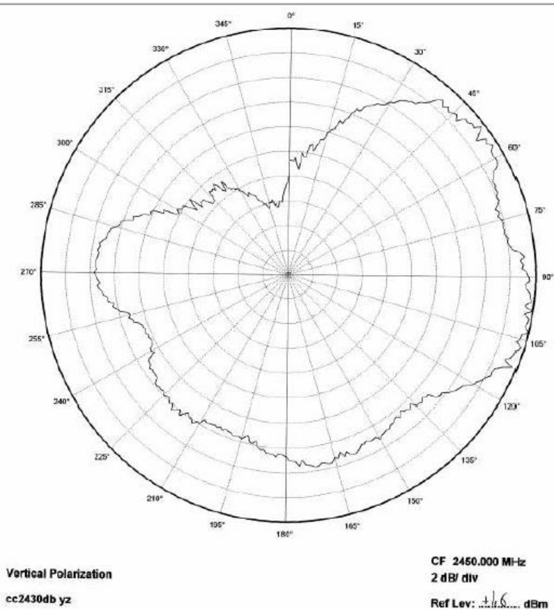
Figure 7. YZ Plane–Vertical Polarization
