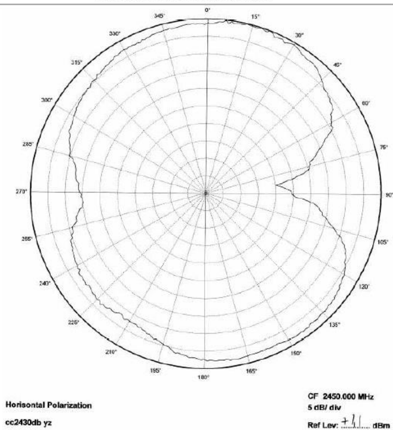
Figure 8. YZ Plane–Horizontal Polarization
