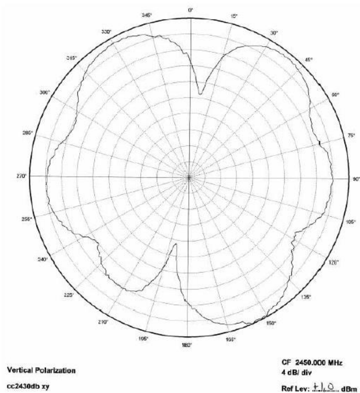
Figure 3. XY Plane-Vertical Polarization
