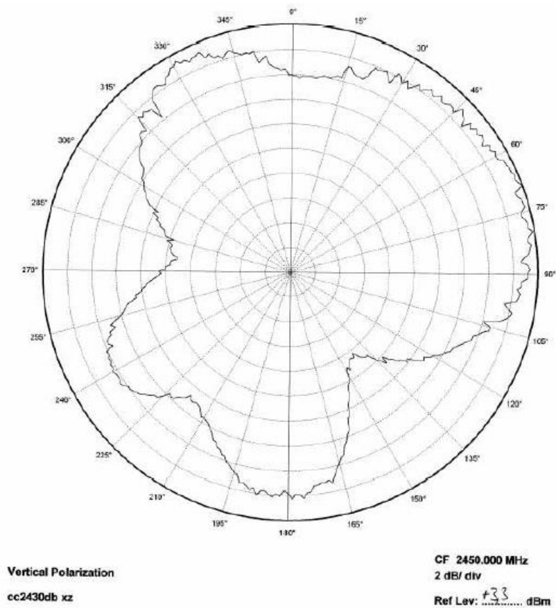
Figure 5. XZ Plane-Vertical Polarization
