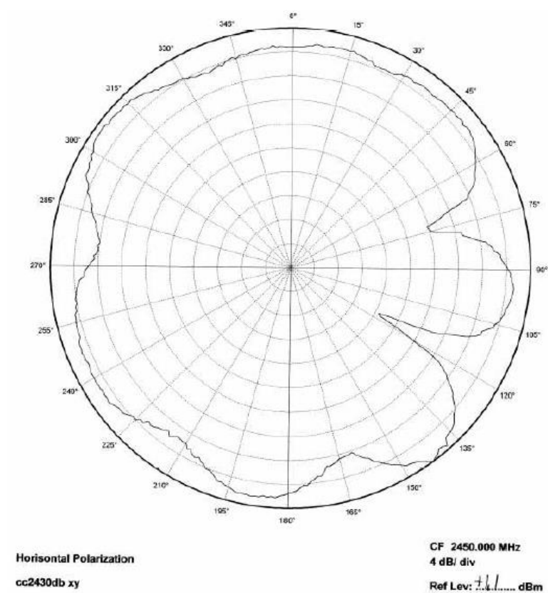
Figure 4. XY Plane-Horizontal Polarization
