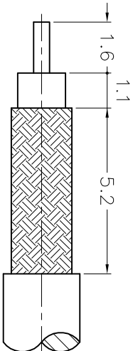
RECOMMENDED CABLE STRIPPING DIM'S (建議剝線尺寸)
