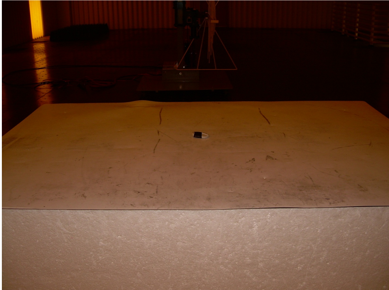
Photograph 1 – Radiated Disturbance Setup – Horizontal Placement
