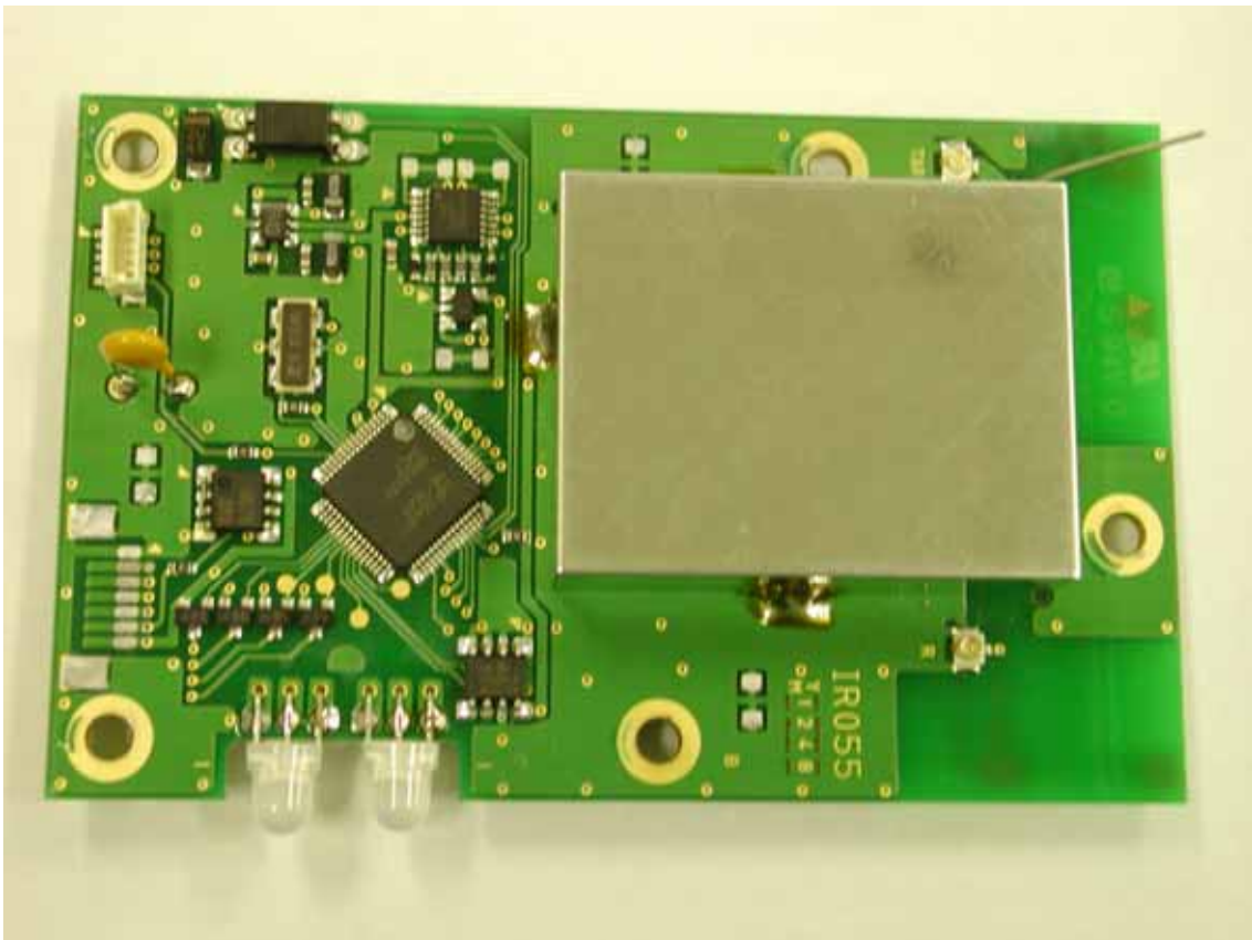
Internal Photo 1 Receiver Model RCSFR1
