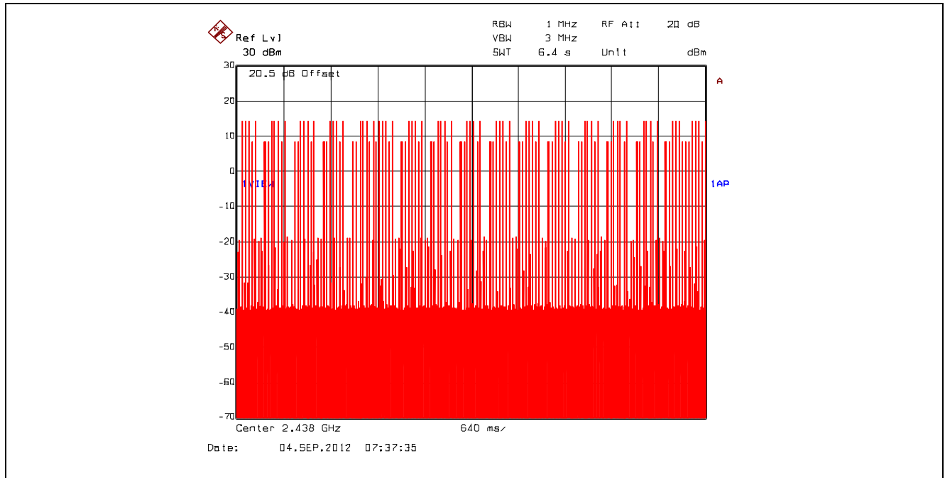
Plot 5.3.4.19. Time of Occupancy, 2438 MHz, 16-QAM, Dwell Time @ 2438 MHz = 190.380762 \mu s
