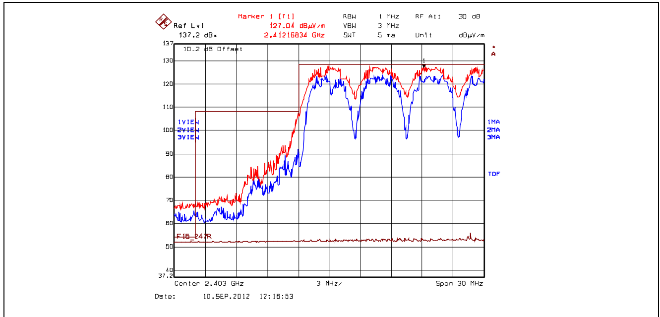
Plot 5.6.4.2.9. Band-Edge RF Radiated Emissions at 3 m, Vertical Polarization Lower Band-edge, Hopping Mode, Power Setting 8, 16-QAM
