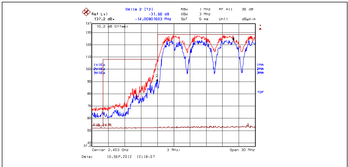
Plot 5.6.4.2.10. Band-Edge RF Radiated Emissions at 3 m, Vertical Polarization Lower Band-edge, Hopping Mode, Power Setting 8, 16-QAM
