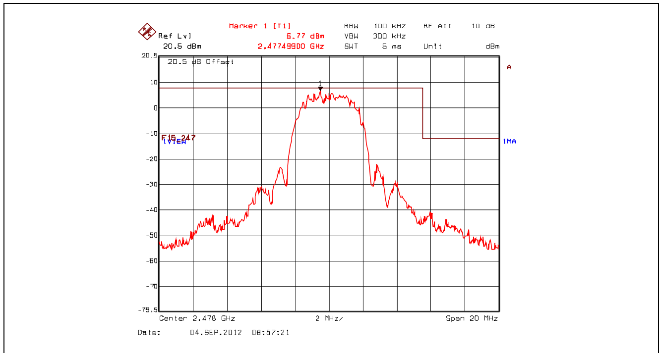
Plot 5.5.4.1.11. Band-Edge RF Conducted Emissions, Upper Band-edge, Single Frequency Mode, QPSK
