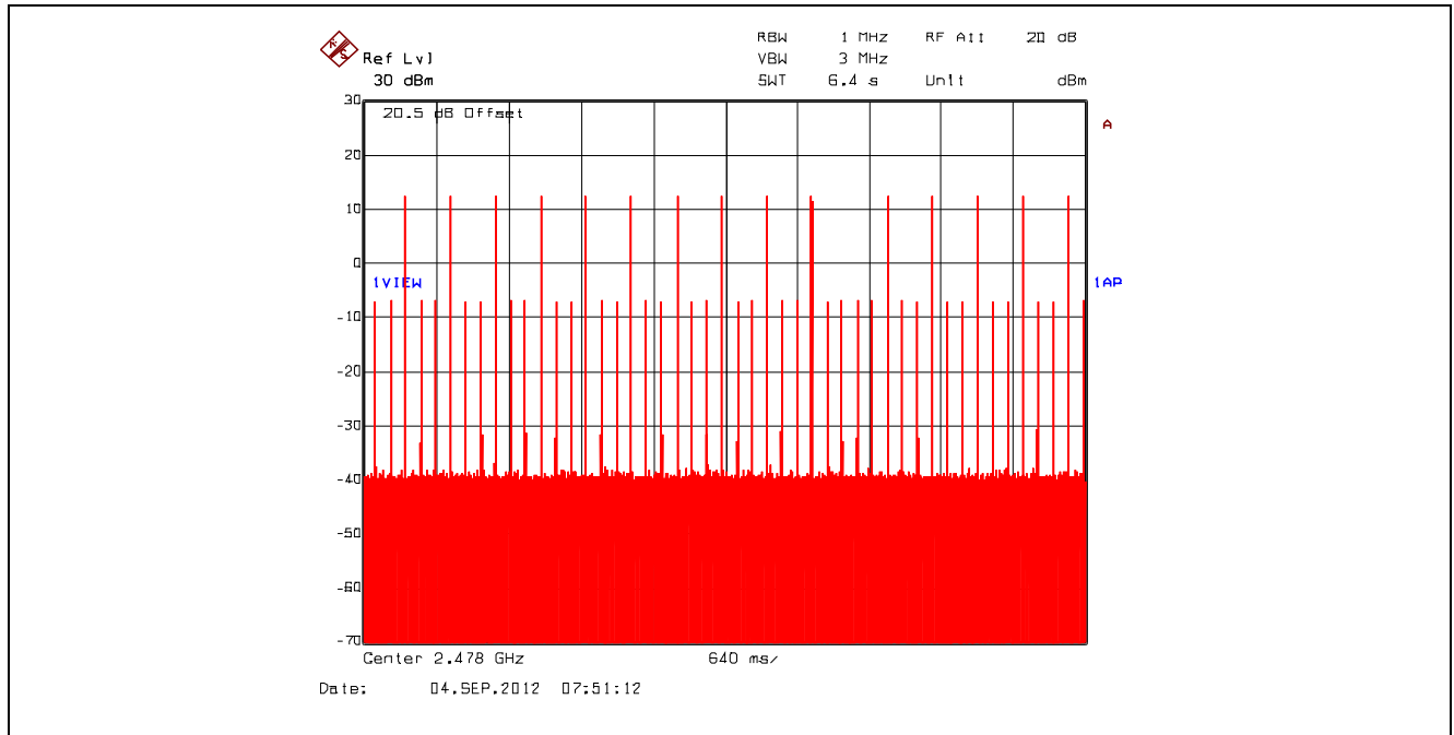
Plot 5.3.4.33. Time of Occupancy, 2478 MHz, QPSK, Dwell Time @ 2478 MHz = 210.420842 µs
