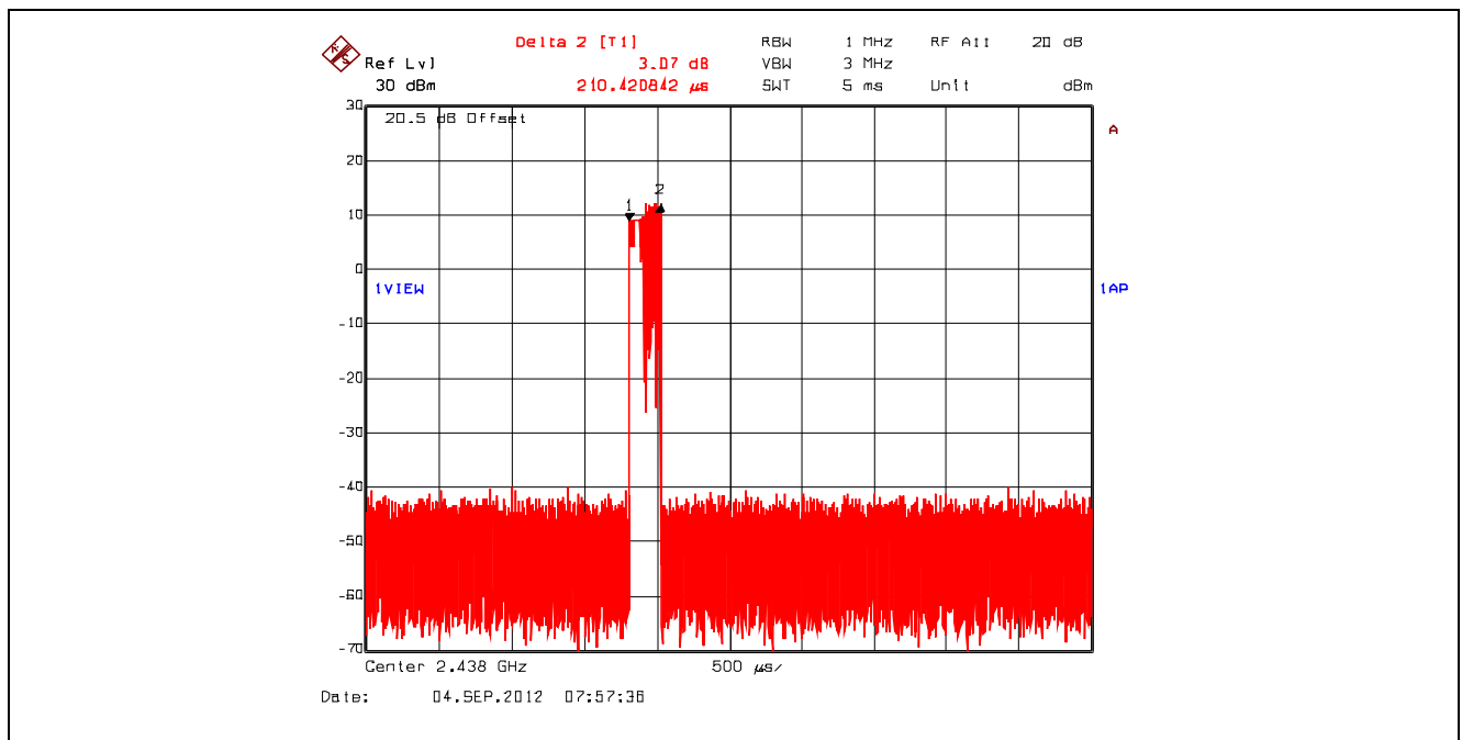
Plot 5.3.4.31. Time of Occupancy, 2438 MHz, QPSK, Dwell Time @ 2438 MHz = 210.420842 \mu s
