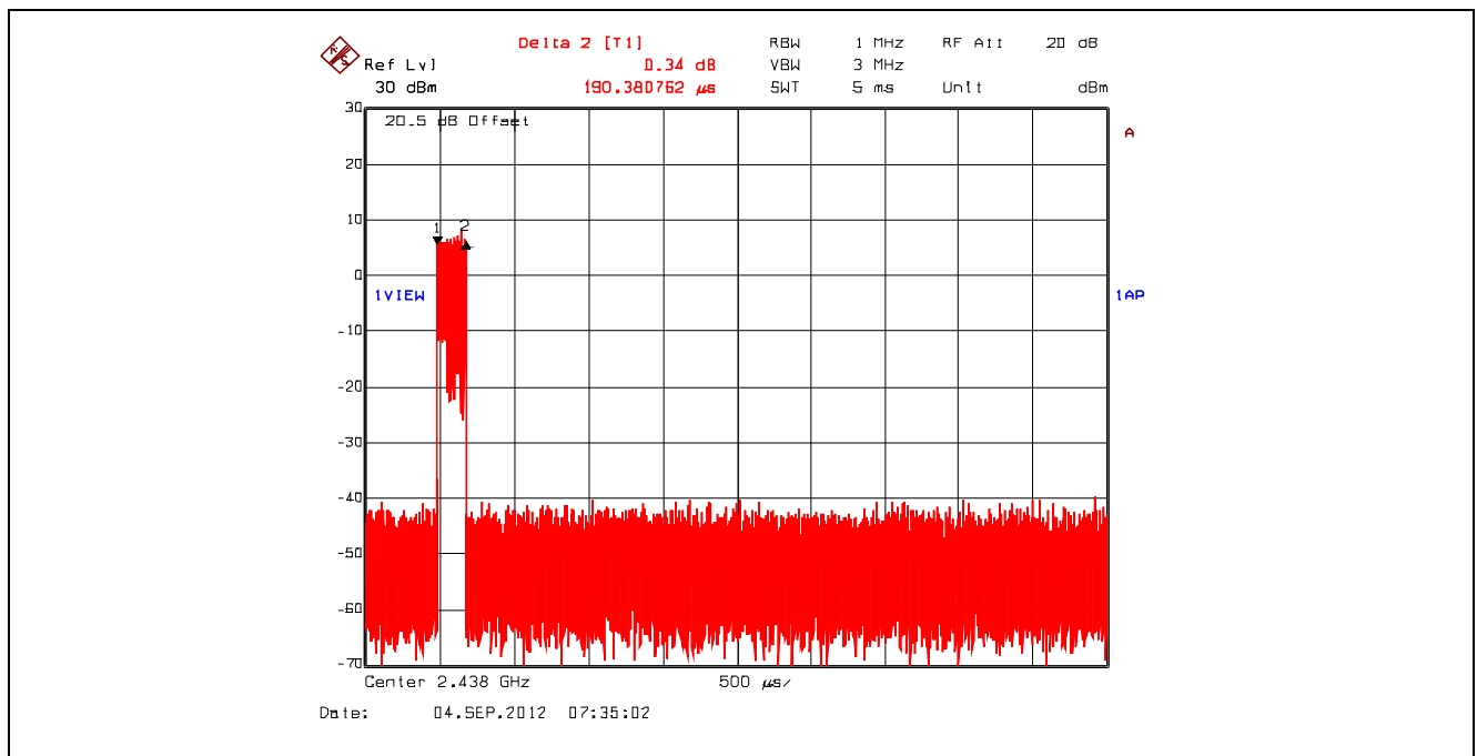
Plot 5.3.4.19. Time of Occupancy, 2438 MHz, 16-QAM, Dwell Time @ 2438 MHz = 190.380762 \mu s
