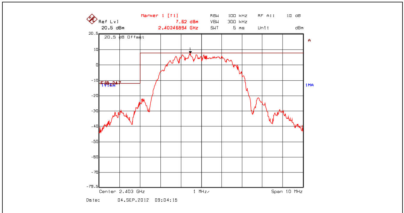
Plot 5.5.4.1.9. Band-Edge RF Conducted Emissions, Lower Band-edge, Single Frequency Mode, QPSK
