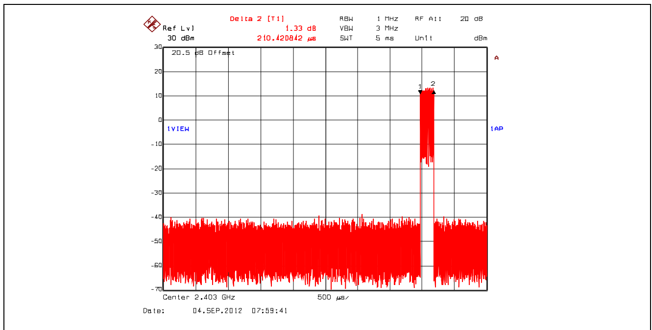
Plot 5.3.4.29. Time of Occupancy, 2403 MHz, QPSK, Dwell Time @ 2403 MHz = 210.420842 µs
