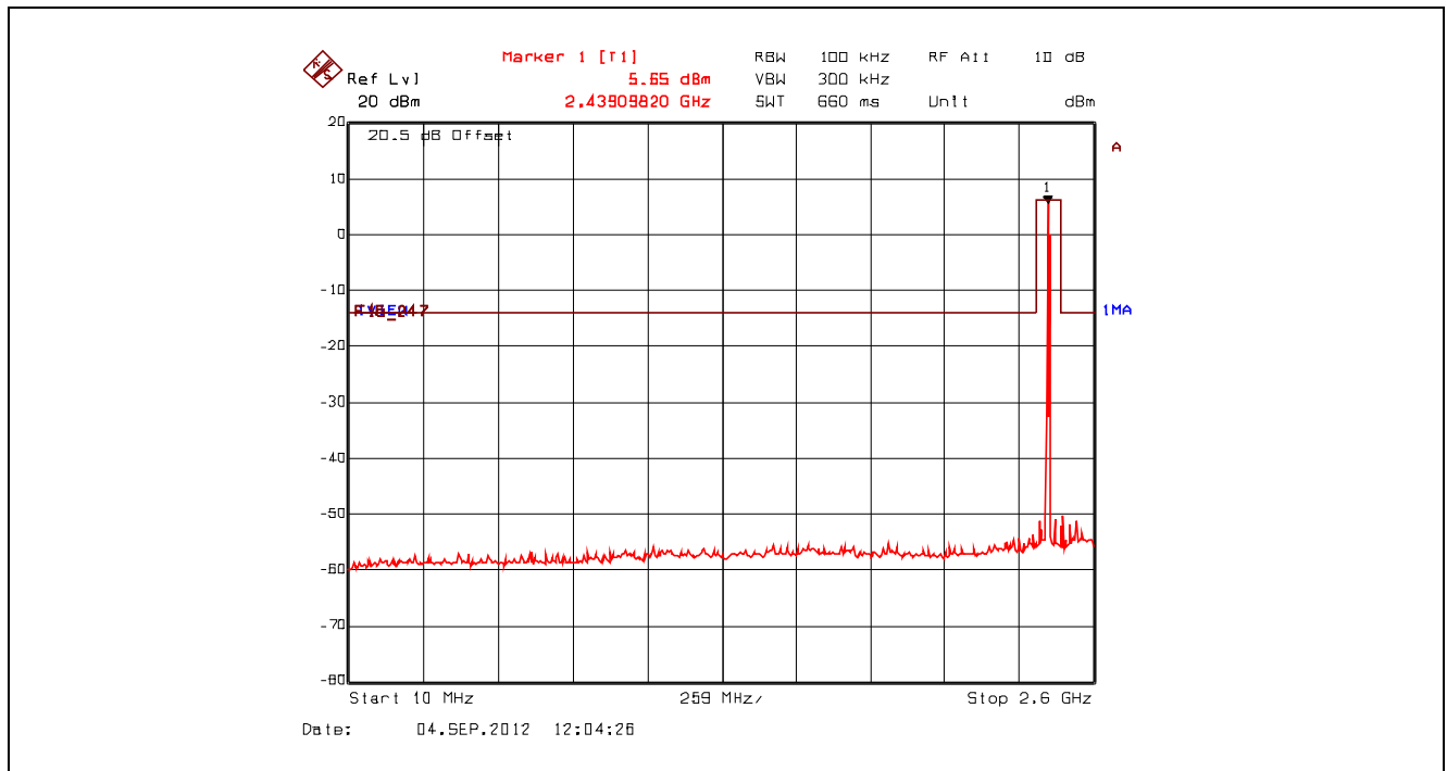
Plot 5.5.4.2.3. Spurious RF Conducted Emissions, 2438 MHz, 16-QAM, 10 MHz – 2.6 GHz
