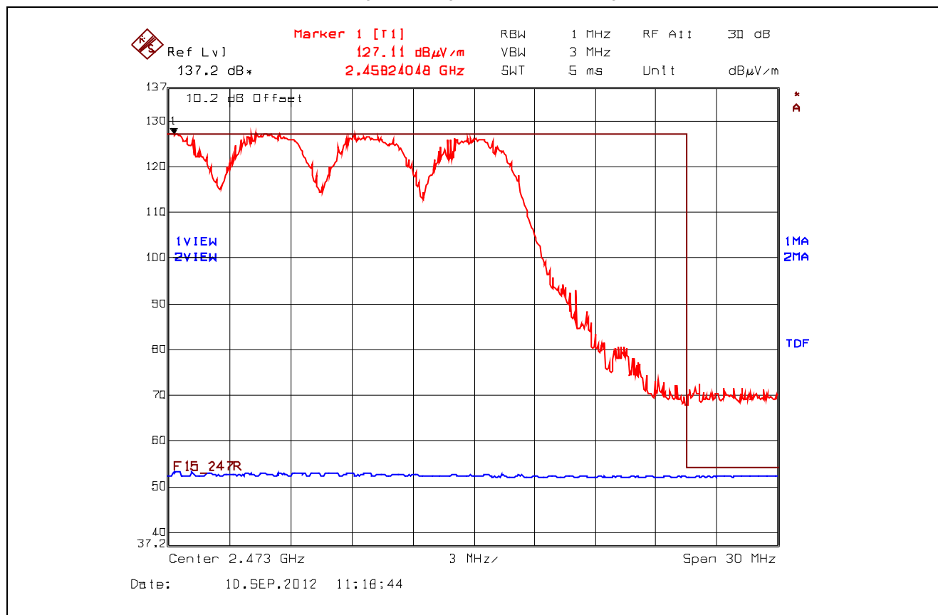
Plot 5.6.4.2.2.12. Band-Edge RF Radiated Emissions at 3 m, Vertical Polarization Upper Band-edge, Hopping Mode, Power Setting 8, 16-QAM
