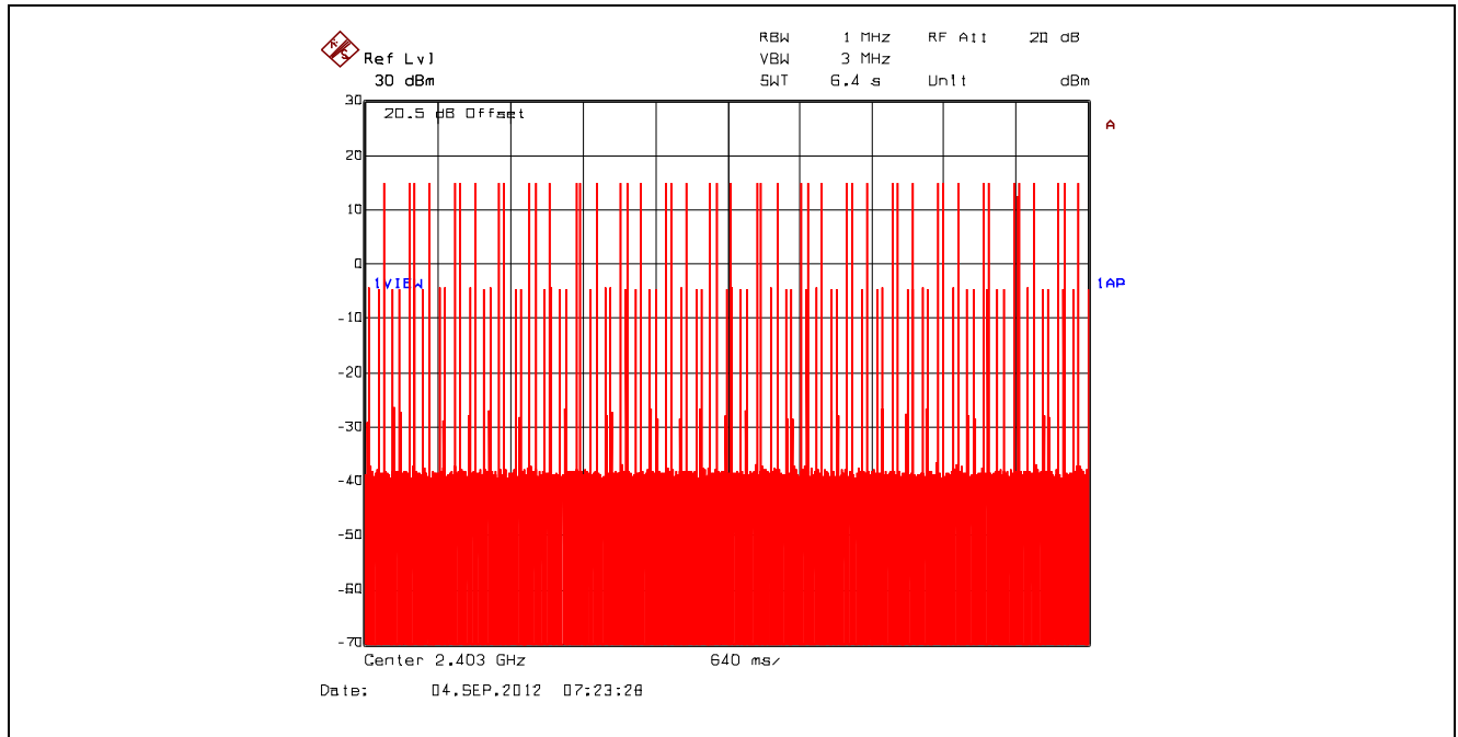
Plot 5.3.4.17. Time of Occupancy, 2403 MHz, 16-QAM, Dwell Time @ 2403 MHz = 190.380762 \mu s
