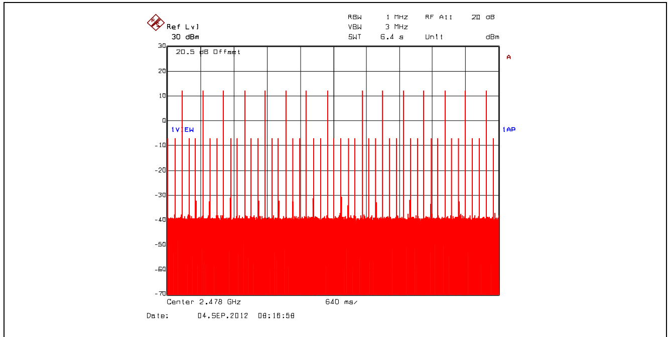
Plot 5.3.4.27. Time of Occupancy, 2478 MHz, BPSK, Dwell Time @ 2478 MHz = 230.460922 \mu s
