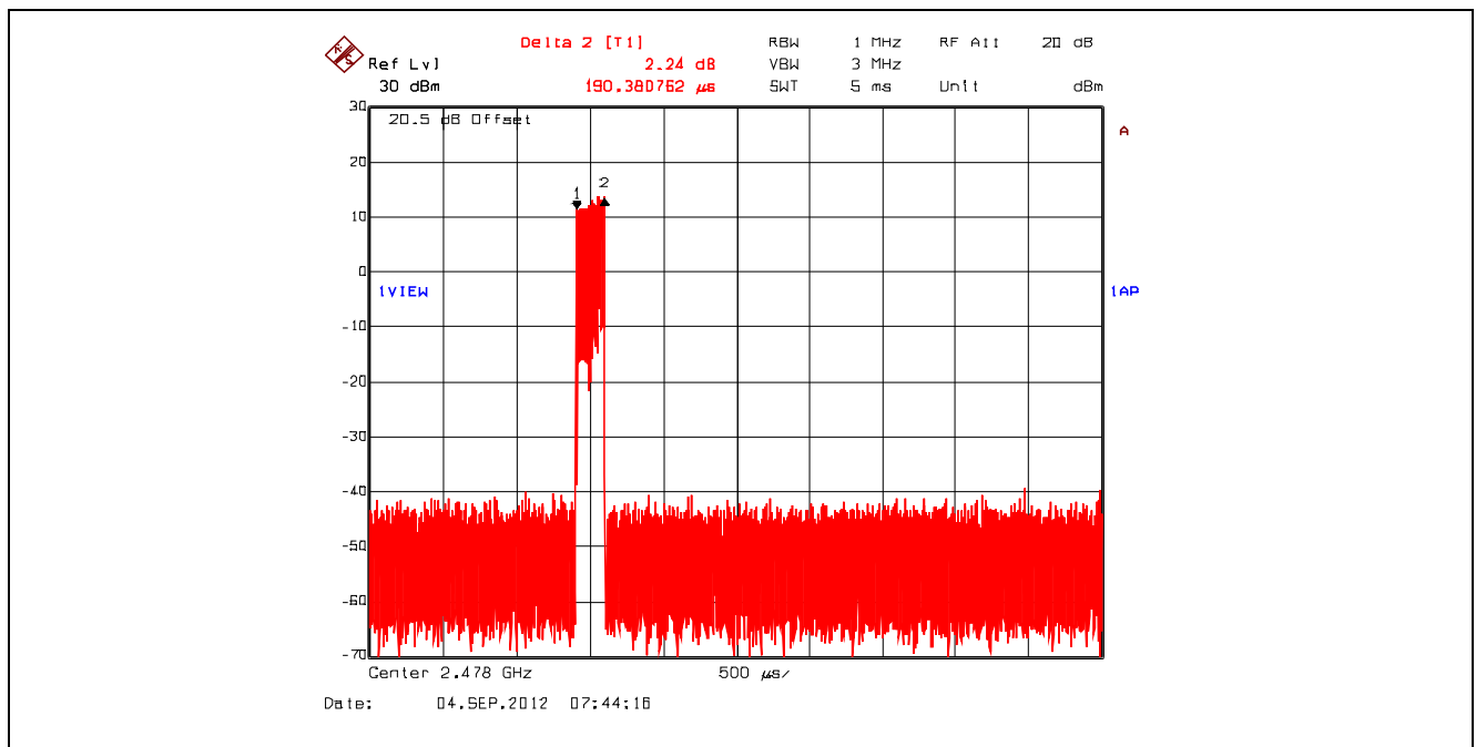
Plot 5.3.4.21. Time of Occupancy, 2478 MHz, 16-QAM, Dwell Time @ 2478 MHz = 190.380762 \mu s
