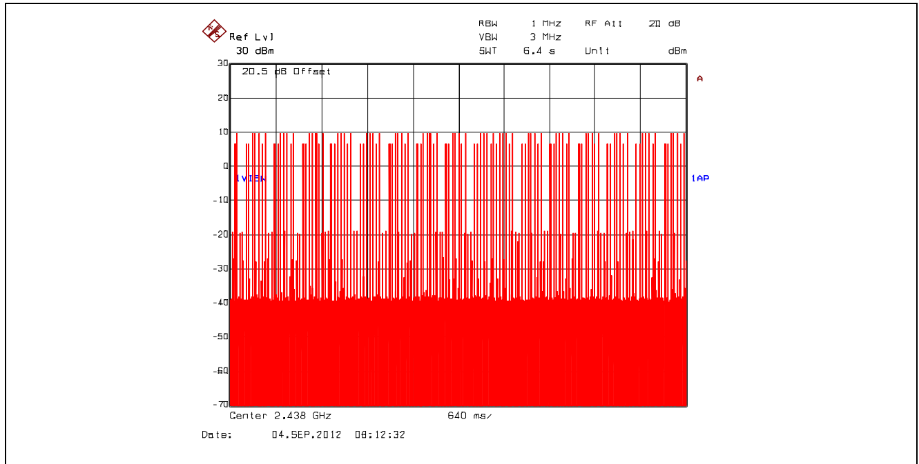
Plot 5.3.4.25. Time of Occupancy, 2438 MHz, BPSK, Dwell Time @ 2438 MHz = 230.460922 \mu s
