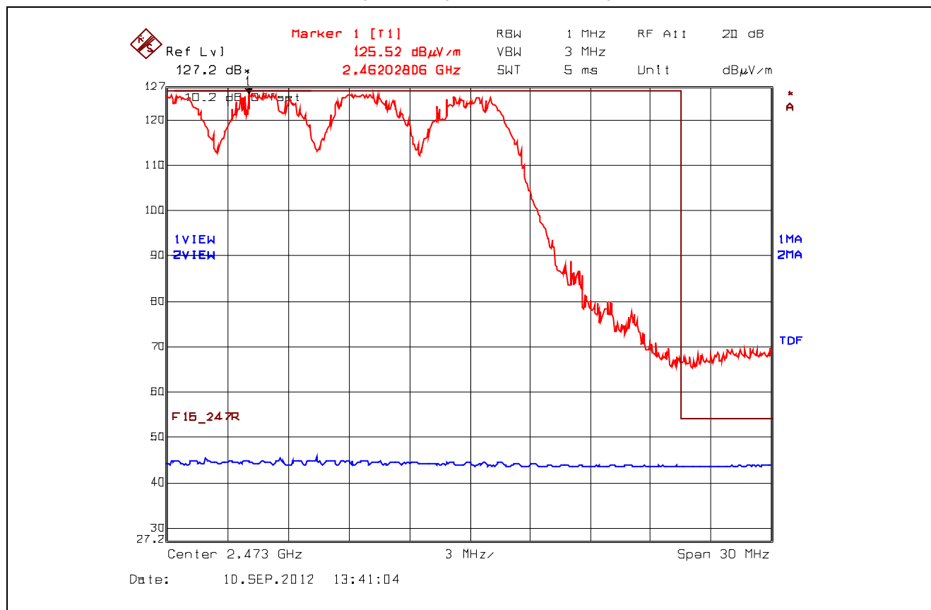
Plot 5.6.4.2.2.11. Band-Edge RF Radiated Emissions at 3 m, Horizontal Polarization Upper Band-edge, Hopping Mode, Power Setting 8, 16-QAM
