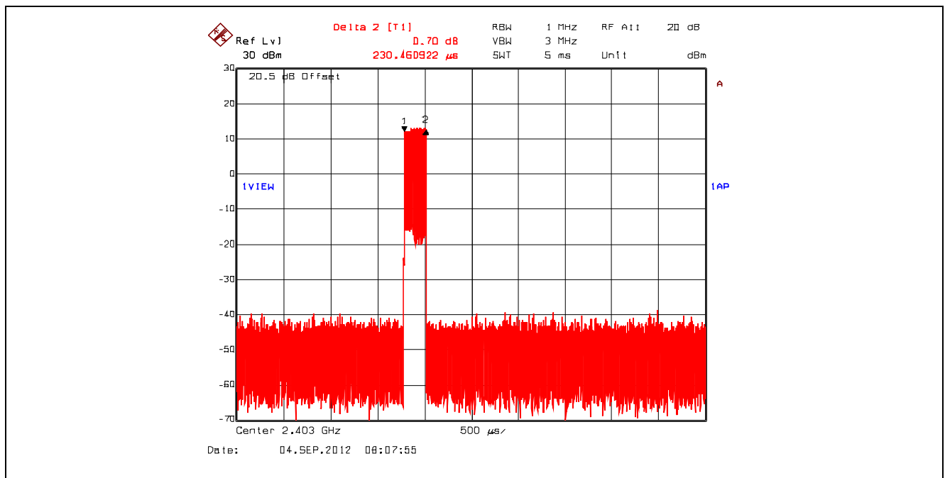
Plot 5.3.4.23. Time of Occupancy, 2403 MHz, BPSK, Dwell Time @ 2403 MHz = 230.460922 \mu s
