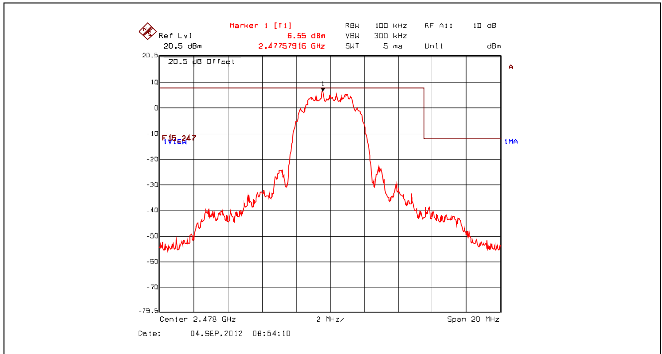
Plot 5.5.4.1.3. Band-Edge RF Conducted Emissions, Upper Band-edge, Single Frequency Mode, 16-QAM
