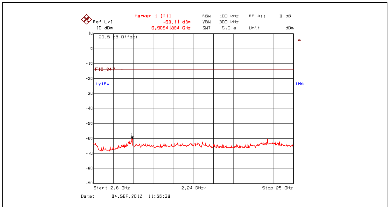
Plot 5.5.4.2.4. Spurious RF Conducted Emissions, 2438 MHz, 16-QAM, 2.6 GHz - 25 GHz
