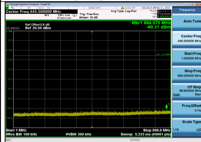
916MHz, Plot 2, 1MHz~890MHz
