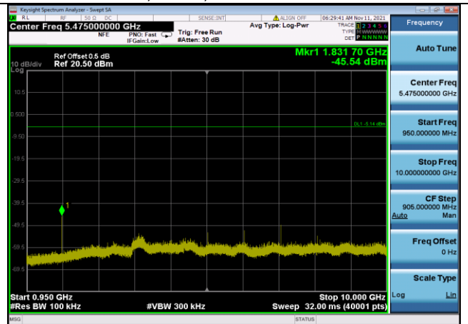
916MHz, Plot 3, 950MHz~10000MHz
