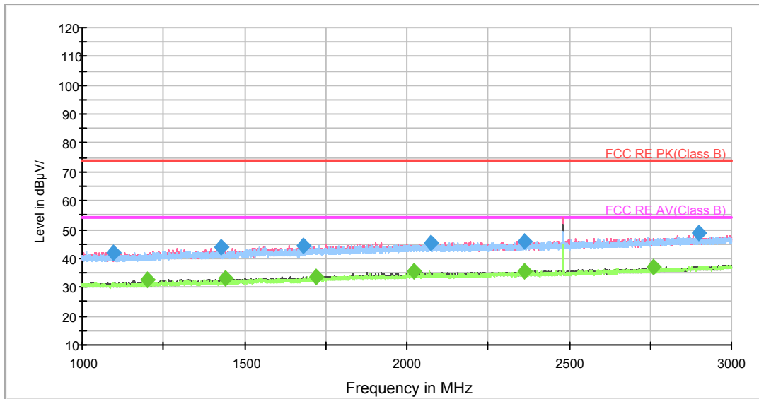
Radiates Emission from 1GHz to 3GHz
