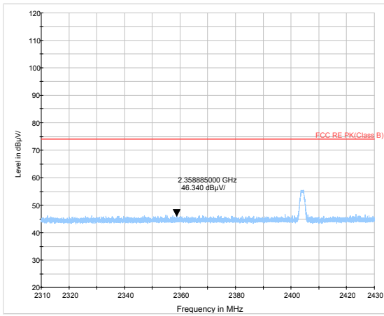
BLE Channel 0 Peak
