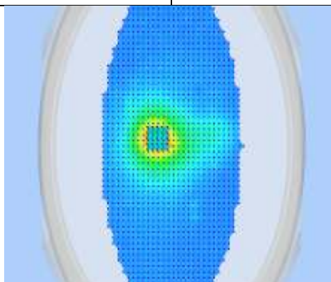
3D View Plot
