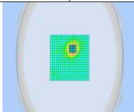
3D View Plot
