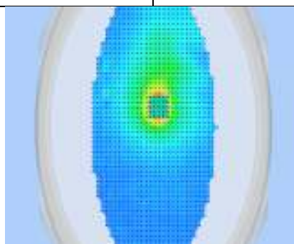
3D View Plot
