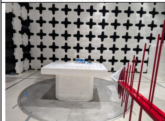
Radiated Emission (30MHz-1GH) Front View
