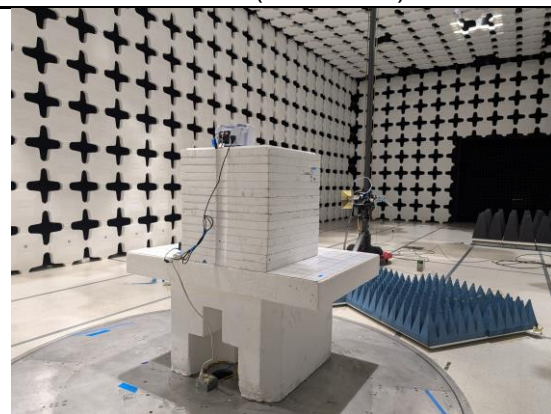
Radiated Emission Above 1GHz Back View
