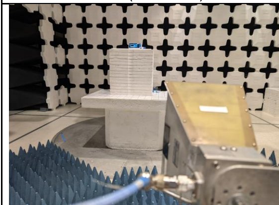
Radiated Emission Above 1GHz Front View
