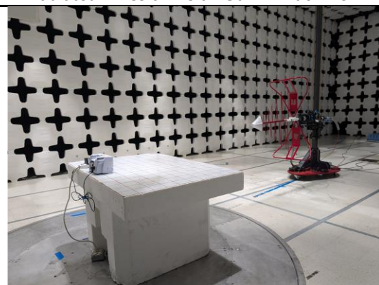
Radiated Emission (30MHz-1GH) Back View
