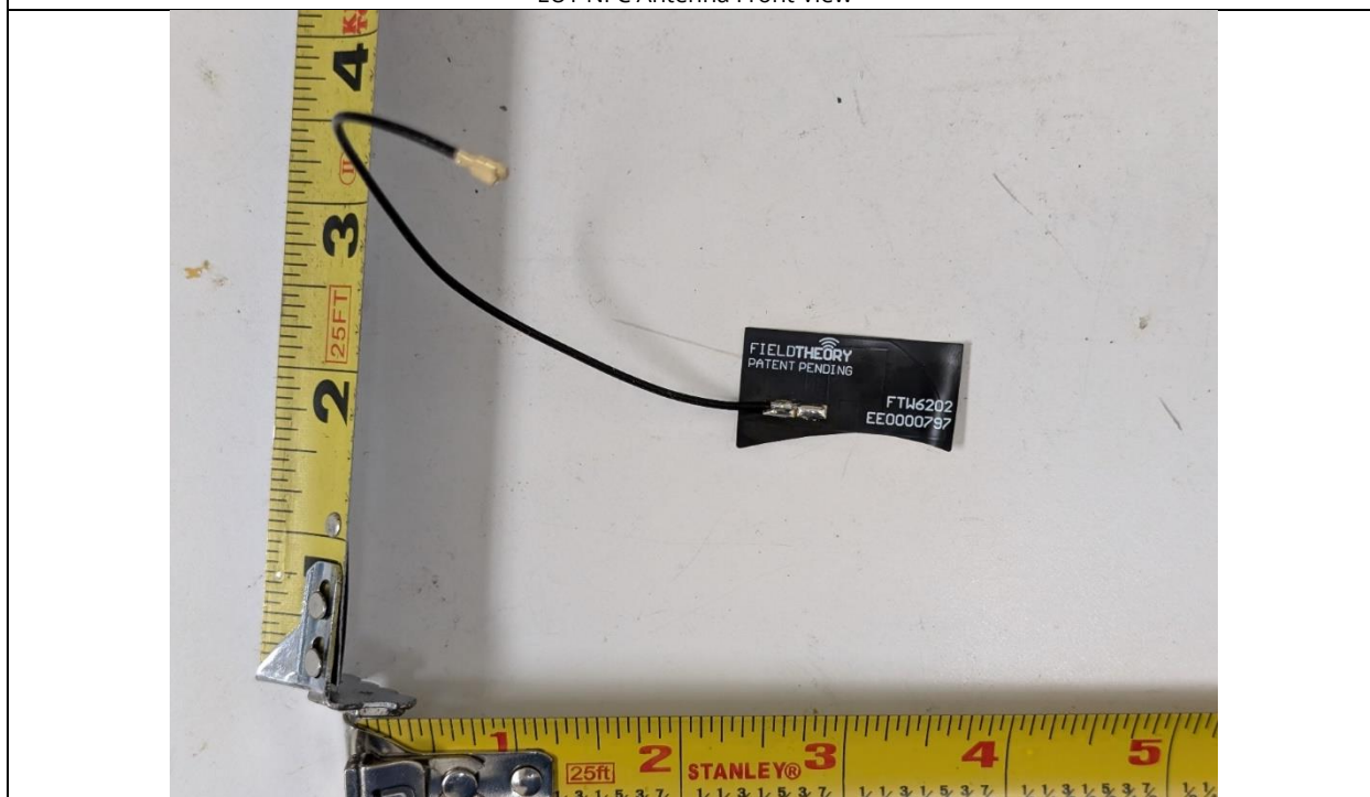
EUT WLAN Antenna Back View
