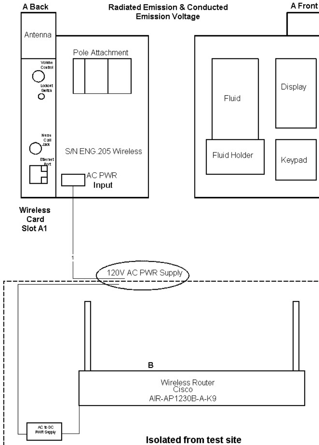
Figure 1. Block Diagram of Test Configuration (FCC 15.207 & FCC 15.209)
