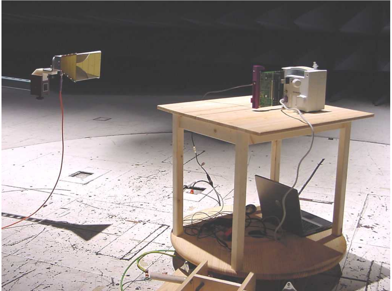
Photograph 6. Restricted Bandedge Test Setup
