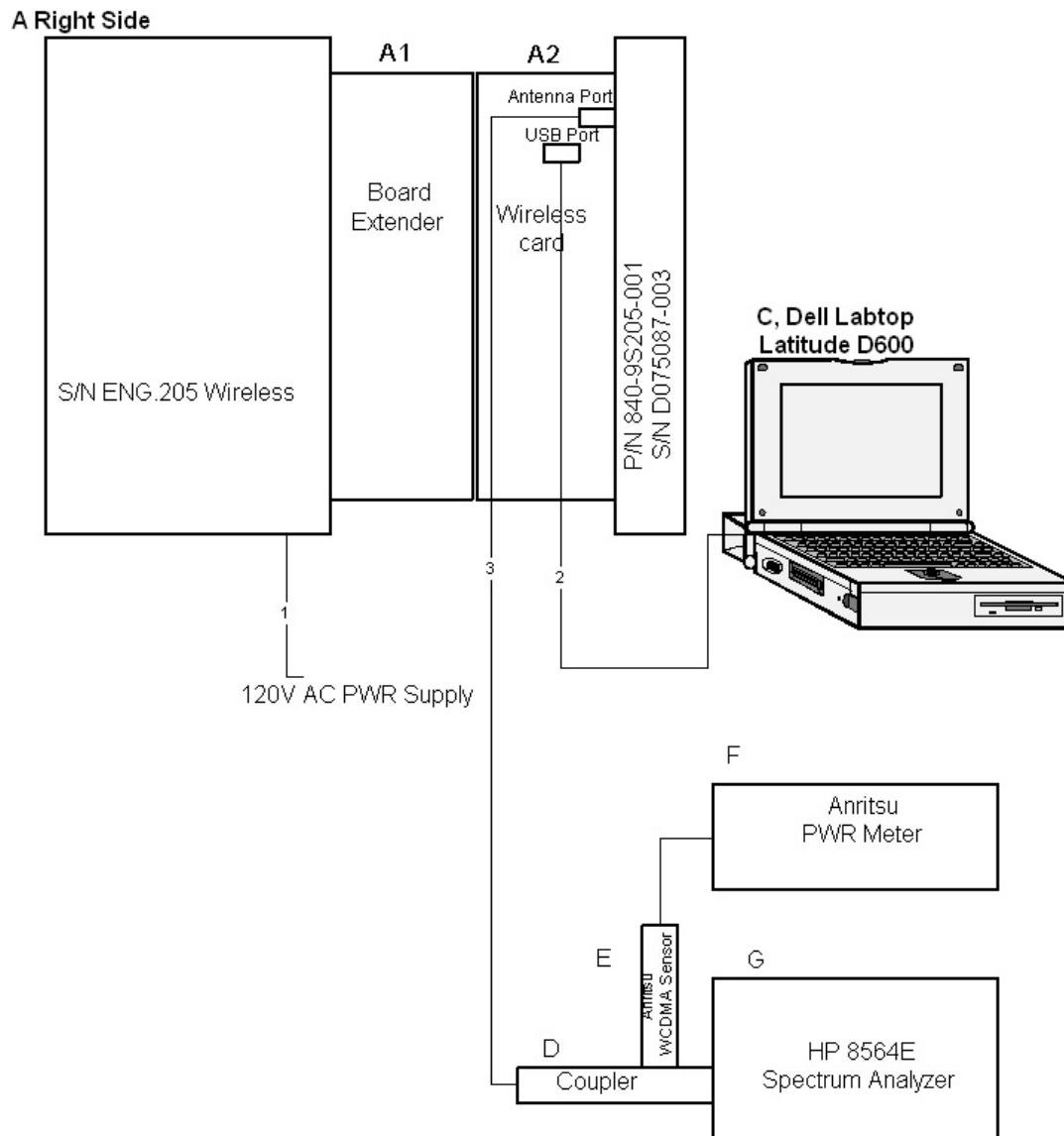
Figure 2. Block Diagram of Test Configuration (FCC 15.247)
