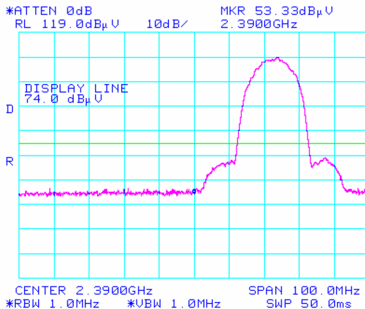
PEAK Limit at Vertical polarization, Lower Edge for 2412 MHz Plot
