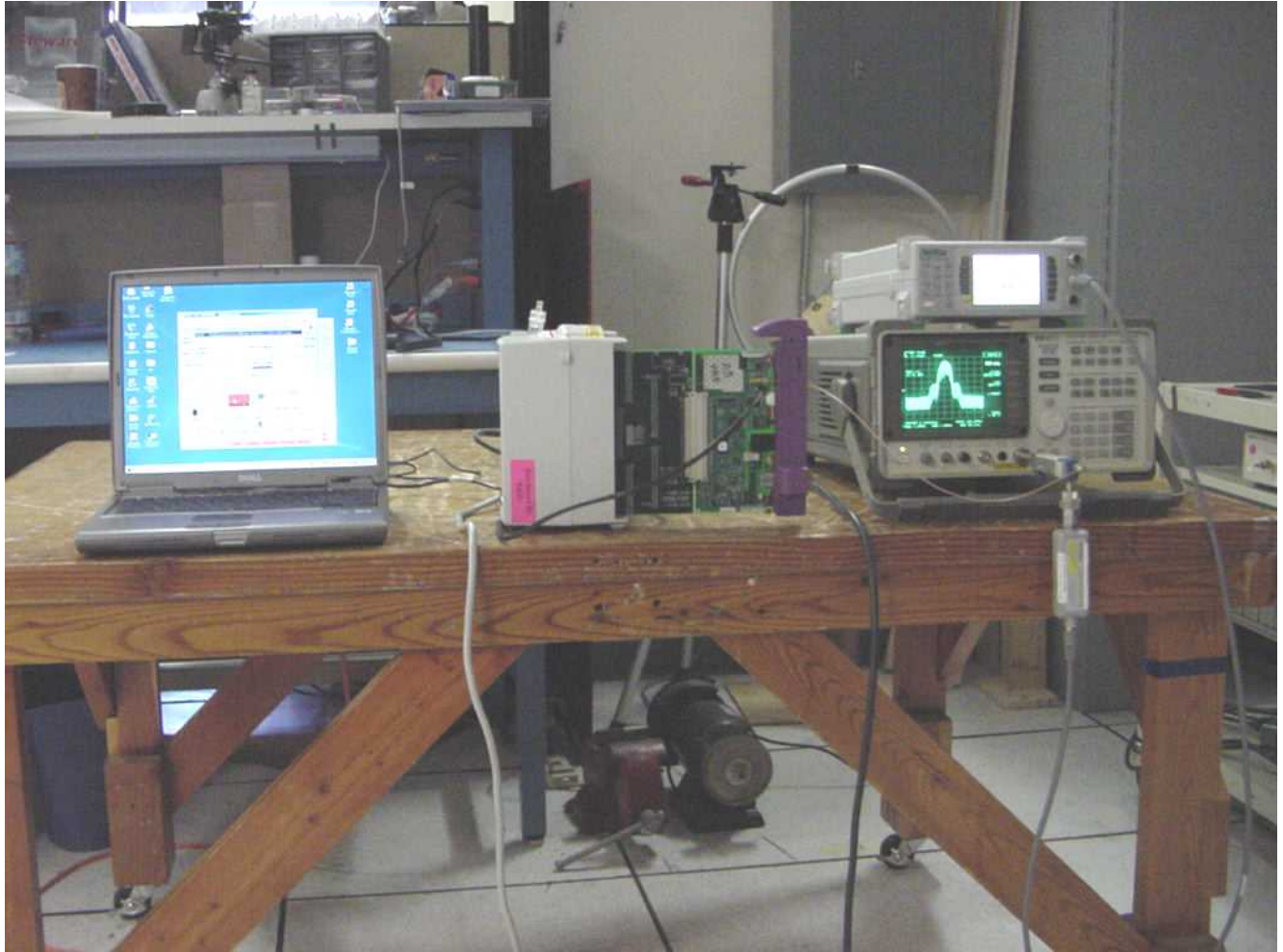
Photograph 7. Peak Power Spectral Density Test Setup
