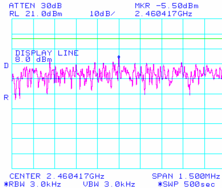
Peak Power Spectral Density for 2462 MHz (High channel)
