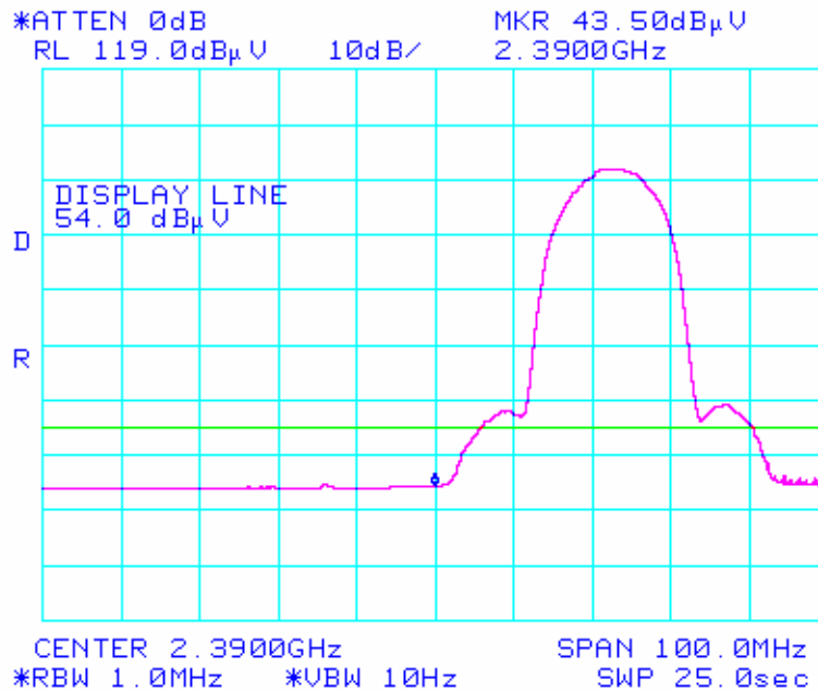
AVERAGE Limit at Vertical polarization, Lower Edge for 2412 MHz Plot
