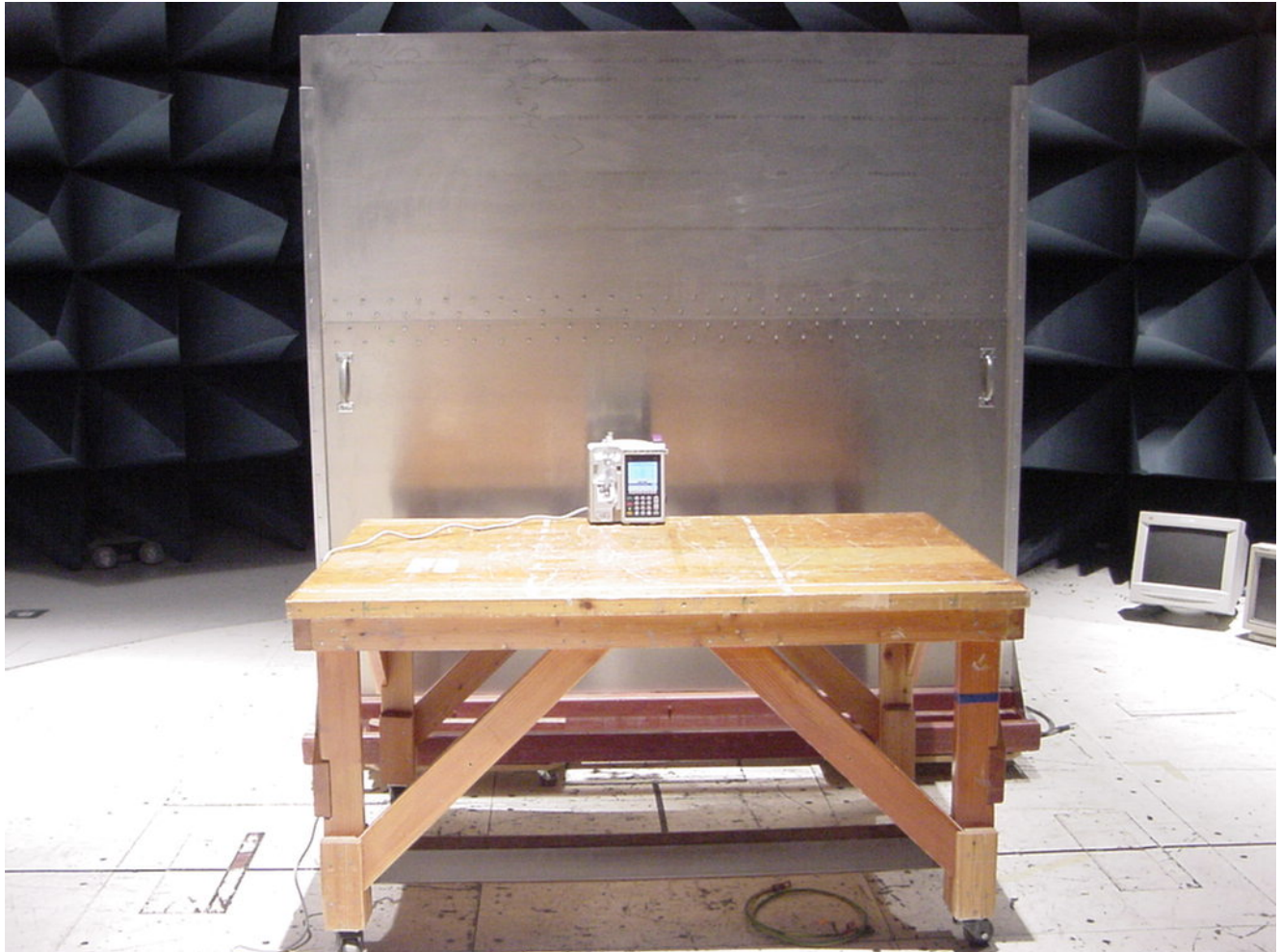
Photograph 1. Conducted Emissions Limits, Test Setup
