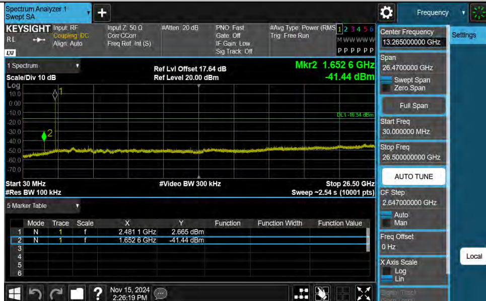
DH5-Ant1-2480-30~26500-PASS
