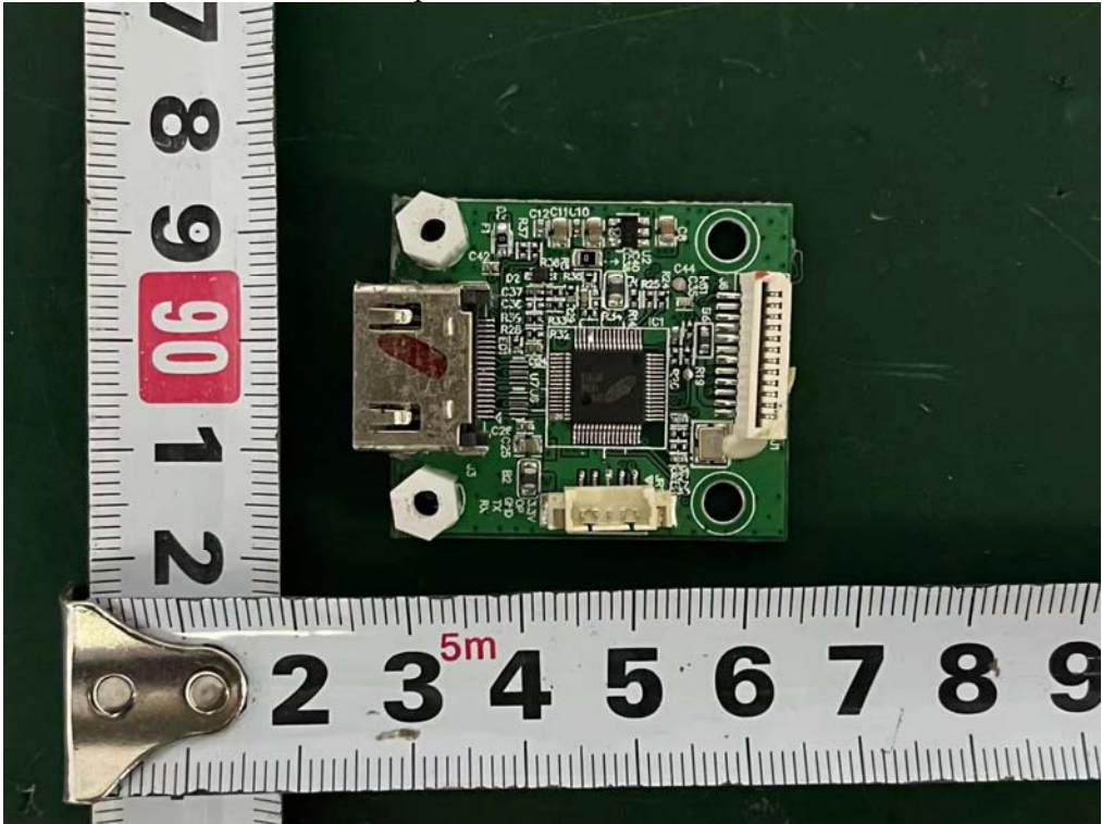
Internal Photos M/N: Klipsch Cinema One Sound Bar
