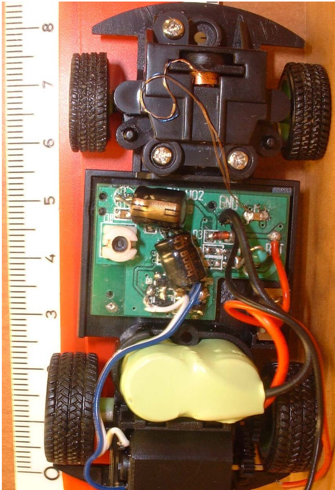
15.Figure 11 Receiver Circuit Board View 1
