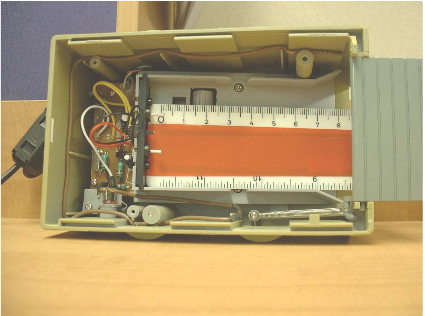
12.4. Figure 8 Transmitter Circuit Board View 1
