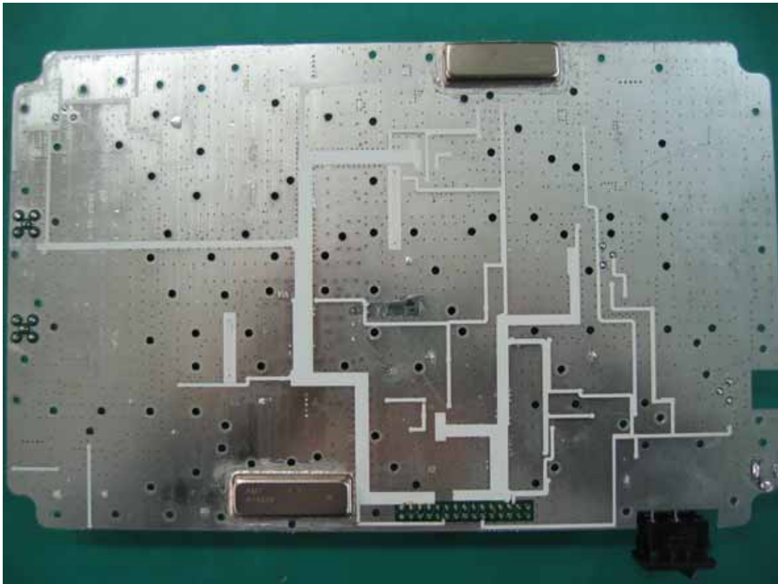
RF PCB 3
