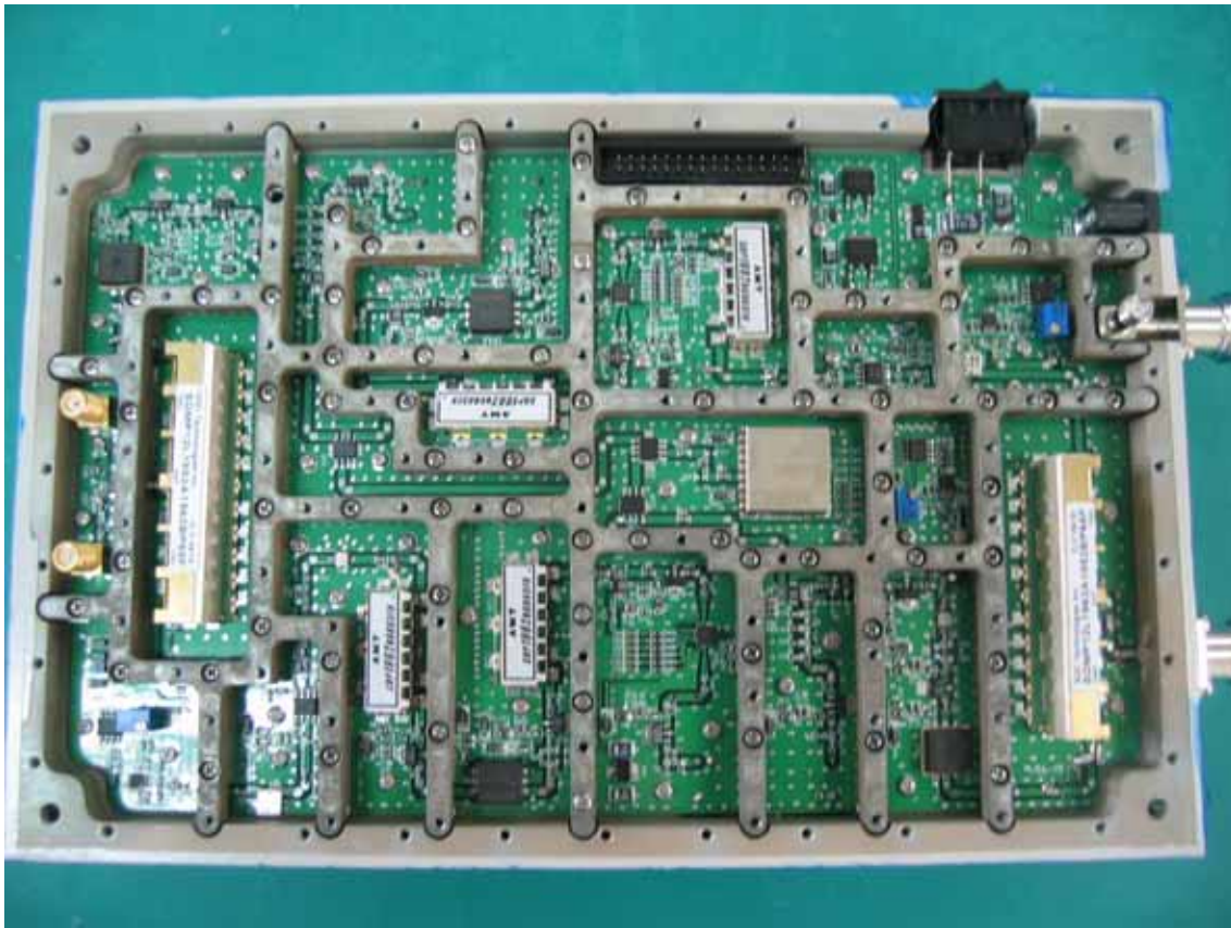
RF PCB 1
