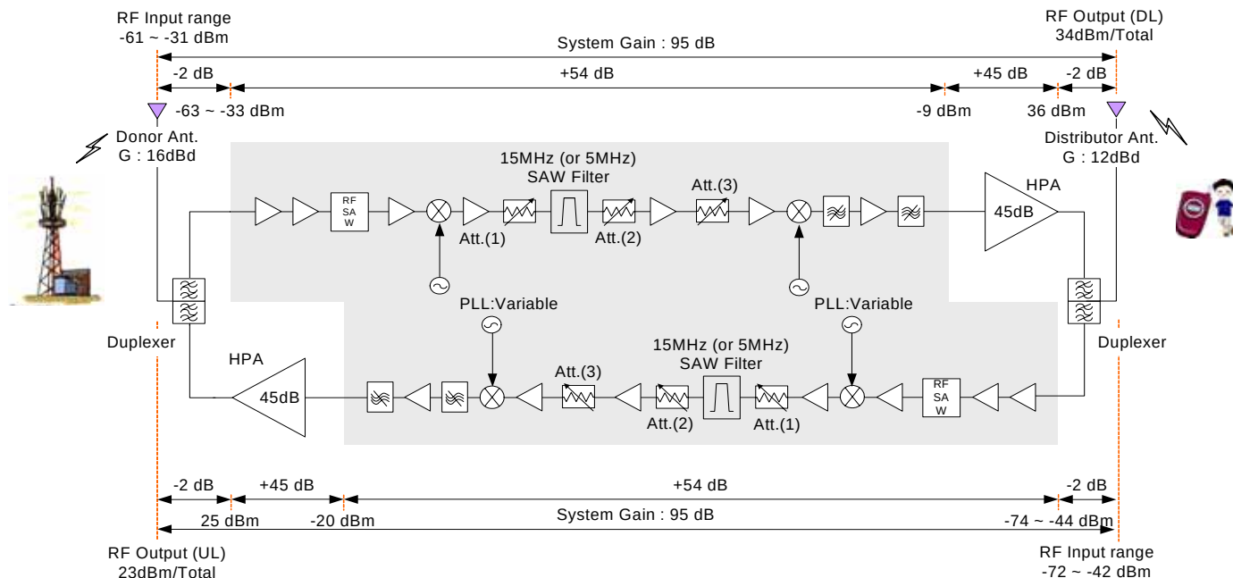
Figure 4.1 shows the block diagram of a band specific repeater.
