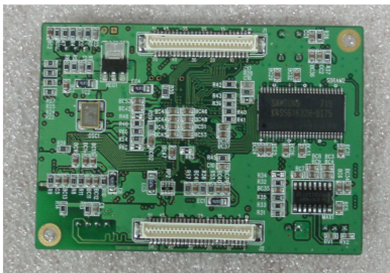
<CPU B'D Bottom View>
