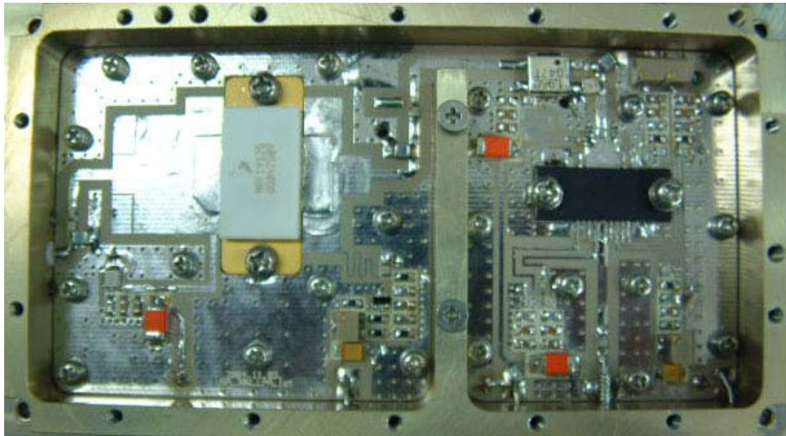
Drive AMP
