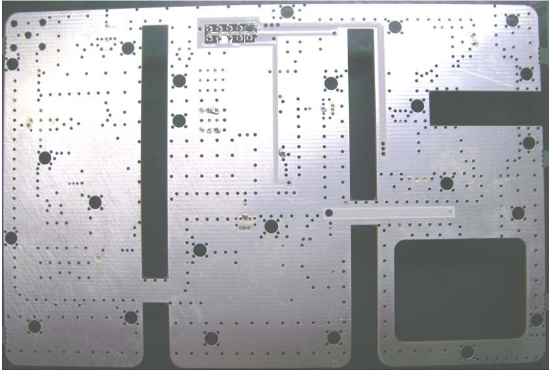
<HPA PCB Bottom View>
