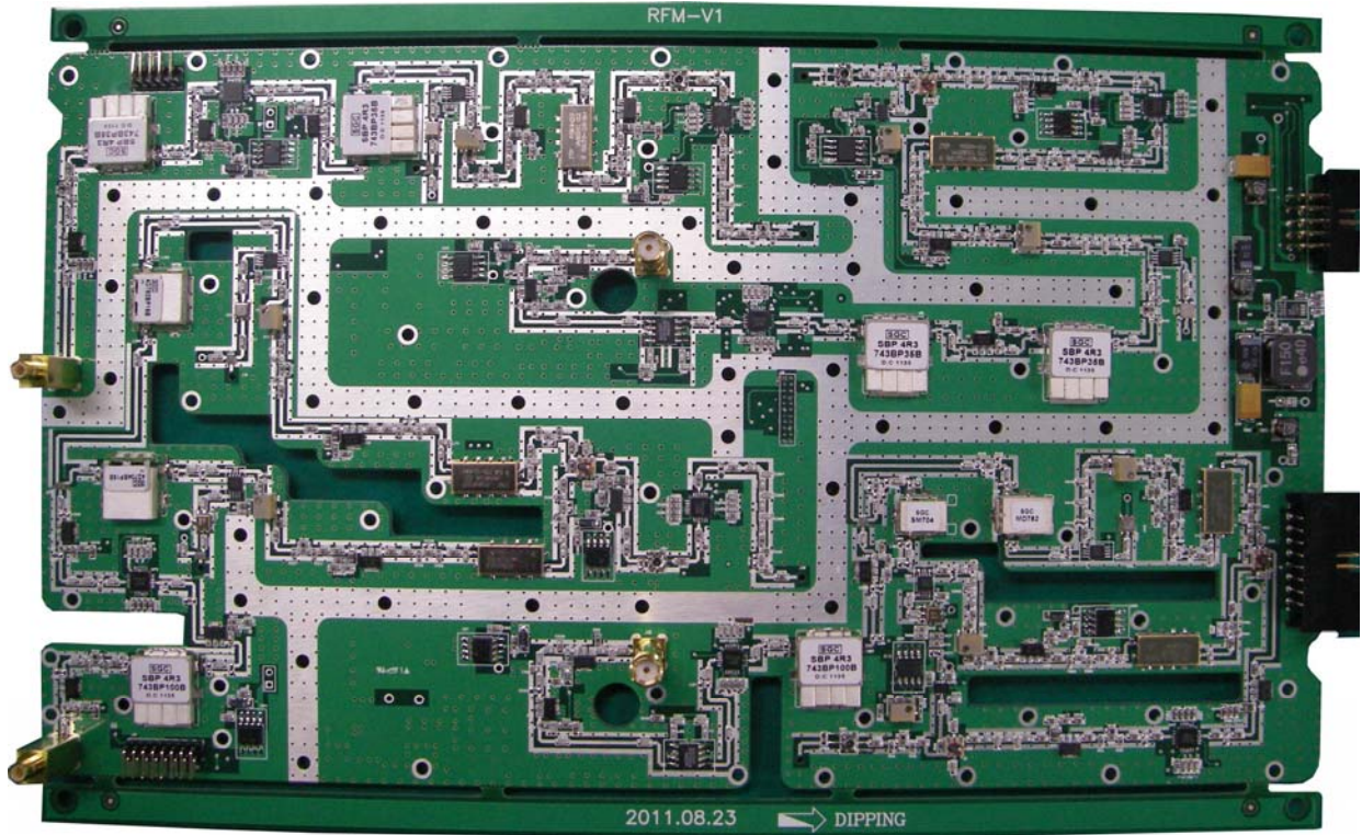
<TOP PCB Top View>
