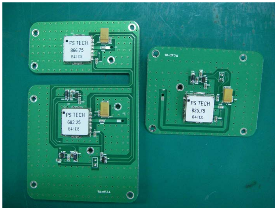
<BOTTOM PCB Top View>
