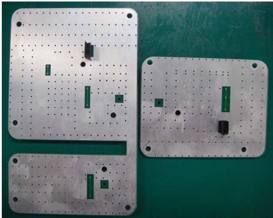
<BOTTOM PCB Bottom View>
