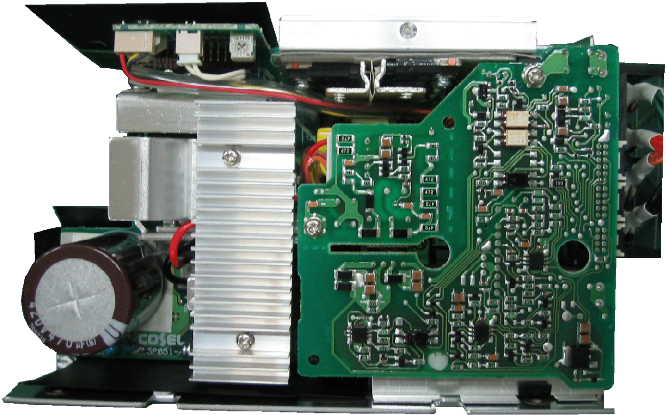
<PSU Top View>
