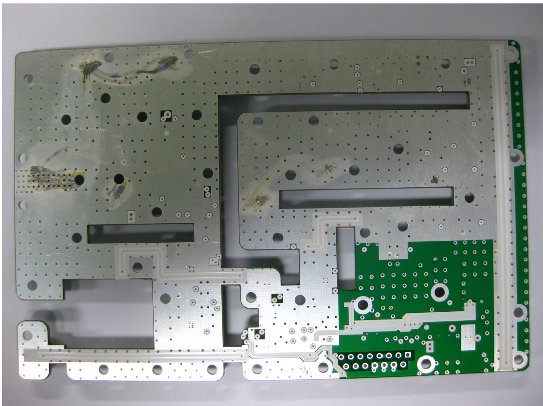
<HPA PCB Bottom View>
