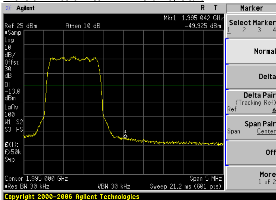
PLOTS OF EMISSION PCS BAND EDGE(1275) G band
