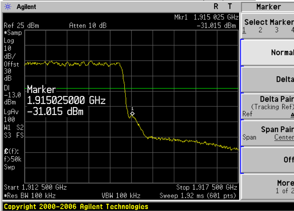
PLOTS OF EMISSION PCS FOR LTE BAND EDGE(1250) _G band
