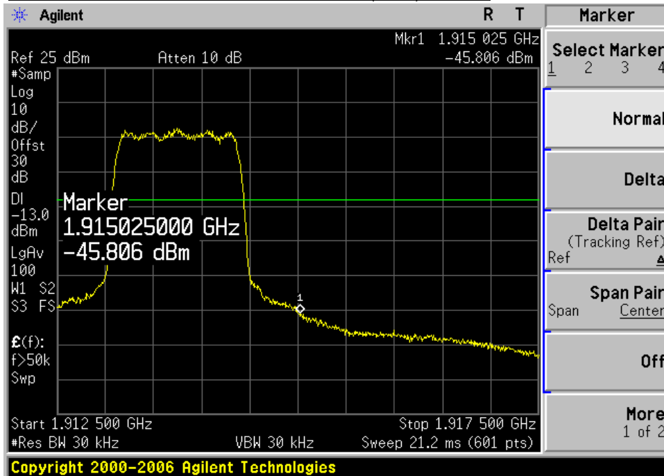
PLOTS OF EMISSION PCS BAND EDGE(1275) G band
