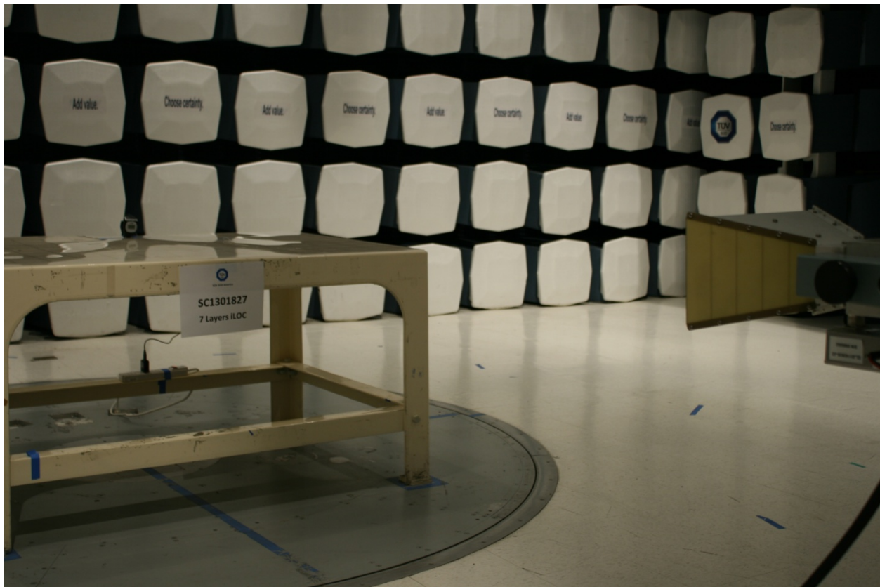
Test Setup Photo BT part15.249 Spurious Emission (Above 1GHz Front)
