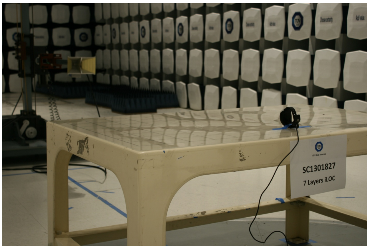
Test Setup Photo BT part15.249 20dB BW, 99% Emission BW and Fundamental (Above 1GHz Back)
