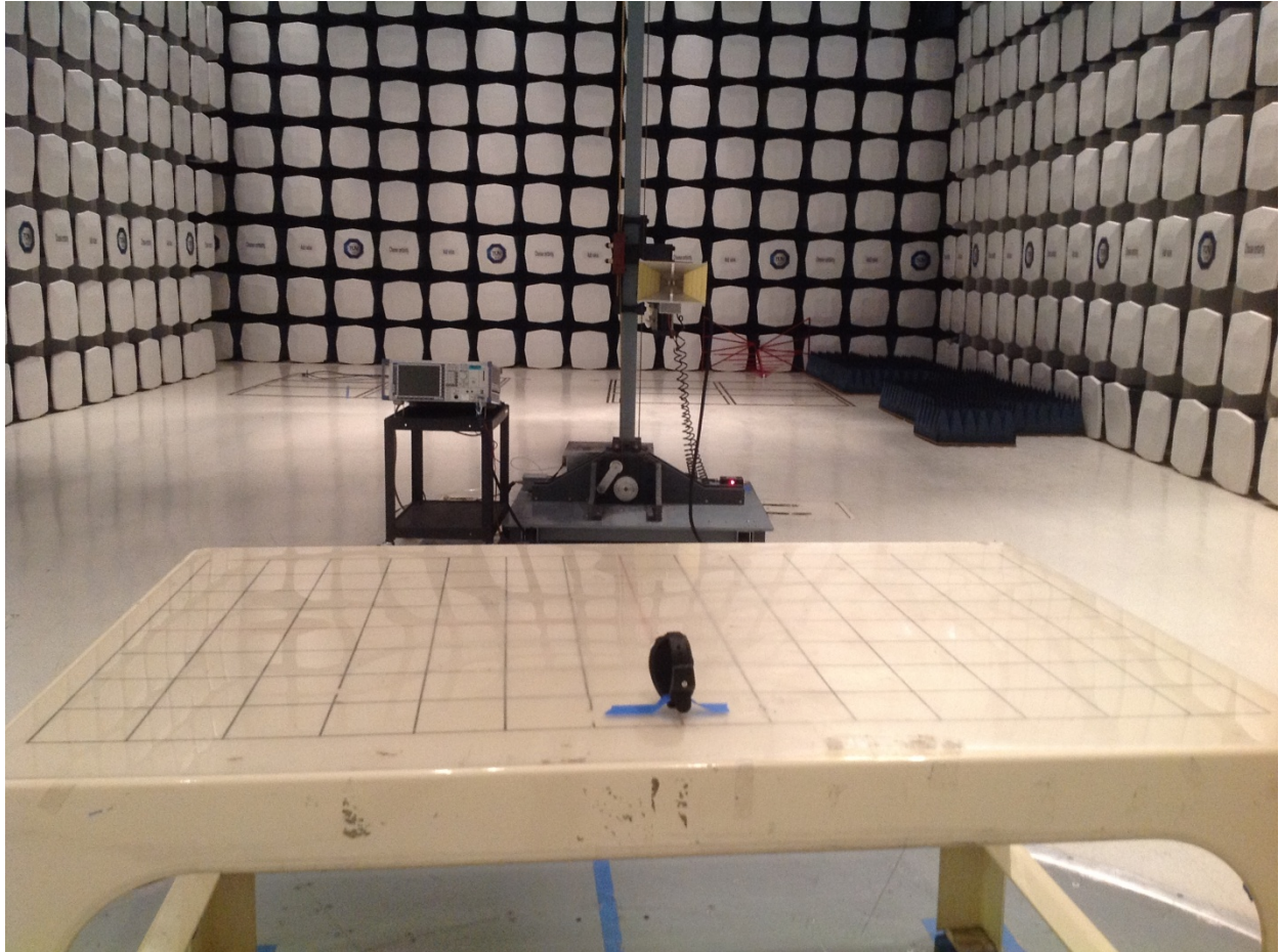
Test Setup Photo (back)
