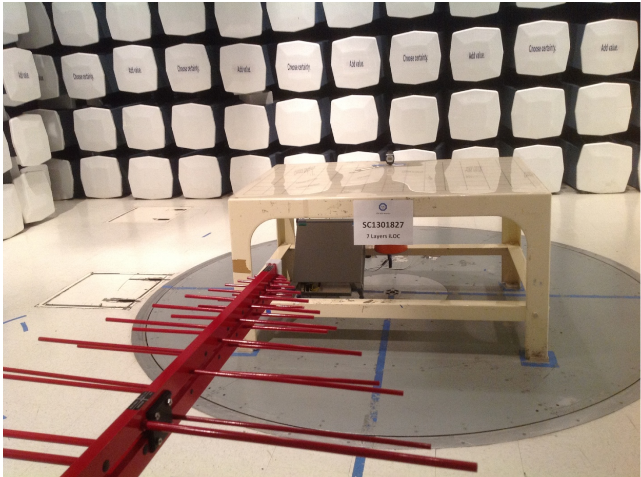
Test Setup Photo (Front)
