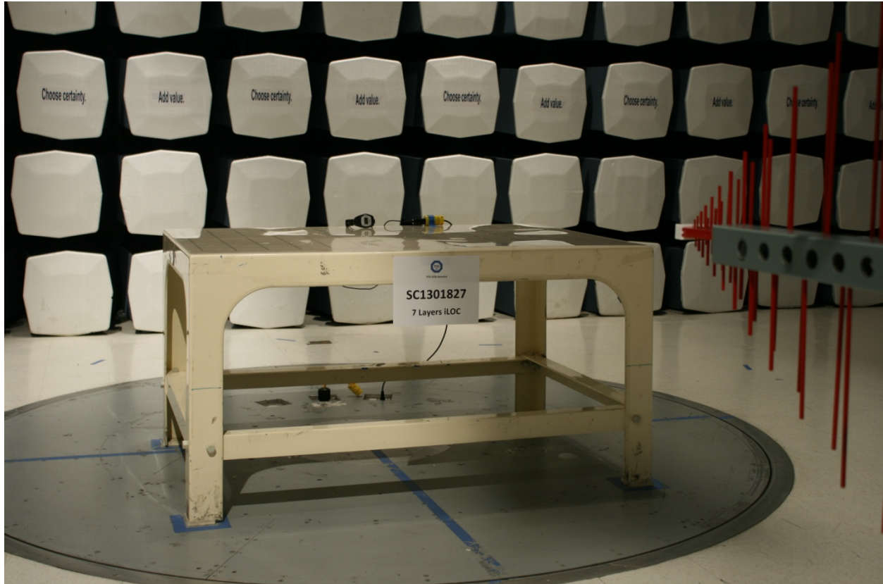
Test Setup Photo BT part15.249 Spurious Emission (Below 1GHz Front)
