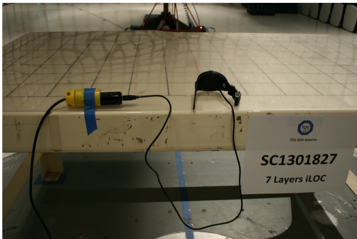
Test Setup Photo BT part15.249 Spurious Emission (Below 1GHz Back)
