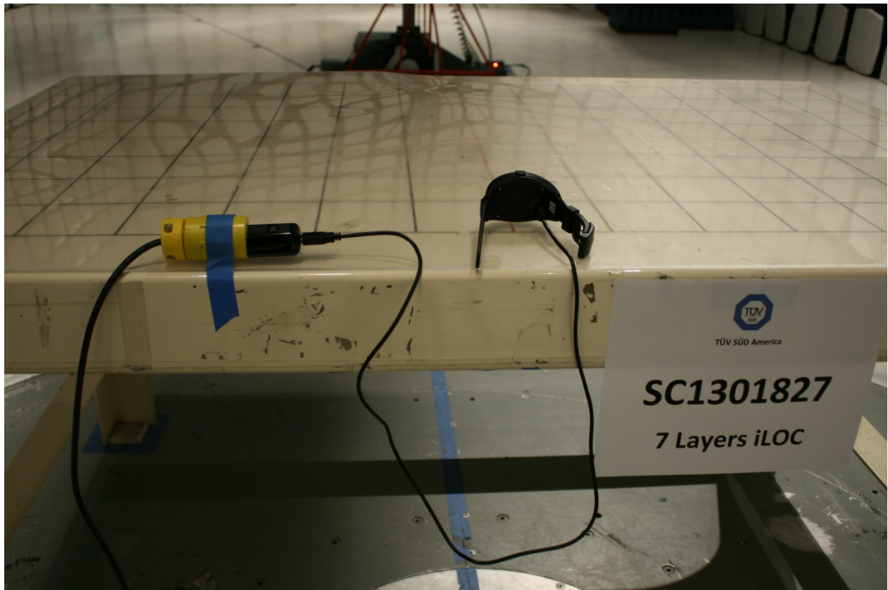
Test Setup Photo (Below 1GHz Back)
