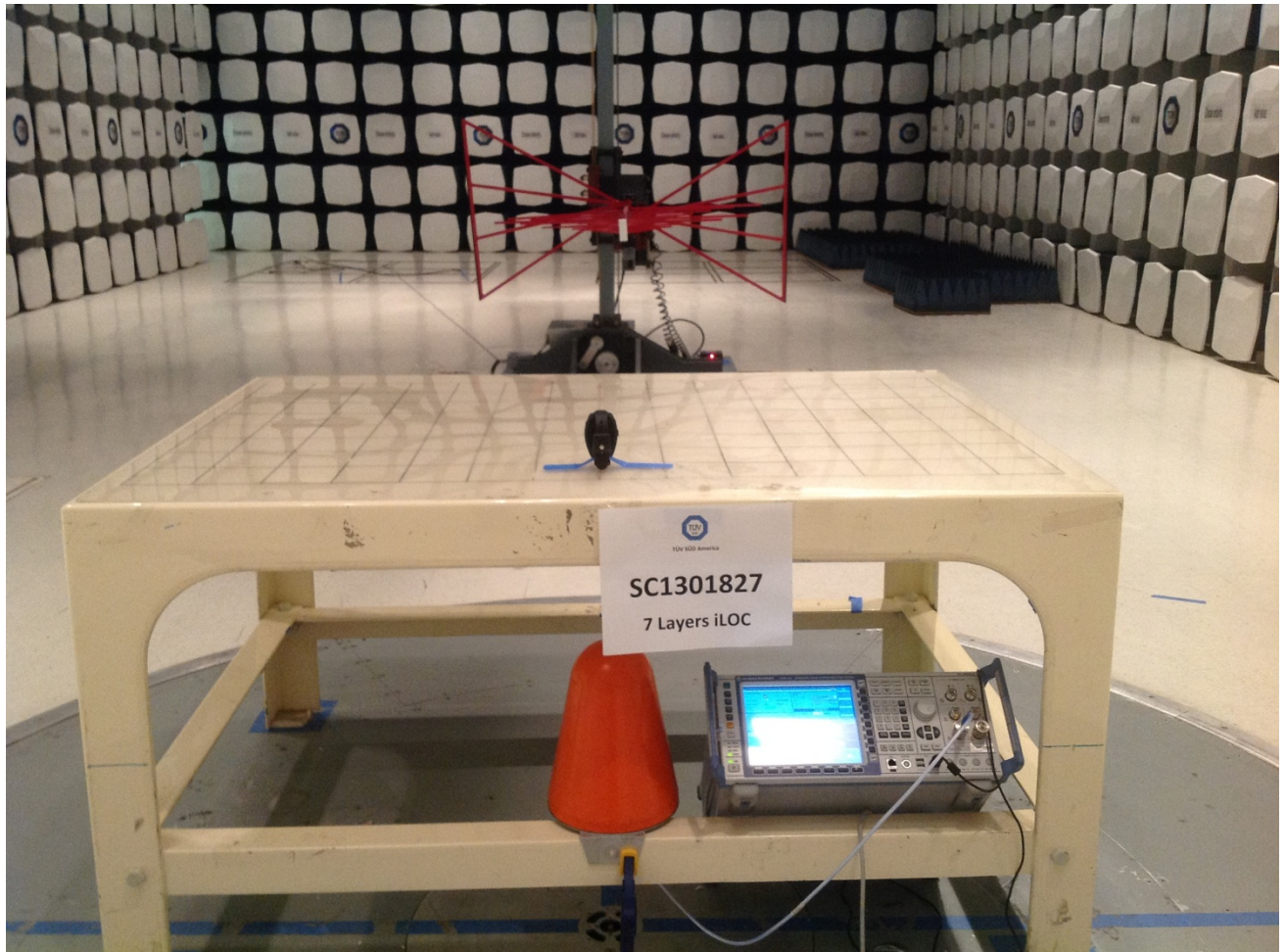
Test Setup Photo (Back)
