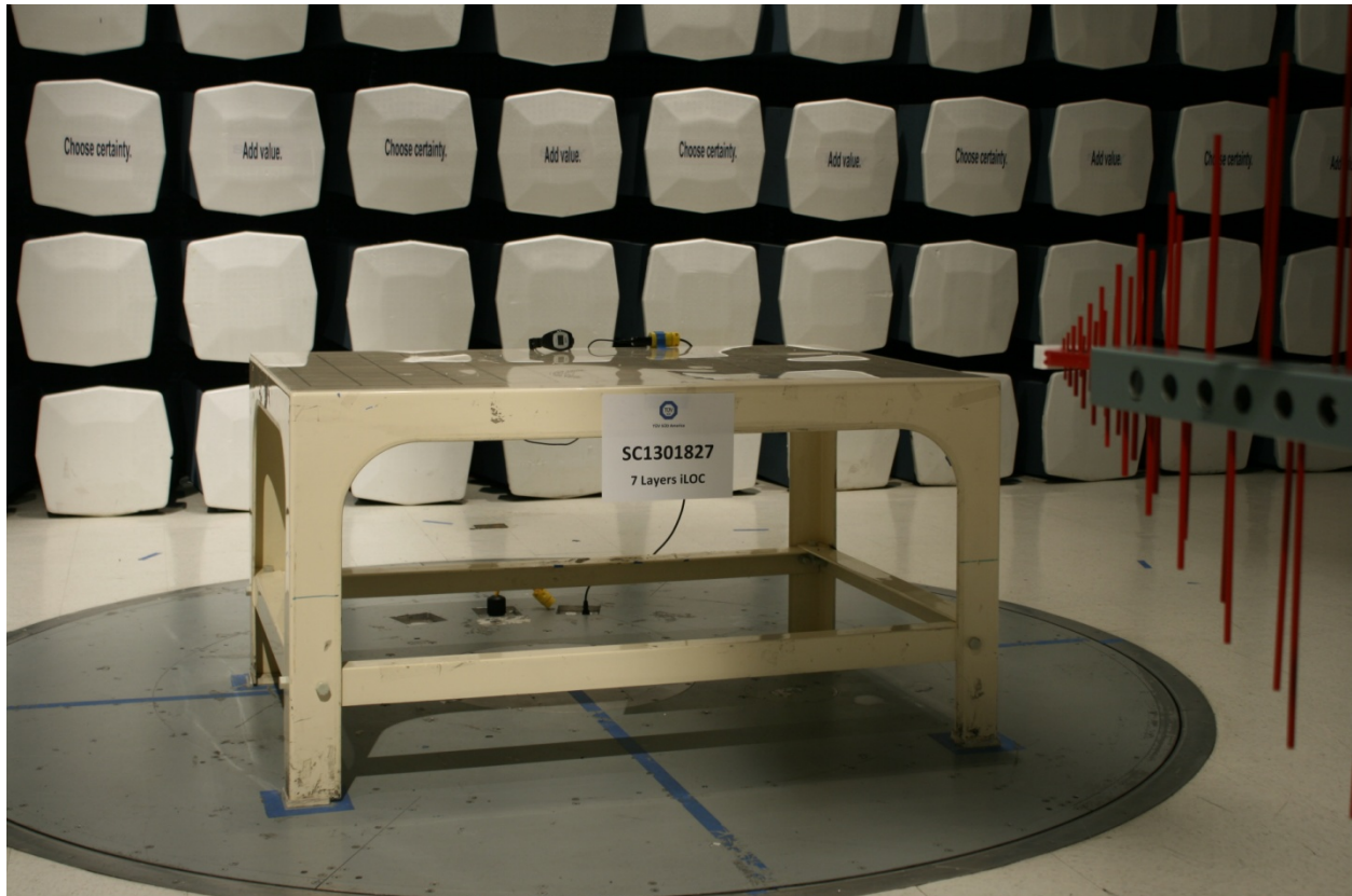
Test Setup Photo (Below 1GHz Front)
