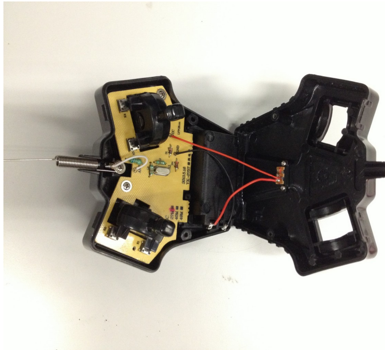
Internal view
