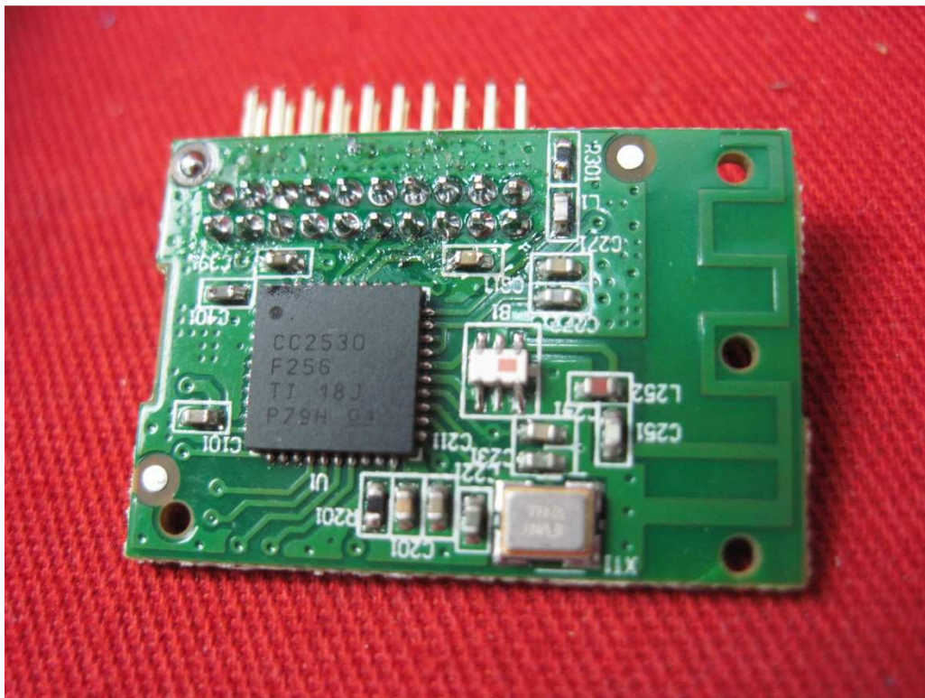
Detail of wireless module-2
