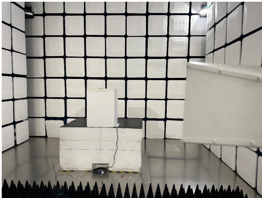
Above 1GHz-RFID
