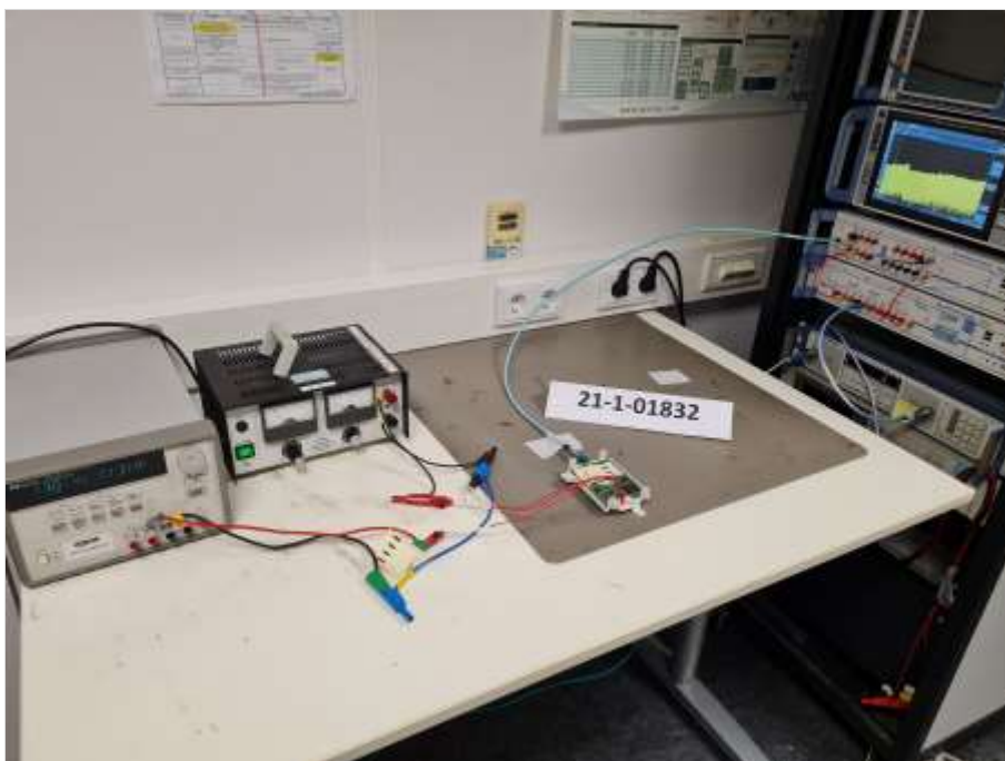
Photograph 10: EUT setup conducted measurement, overview
