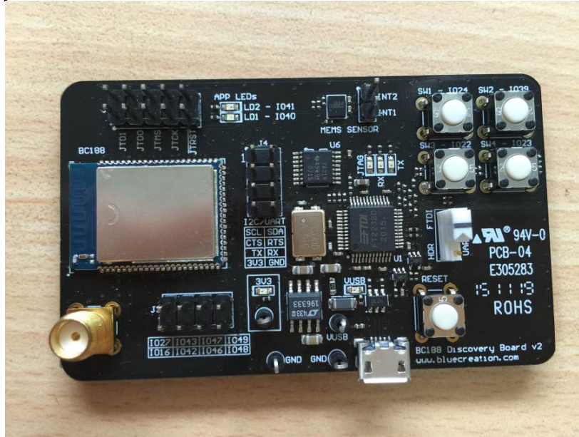
Photograph 1: EUT with test board
