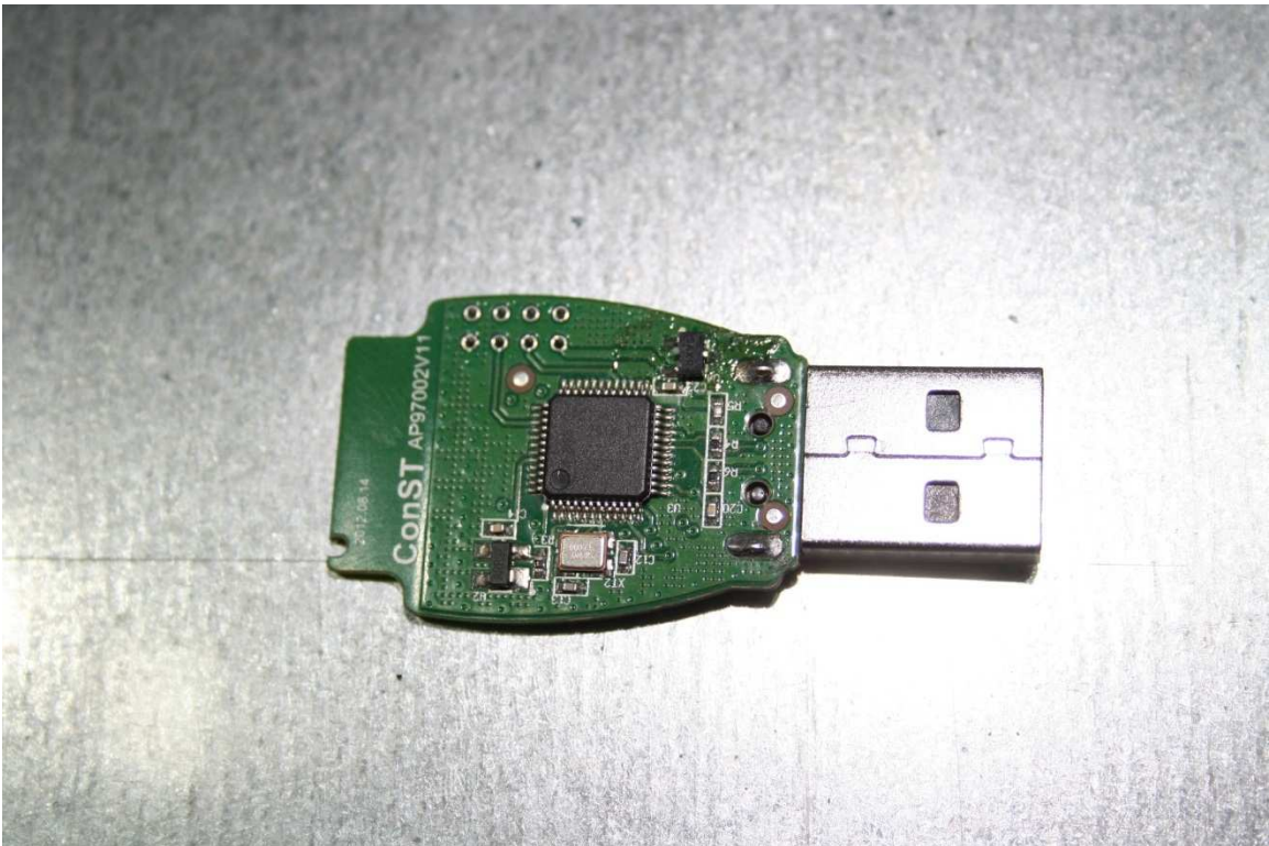
PCB rear side
