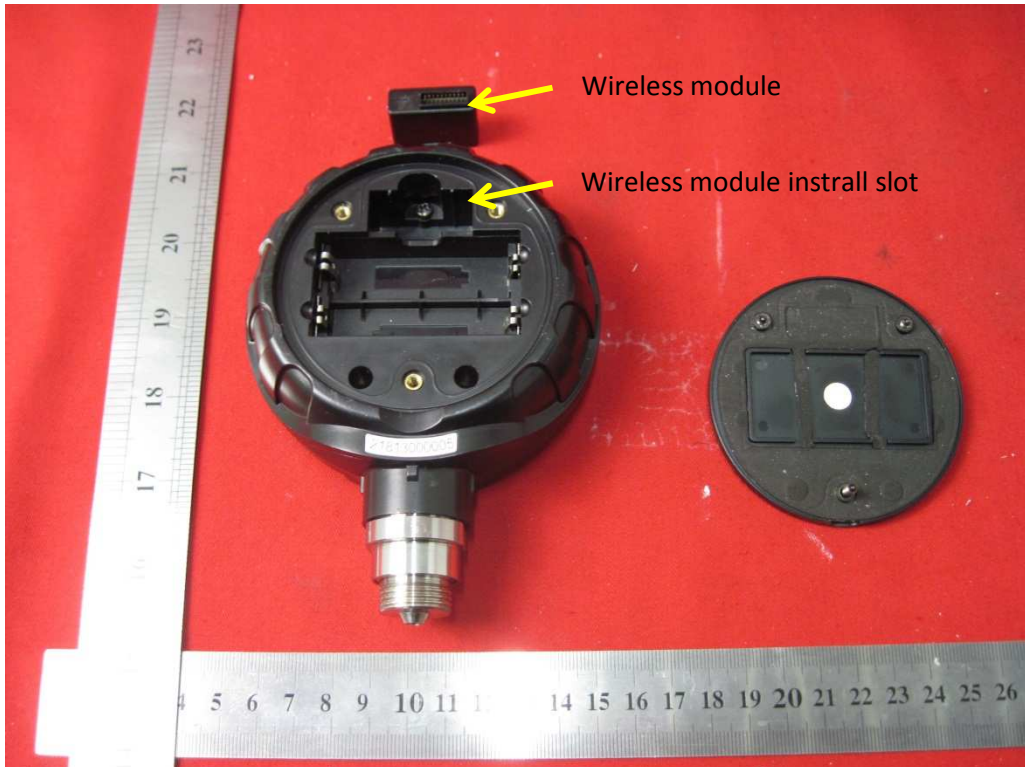
Rear side with removing the wireless module
