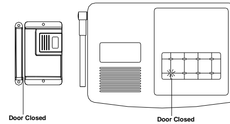
Figure 4. Testing of the magnet sensor transmitter unit and the main receiving unit
