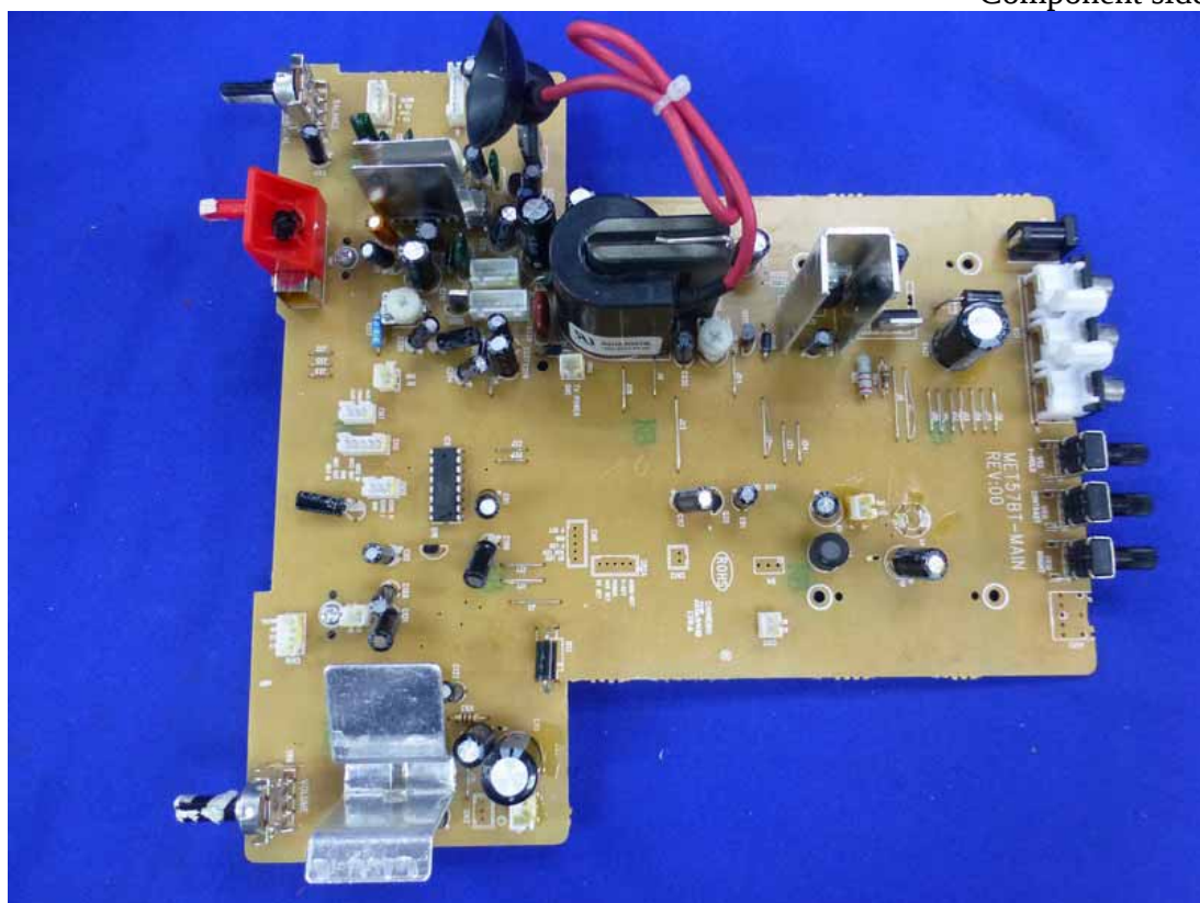
Figure 16 Component side of the PCB
