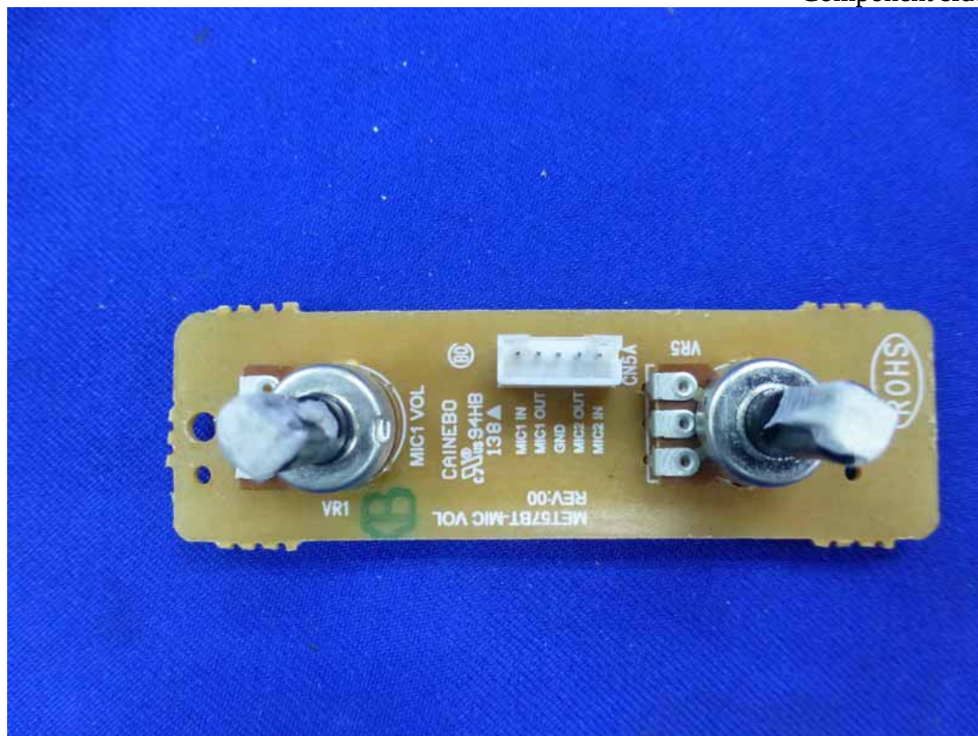
Figure 20 Component side of the PCB
