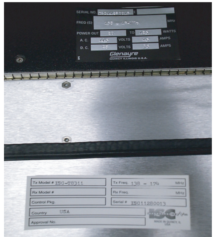
ISC-T8311 TX Information Labels Located on top the unit
