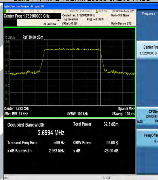
Band4-3MHz-QPSK-20175-15RB#0-PASS
