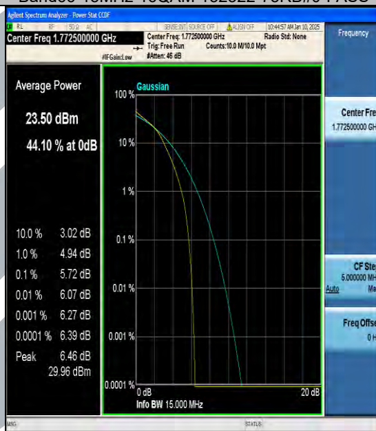
Band66-15MHz-16QAM-132597-75RB#0-PASS
