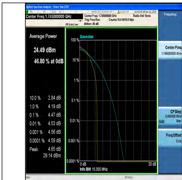
Band66-15MHz-16QAM-132322-1RB#0-PASS
