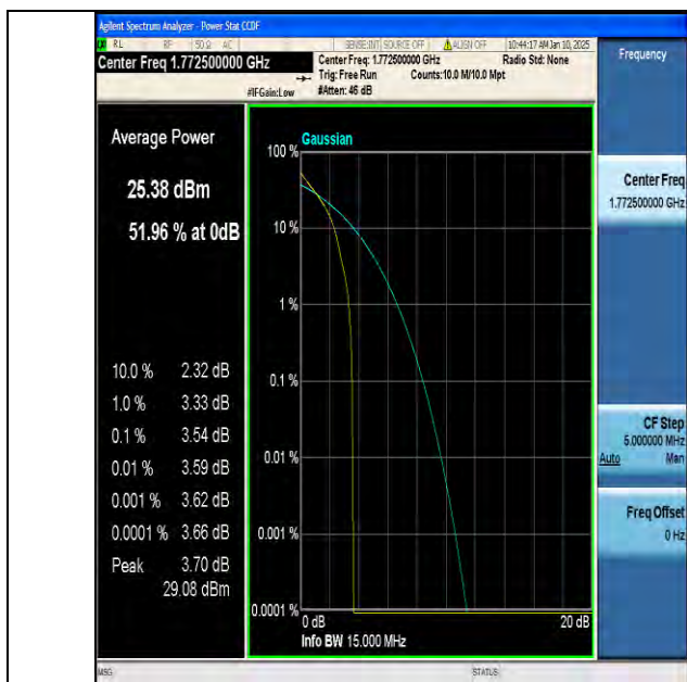
Band66-15MHz-QPSK-132597-1RB#0-PASS
