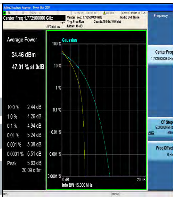
Band66-15MHz-QPSK-132597-75RB#0-PASS
