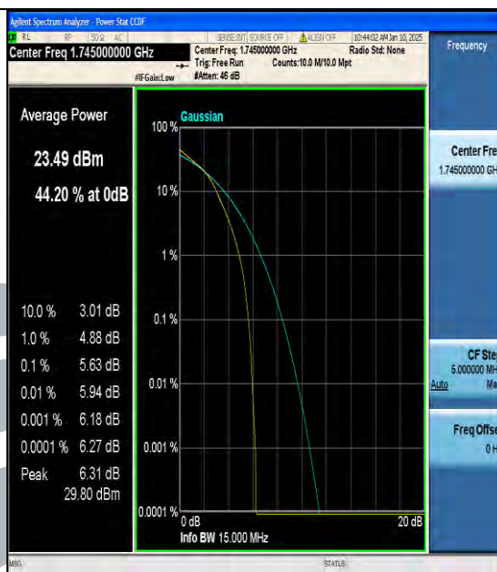
Band66-15MHz-16QAM-132322-75RB#0-PASS
