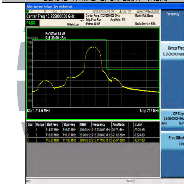
Band12 1.4MHz QPSK 23173 1RB#5
