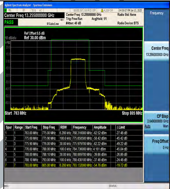
Band13 5MHz QPSK 23255 25RB#0
