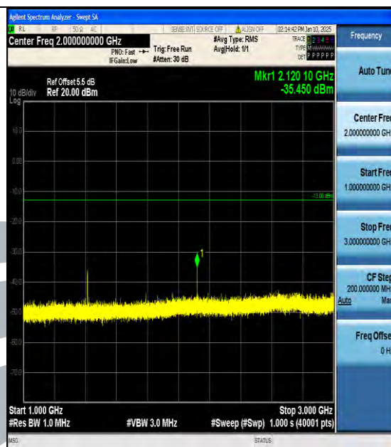
Band17_10MHz_QPSK_23800_1RB#0_1000~3000_1000~3000
