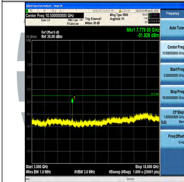
Band38_5MHz_16QAM_38000_1RB#0_3000~18000_3000~18000
