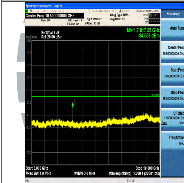
Band38_15MHz_QPSK_38175_1RB#0_3000~18000_3000~18000
