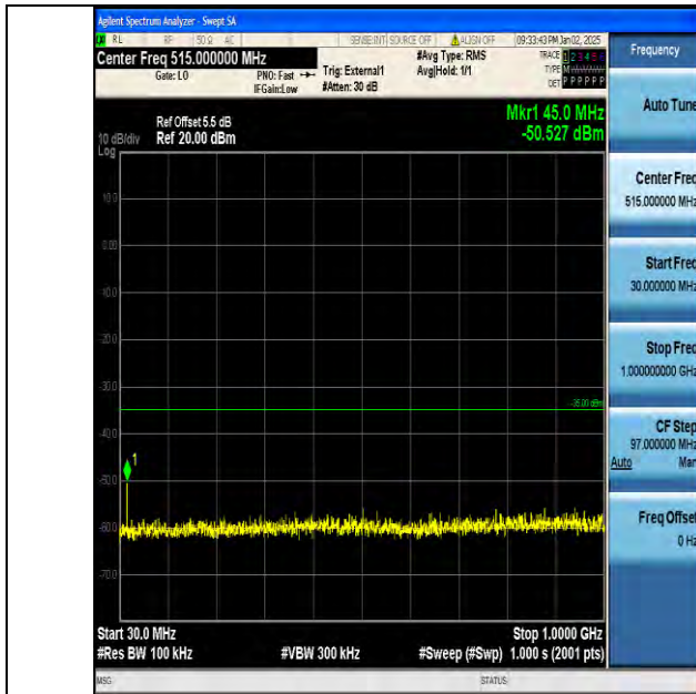
Band38_15MHz_QPSK_38175_1RB#0_30~1000_30~1000
