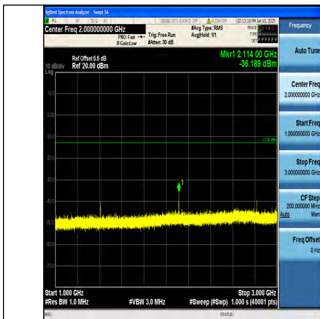
Band17_10MHz_16QAM_23780_1RB#0_1000~3000_1000~3000
