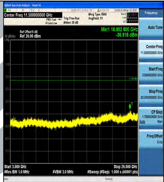
Band66_3MHz_QPSK_132322_1RB#0_3000~20000_3000~20000
