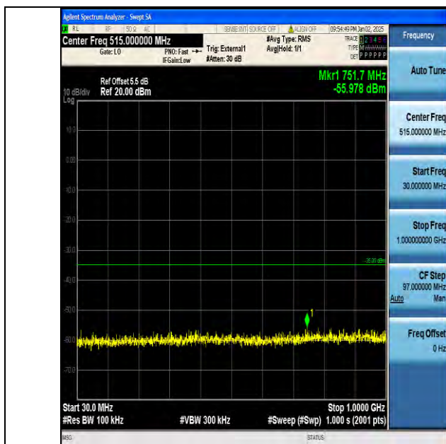
Band38_20MHz_QPSK_37850_1RB#0_30~1000_30~1000
