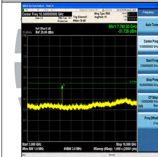
Band38_15MHz_16QAM_38000_1RB#0_3000~18000_3000~18000
