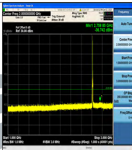
Band38_5MHz_16QAM_38225_1RB#0_1000~3000_1000~3000
