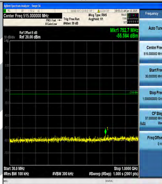
Band66_1.4MHz_QPSK_132322_1RB#0_30~1000_30~1000
