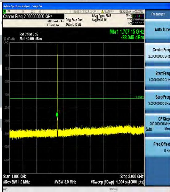
Band66_1.4MHz_16QAM_131979_1RB#0_1000~3000_1000~3000
