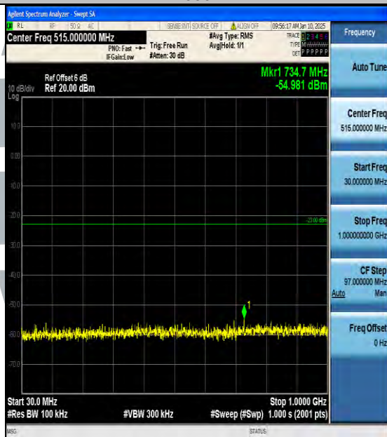
Band66_1.4MHz_QPSK_132665_1RB#0_30~1000_30~1000
