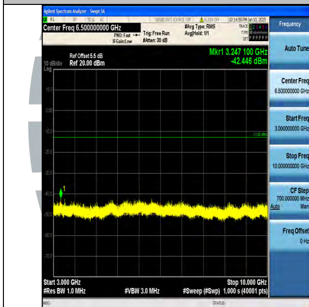
Band17_10MHz_QPSK_23800_1RB#0_3000~10000_3000~10000
