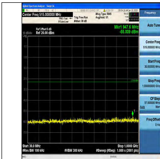
Band66_1.4MHz_QPSK_131979_1RB#0_30~1000_30~1000
