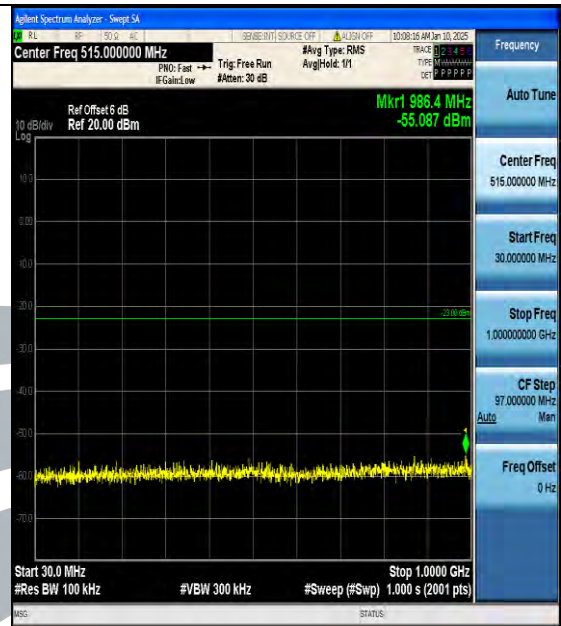
Band66_3MHz_QPSK_132322_1RB#0_30~1000_30~1000
