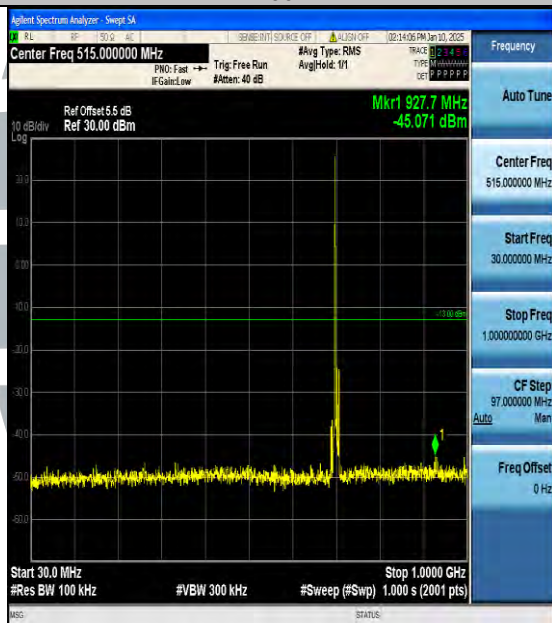
Band17_10MHz_16QAM_23790_1RB#0_30~1000_30~1000
