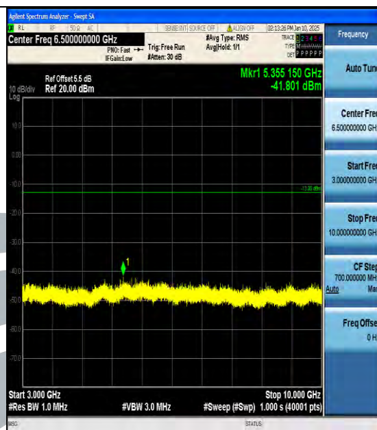
Band17_10MHz_16QAM_23780_1RB#0_3000~10000_3000~10000
