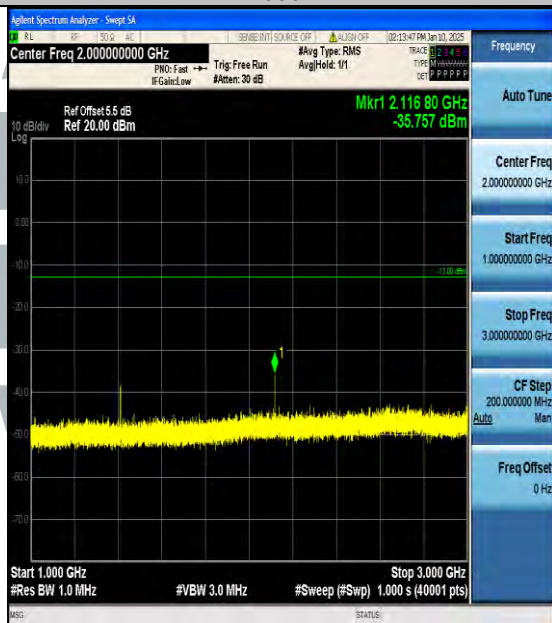
Band17_10MHz_QPSK_23790_1RB#0_1000~3000_1000~3000
