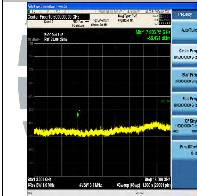
Band38_20MHz_16QAM_38150_1RB#0_3000~18000_3000~18000
