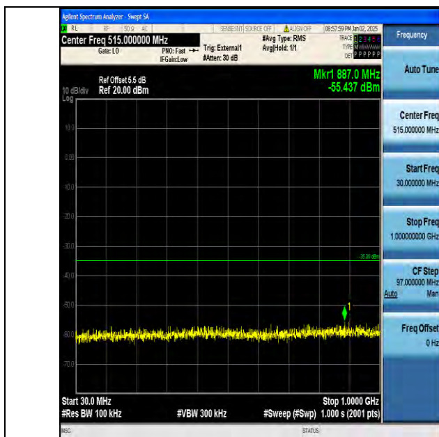
Band38_10MHz_QPSK_37800_1RB#0_30~1000_30~1000
