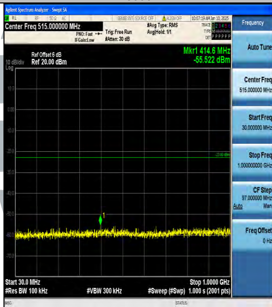
Band66_3MHz_QPSK_131987_1RB#0_30~1000_30~1000
