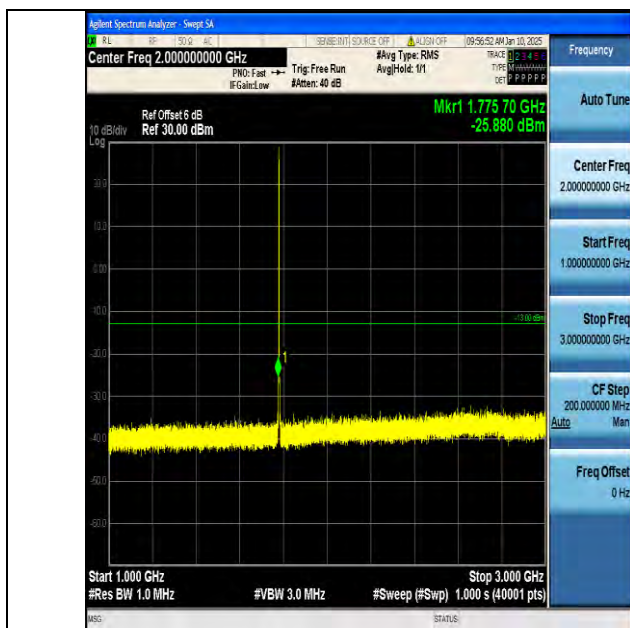
Band66_1.4MHz_16QAM_132665_1RB#0_1000~3000_1000~3000
