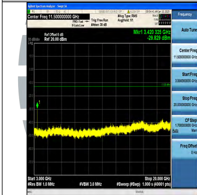
Band66_1.4MHz_QPSK_131979_1RB#0_3000~20000_3000~20000
