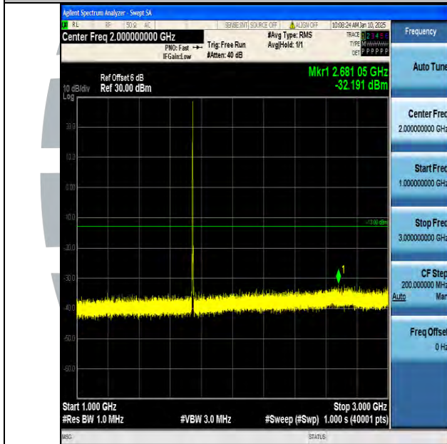
Band66_3MHz_QPSK_132322_1RB#0_1000~3000_1000~3000
