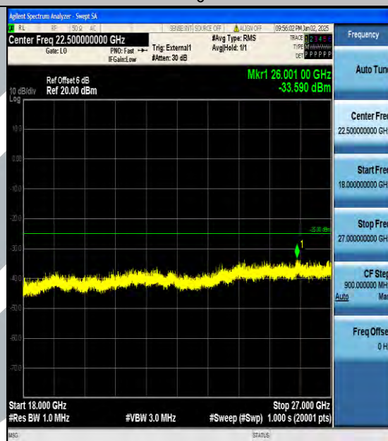
Band38_20MHz_QPSK_37850_1RB#0_18000~27000_18000~27000
