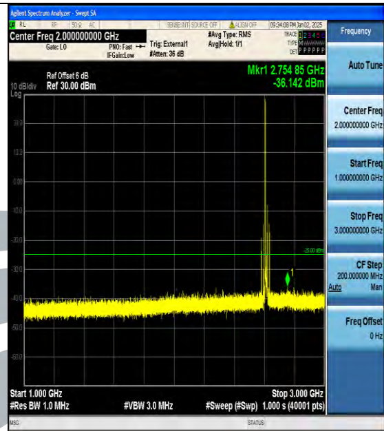
Band38_15MHz_QPSK_38175_1RB#0_1000~3000_1000~3000
