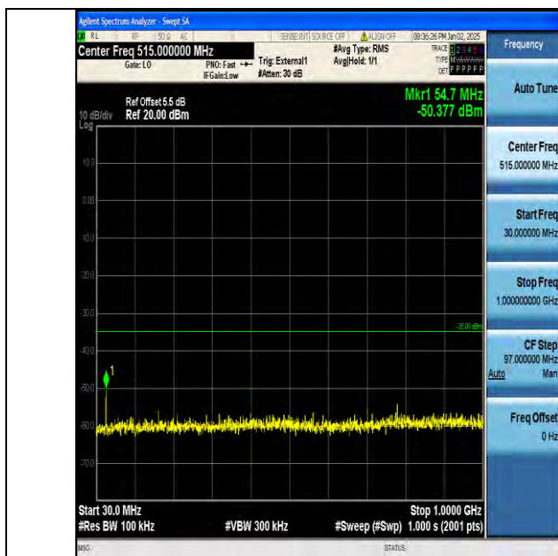
Band38_5MHz_16QAM_38225_1RB#0_30~1000_30~1000
