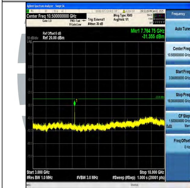
Band38_15MHz_QPSK_38000_1RB#0_3000~18000_3000~18000
