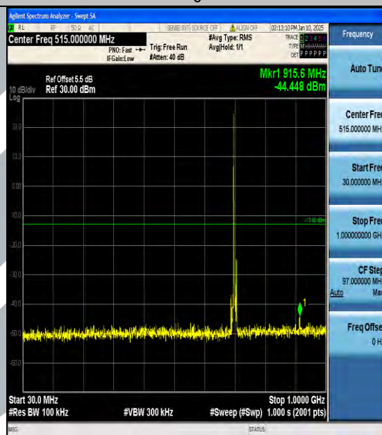
Band17_10MHz_16QAM_23780_1RB#0_30~1000_30~1000
