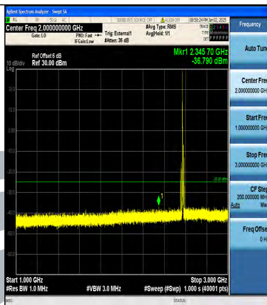
Band38_10MHz_QPSK_37800_1RB#0_1000~3000_1000~3000
