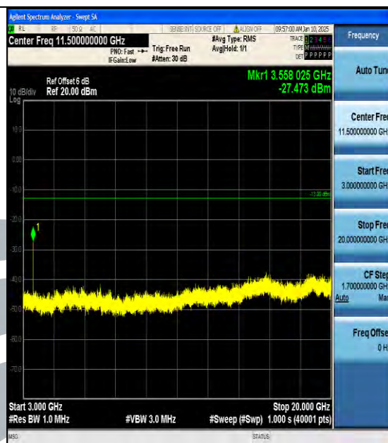
Band66_1.4MHz_16QAM_132665_1RB#0_3000~20000_3000~20000
