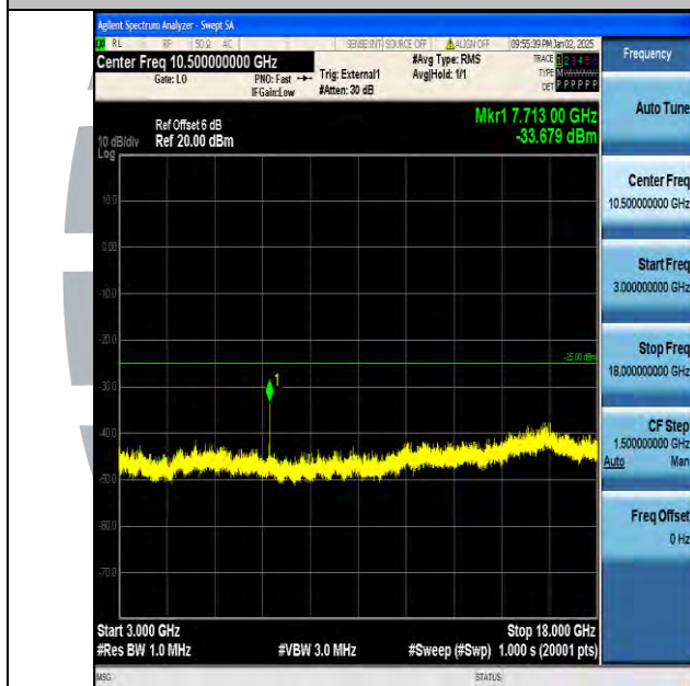
Band38_20MHz_QPSK_37850_1RB#0_3000~18000_3000~18000
