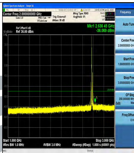
Band38_20MHz_QPSK_37850_1RB#0_1000~3000_1000~3000
