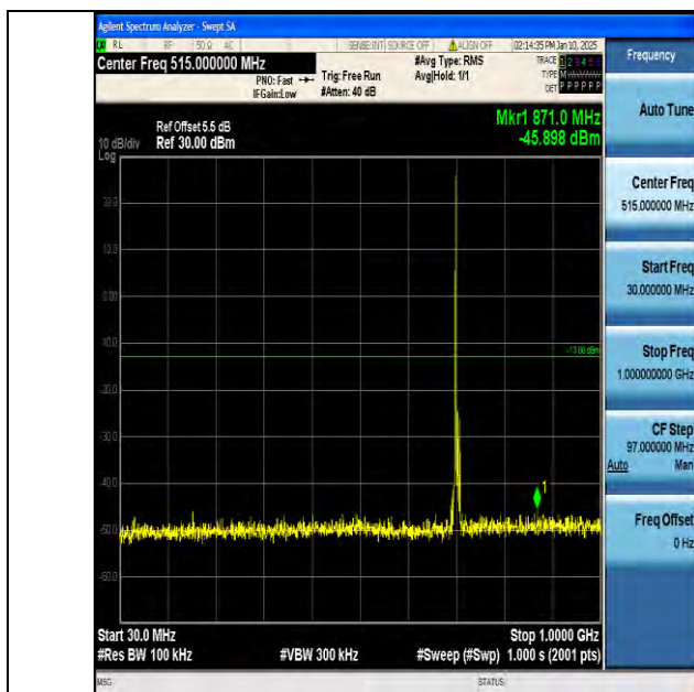
Band17_10MHz_QPSK_23800_1RB#0_30~1000_30~1000
