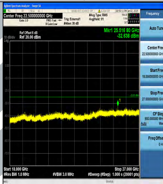
Band38_10MHz_QPSK_37800_1RB#0_18000~27000_18000~27000
