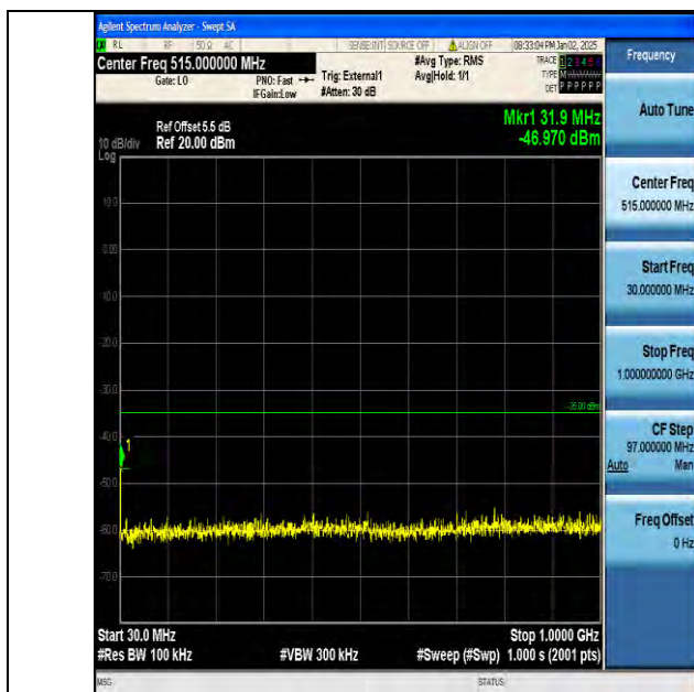
Band38_5MHz_16QAM_38000_1RB#0_30~1000_30~1000
