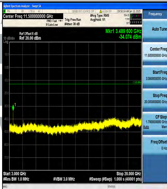
Band66_1.4MHz_16QAM_132322_1RB#0_3000~20000_3000~20000
