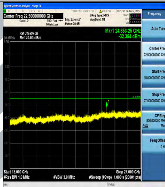
Band38_20MHz_16QAM_37850_1RB#0_18000~27000_18000~27000
