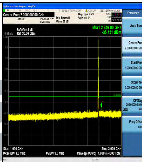
Band38_5MHz_16QAM_38000_1RB#0_1000~3000_1000~3000
