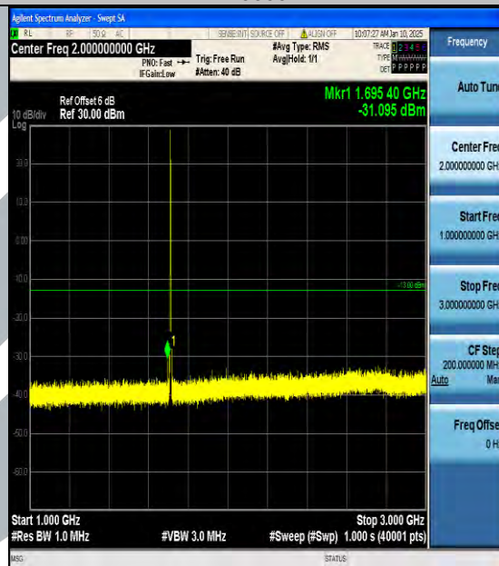
Band66_3MHz_QPSK_131987_1RB#0_1000~3000_1000~3000
