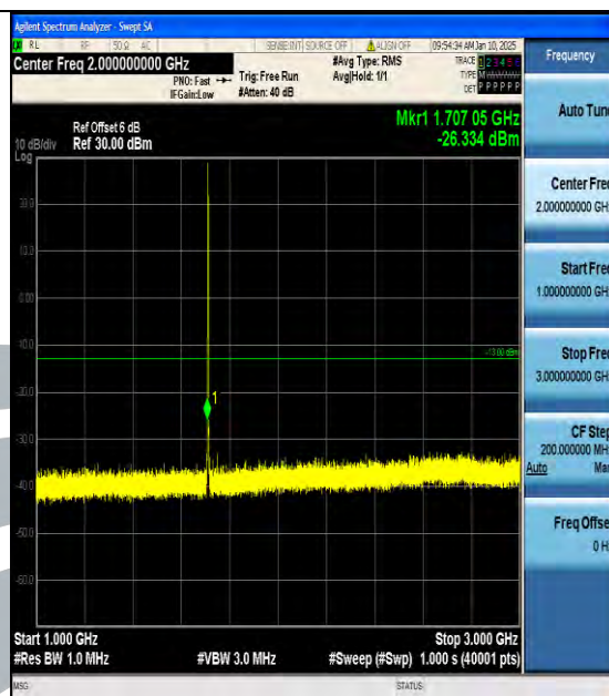
Band66_1.4MHz_QPSK_131979_1RB#0_1000~3000_1000~3000
