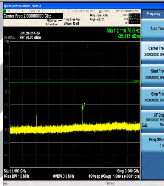
Band17_10MHz_16QAM_23790_1RB#0_1000~3000_1000~3000
