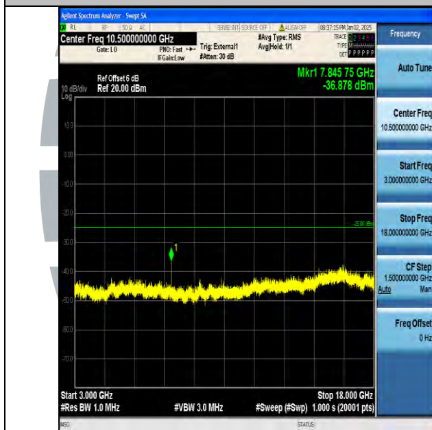
Band38_5MHz_16QAM_38225_1RB#0_3000~18000_3000~18000
