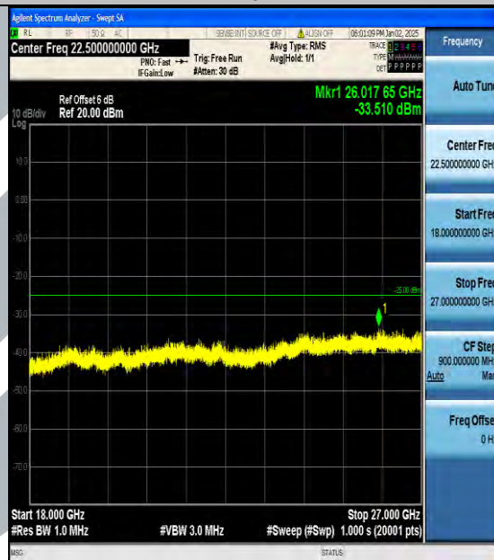
Band7_10MHz_16QAM_20800_1RB#0_18000~27000_18000~27000
