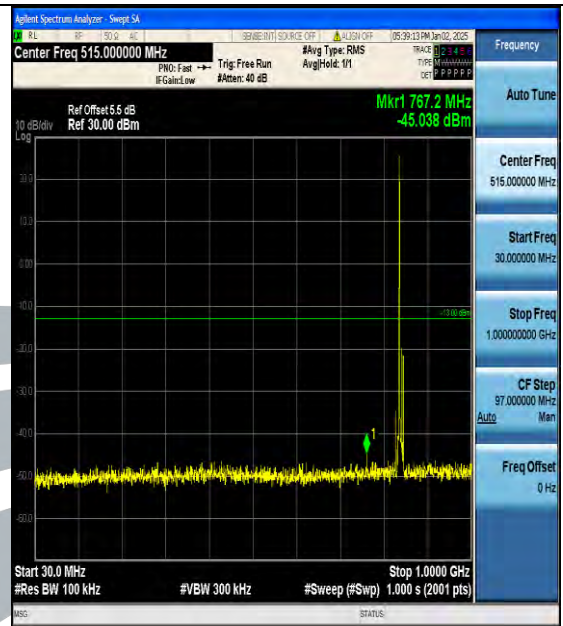
Band5_10MHz_16QAM_20600_1RB#0_30~1000_30~1000
