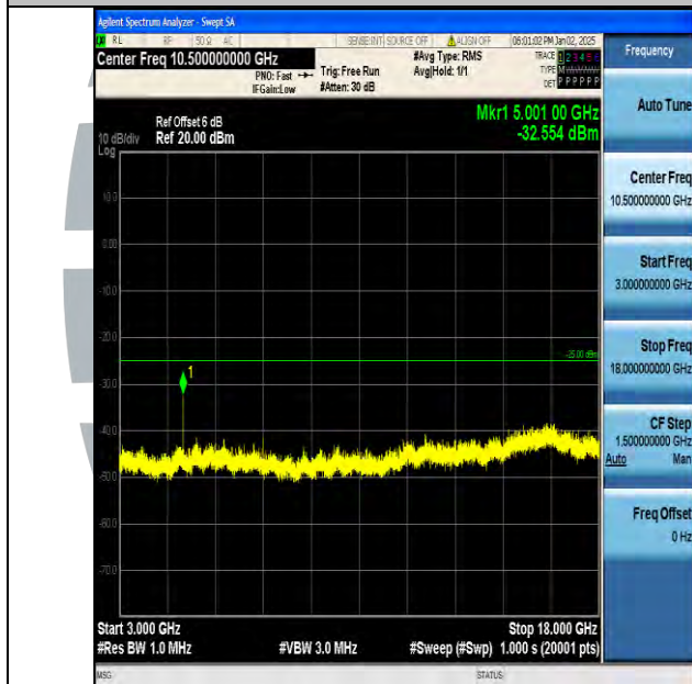
Band7_10MHz_16QAM_20800_1RB#0_3000~18000_3000~18000
