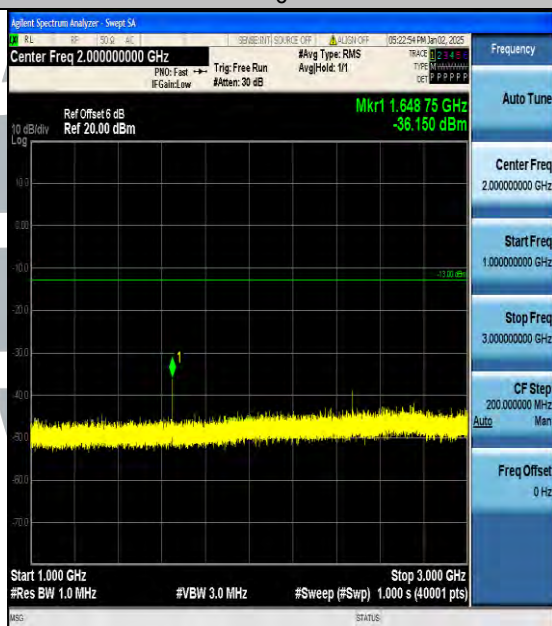
Band5_5MHz_16QAM_20425_1RB#0_1000~3000_1000~3000
