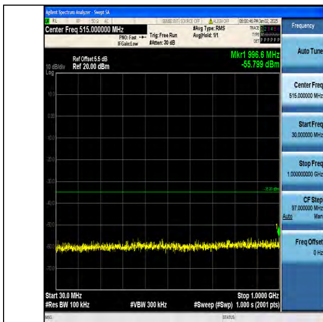
Band7_10MHz_16QAM_20800_1RB#0_30~1000_30~1000
