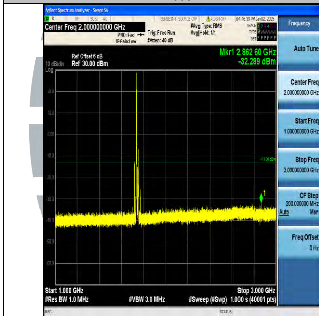
Band4_20MHz_16QAM_20300_1RB#0_1000~3000_1000~3000
