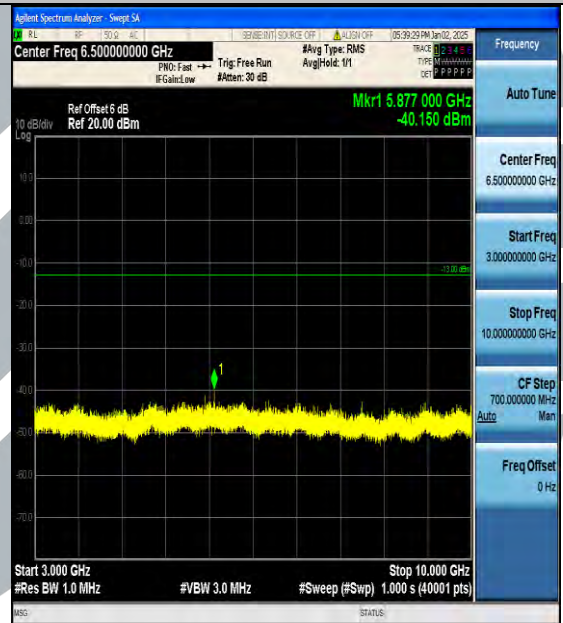
Band5_10MHz_16QAM_20600_1RB#0_3000~10000_3000~10000
