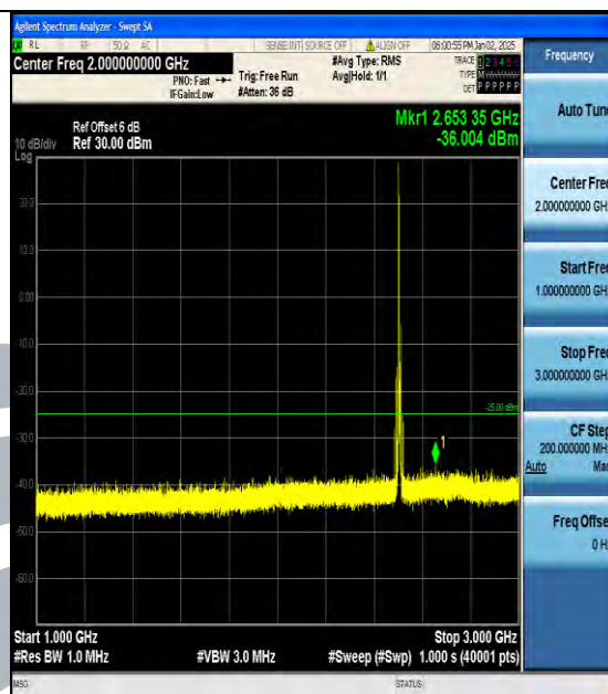
Band7_10MHz_16QAM_20800_1RB#0_1000~3000_1000~3000
