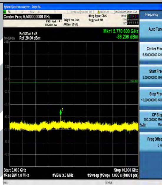
Band5_5MHz_16QAM_20425_1RB#0_3000~10000_3000~10000
