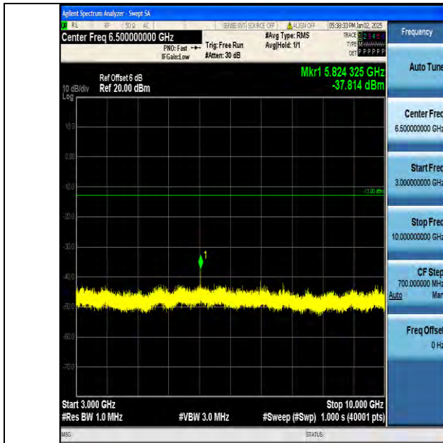
Band5_10MHz_16QAM_20525_1RB#0_3000~10000_3000~10000
