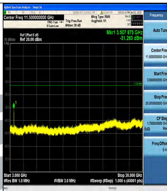
Band4_1.4MHz_16QAM_20393_1RB#0_3000~20000_3000~20000
