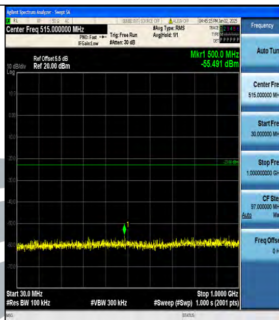
Band4_20MHz_QPSK_20175_1RB#0_30~1000_30~1000
