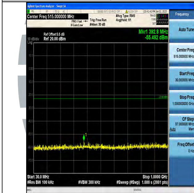
Band2_20MHz_16QAM_18900_1RB#0_30~1000_30~1000
