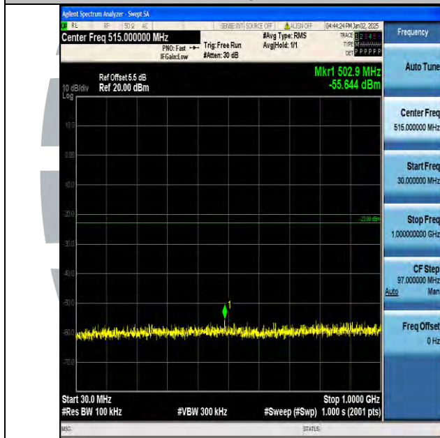
Band4_20MHz_QPSK_20050_1RB#0_30~1000_30~1000
