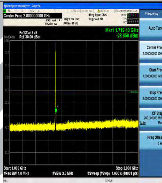
Band4_3MHz_QPSK_19965_1RB#0_1000~3000_1000~3000
