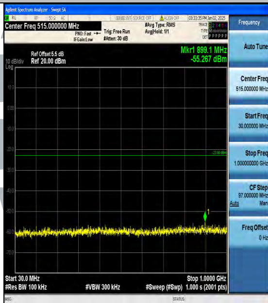
Band2_15MHz_QPSK_19125_1RB#0_30~1000_30~1000
