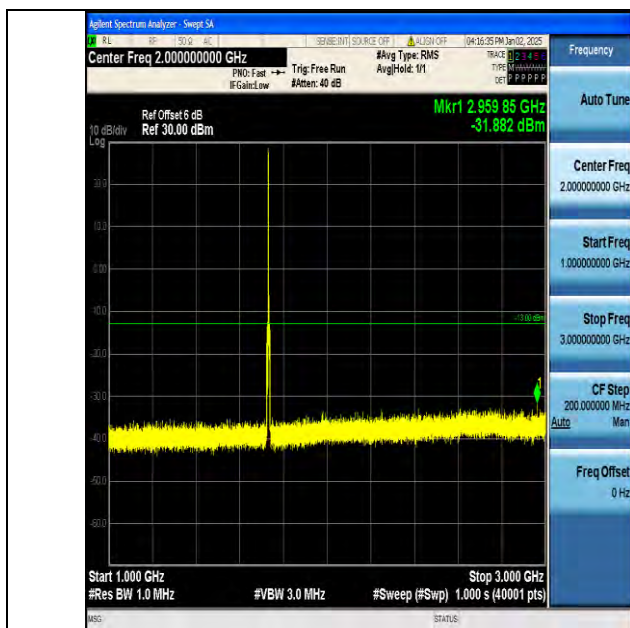
Band4_5MHz_QPSK_20175_1RB#0_1000~3000_1000~3000
