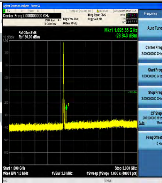
Band2_15MHz_16QAM_18675_1RB#0_1000~3000_1000~3000
