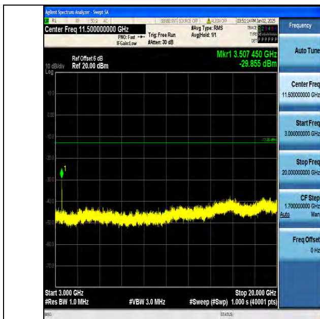
Band4_1.4MHz_QPSK_20393_1RB#0_3000~20000_3000~20000
