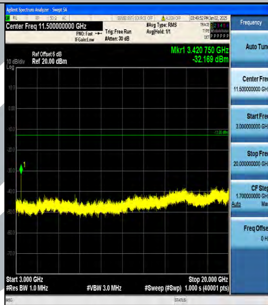
Band4_1.4MHz_16QAM_19957_1RB#0_3000~20000_3000~20000
