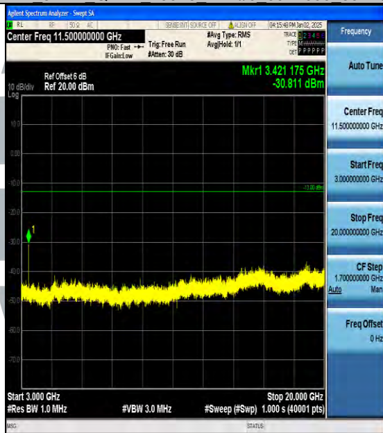
Band4_5MHz_QPSK_19975_1RB#0_3000~20000_3000~2000 0
