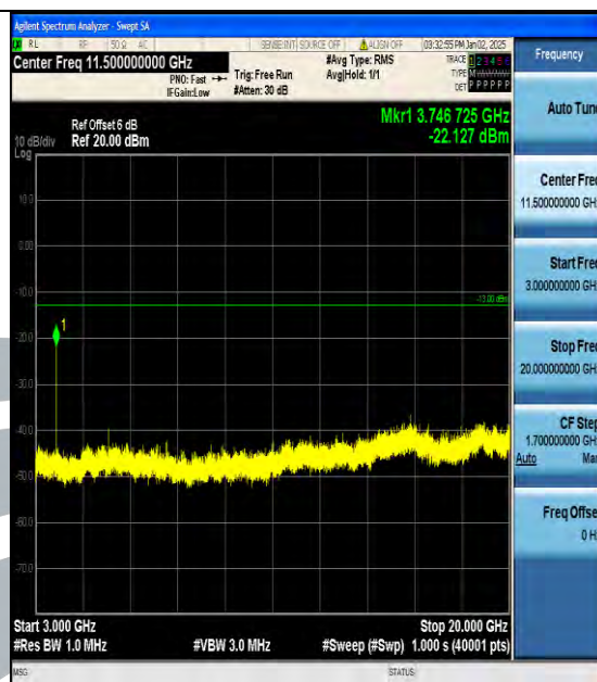
Band2_15MHz_QPSK_18900_1RB#0_3000~20000_3000~20000
