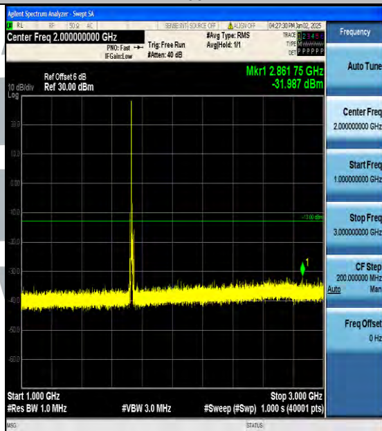
Band4_10MHz_QPSK_20175_1RB#0_1000~3000_1000~3000
