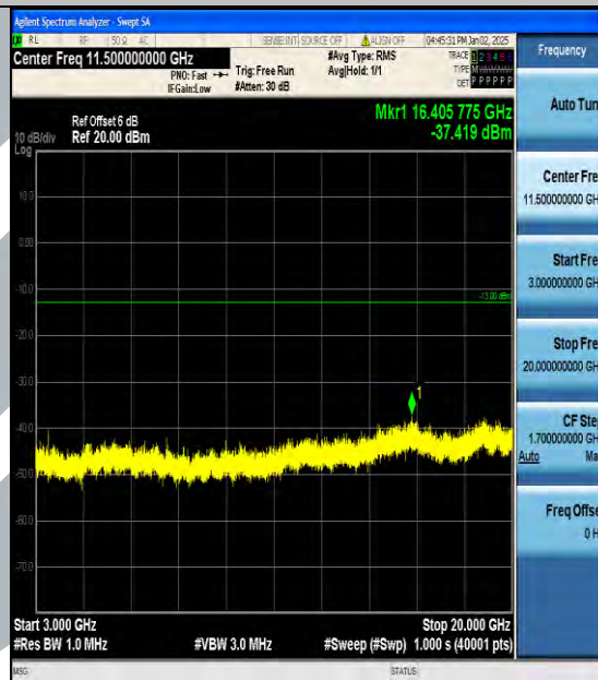
Band4_20MHz_QPSK_20175_1RB#0_3000~20000_3000~20000
