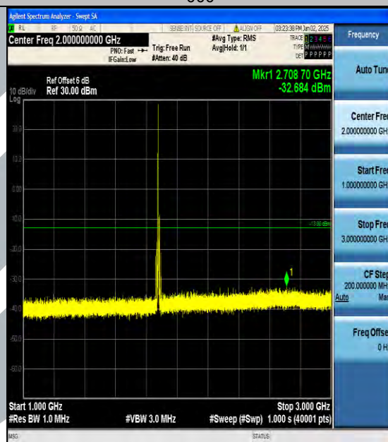
Band2_10MHz_16QAM_18900_1RB#0_1000~3000_1000~3000
