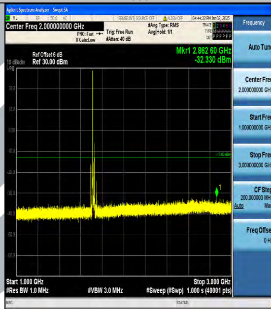
Band4_20MHz_QPSK_20050_1RB#0_1000~3000_1000~3000
