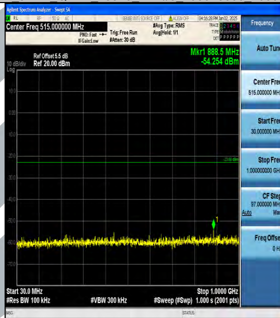
Band4_5MHz_QPSK_20175_1RB#0_30~1000_30~1000
