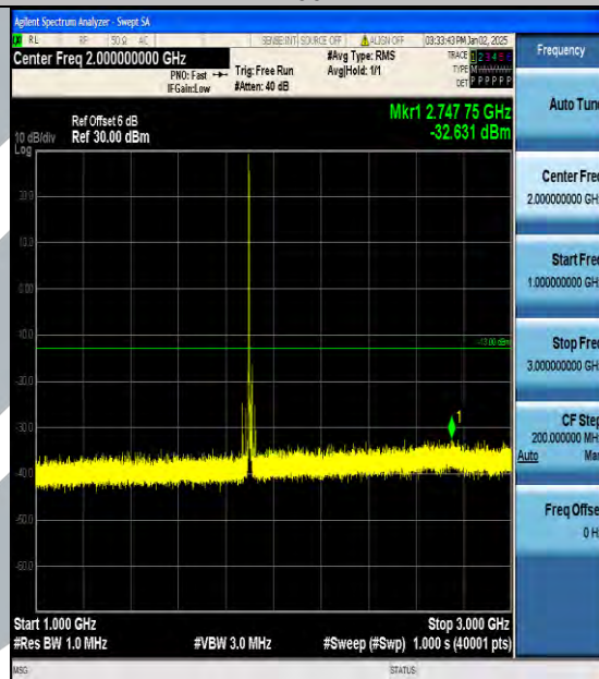
Band2_15MHz_QPSK_19125_1RB#0_1000~3000_1000~3000
