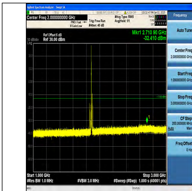
Band2_15MHz_QPSK_18900_1RB#0_1000~3000_1000~3000
