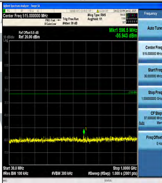
Band4_3MHz_QPSK_19965_1RB#0_30~1000_30~1000
