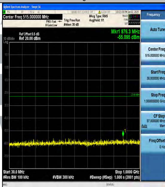
Band2_10MHz_16QAM_18900_1RB#0_30~1000_30~1000
