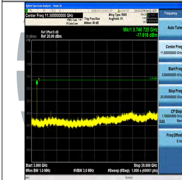
Band2_15MHz_16QAM_18900_1RB#0_3000~20000_3000~20000
