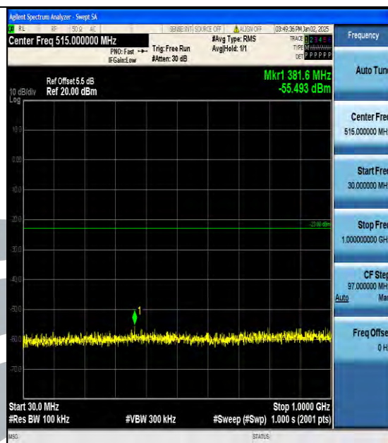
Band4_1.4MHz_16QAM_19957_1RB#0_30~1000_30~1000
