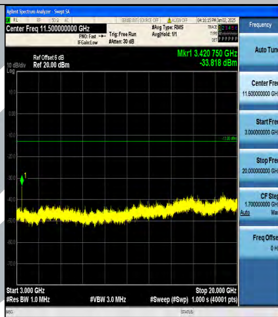
Band4_5MHz_16QAM_19975_1RB#0_3000~20000_3000~20000
