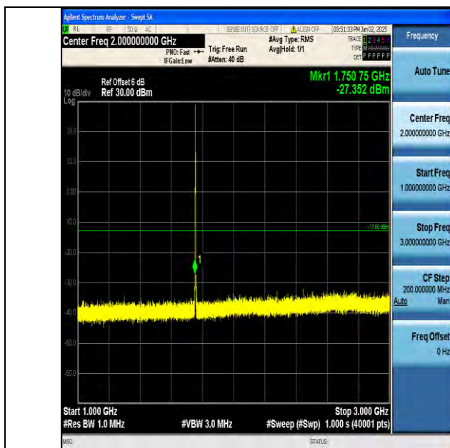
Band4_1.4MHz_16QAM_20393_1RB#0_1000~3000_1000~3000
