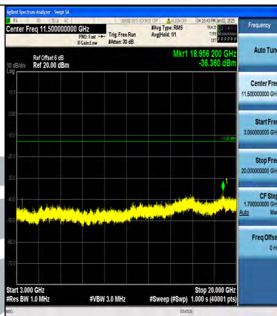
Band4_5MHz_QPSK_20175_1RB#0_3000~20000_3000~20000
