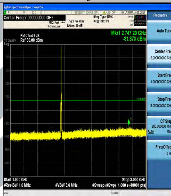
Band4_5MHz_QPSK_20375_1RB#0_1000~3000_1000~3000
