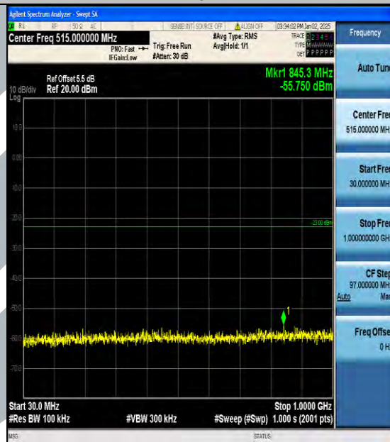
Band2_15MHz_16QAM_19125_1RB#0_30~1000_30~1000
