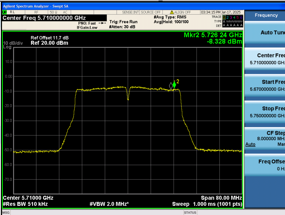
11AC40SISO-Ant1-5710_UNII-3-PASS
