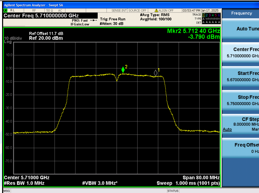
11AC40SISO-Ant1-5710_UNII-2C-PASS
