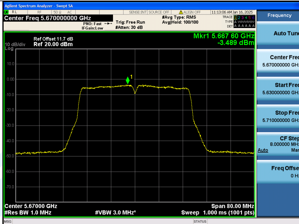
11N40SISO-Ant1-5670-PASS
