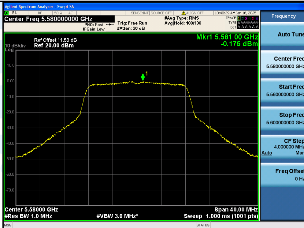
11A-Ant1-5580-PASS
