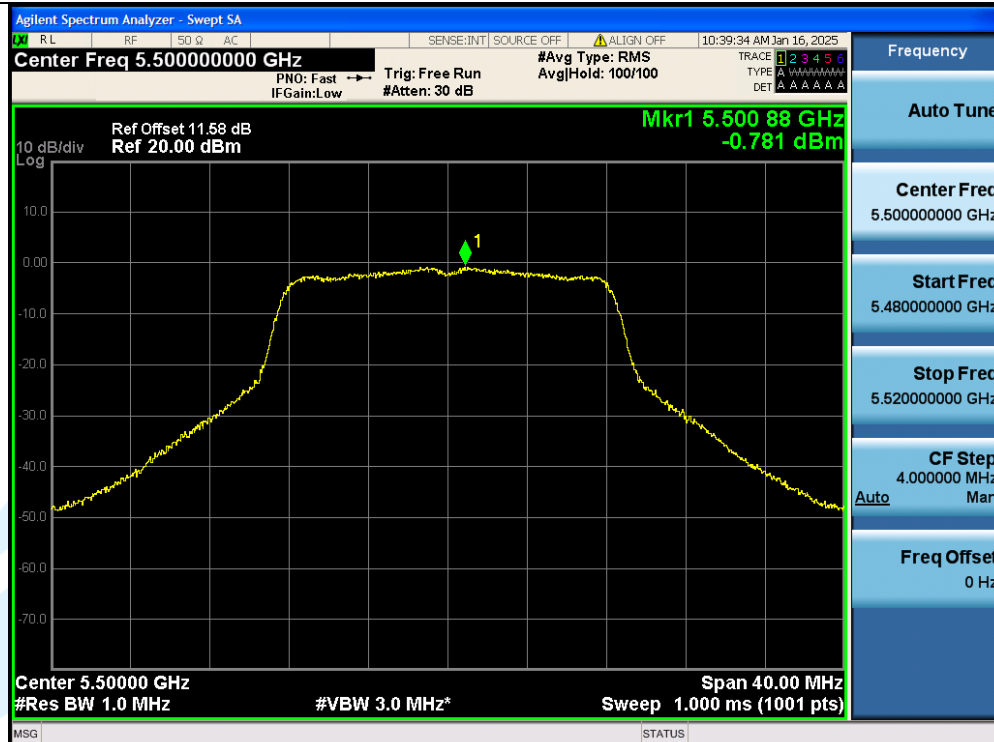
11A-Ant1-5500-PASS
