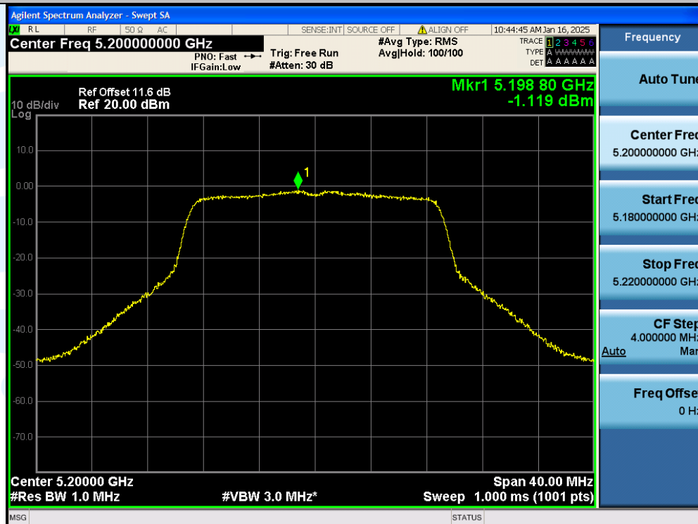
11N20SISO-Ant1-5200-PASS
