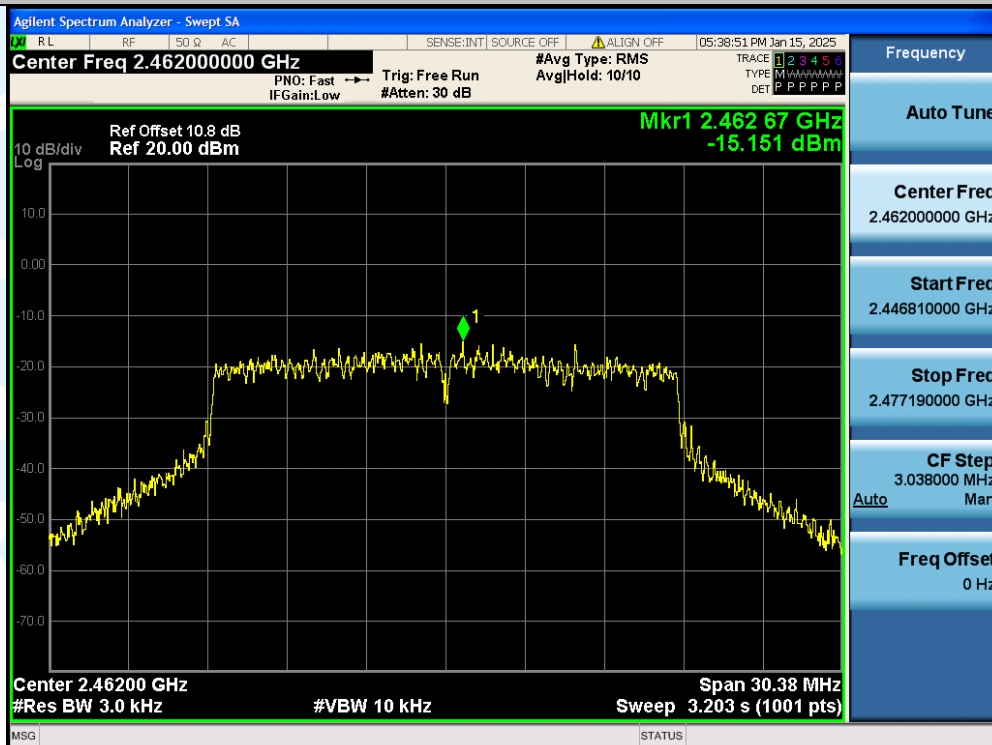
11N20SISO-Ant1-2462MHz-PASS
