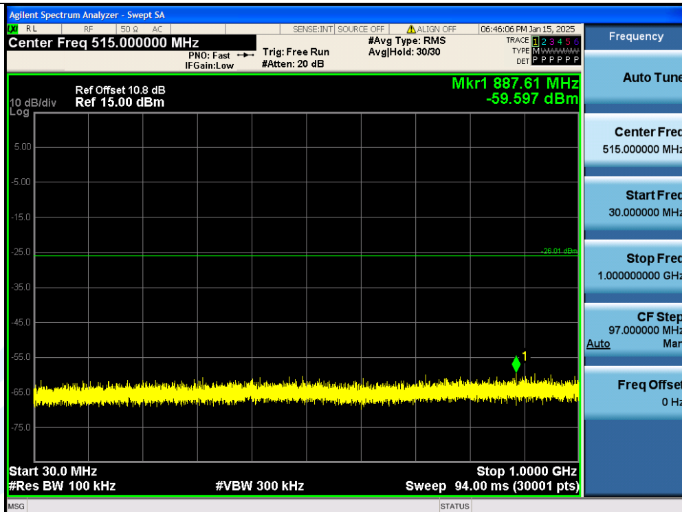
11N40SISO-Ant1-2462MHz-30~1000 MHz-PASS
