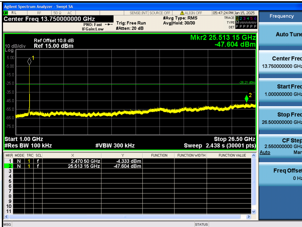
11N20SISO-Ant1-2472MHz-1000~26500MHz-PASS
