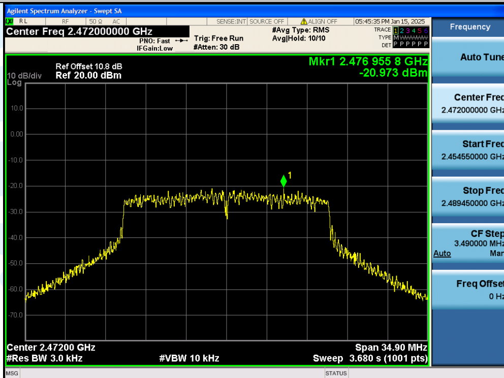
11N20SISO-Ant1-2472MHz-PASS
