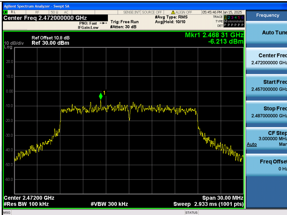
11N20SISO-Ant1-2472MHz-0~Reference-PASS
