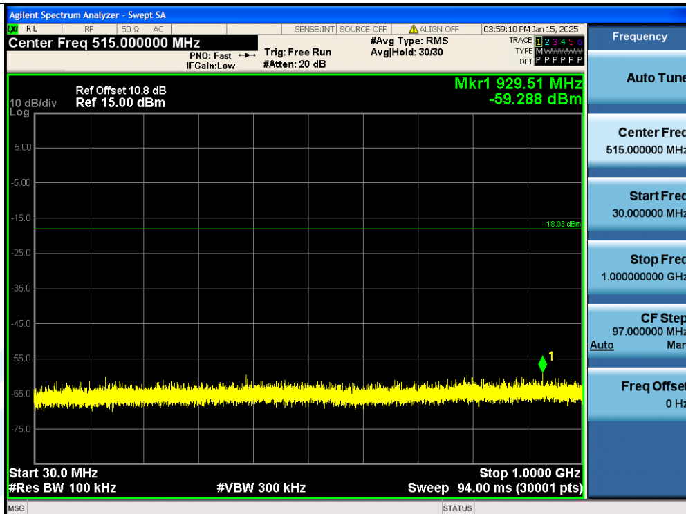
11B-Ant1-2437MHz-30~1000 MHz-PASS
