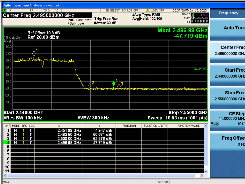
11N40SISO-Ant1-2457MHz-PASS
