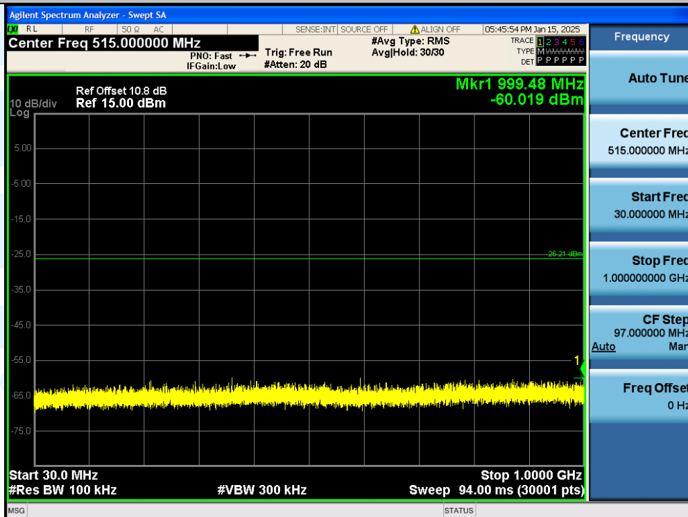
11N20SISO-Ant1-2472MHz-30~1000 MHz-PASS
