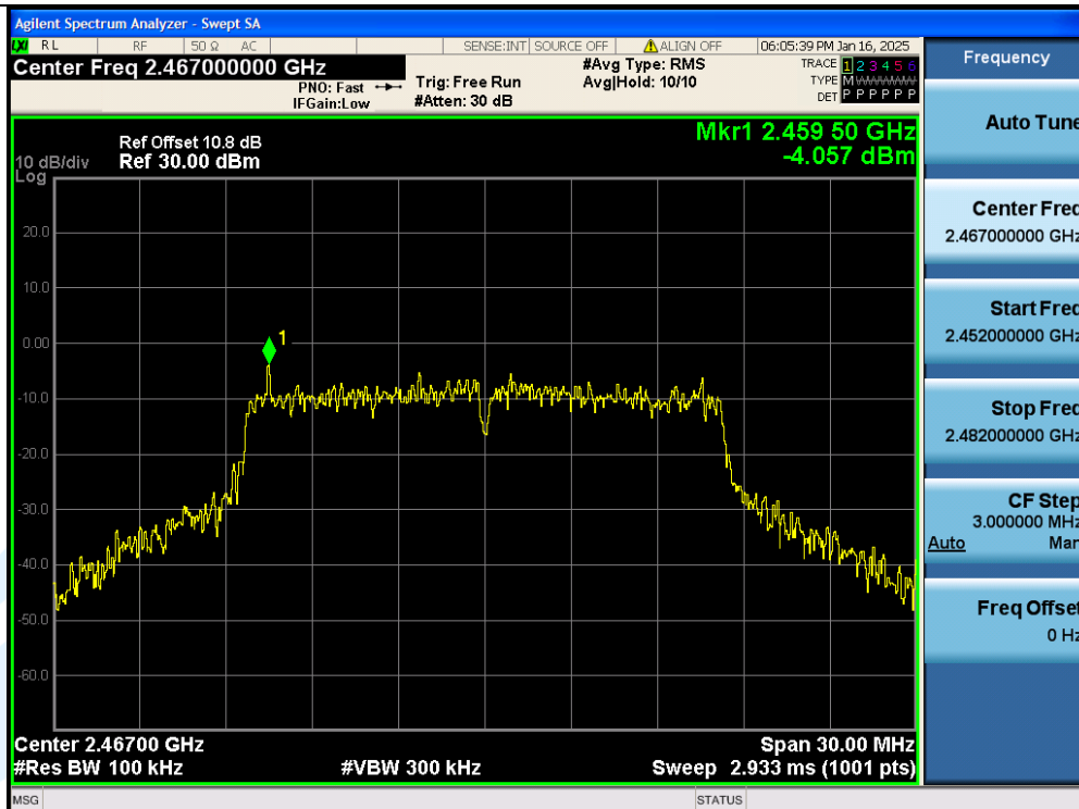
11G-Ant1-2467MHz-0-Reference-PASS
