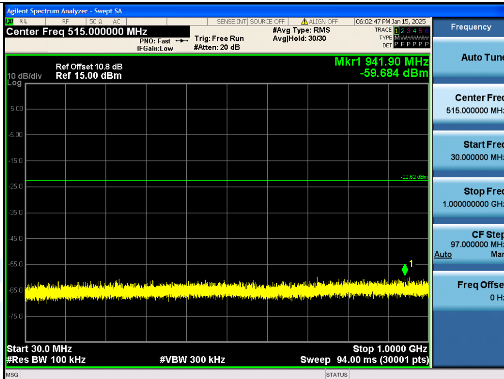
11N40SISO-Ant1-2452MHz-30~1000 MHz-PASS
