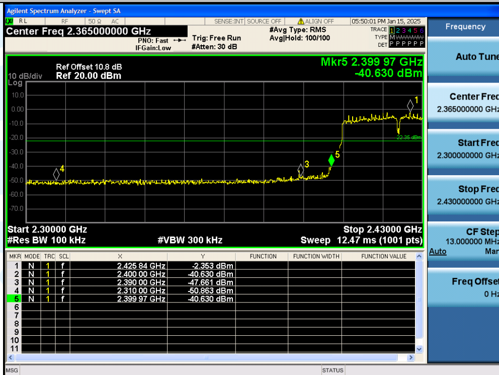
11N40SISO-Ant1-2422MHz-PASS
