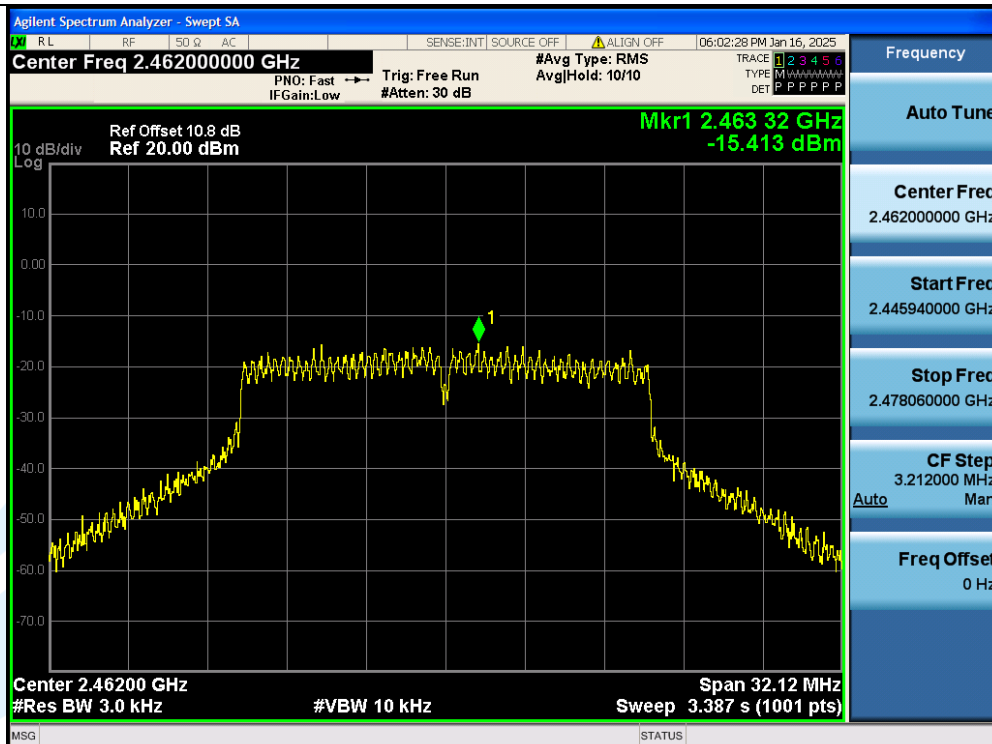
11G-Ant1-2462MHz-PASS
