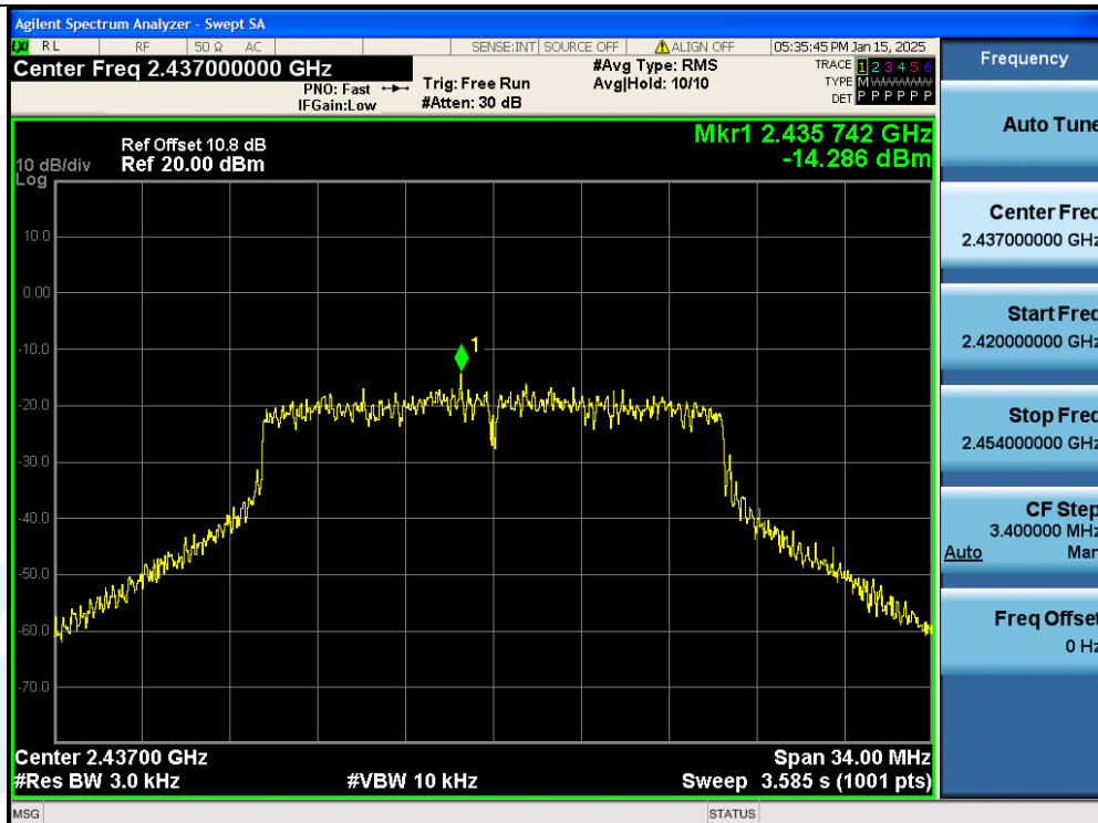
11N20SISO-Ant1-2437MHz-PASS
