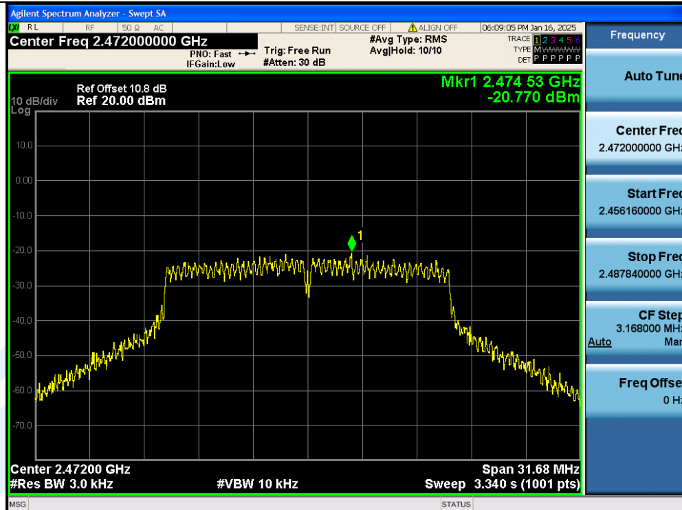
11G-Ant1-2472MHz-PASS
