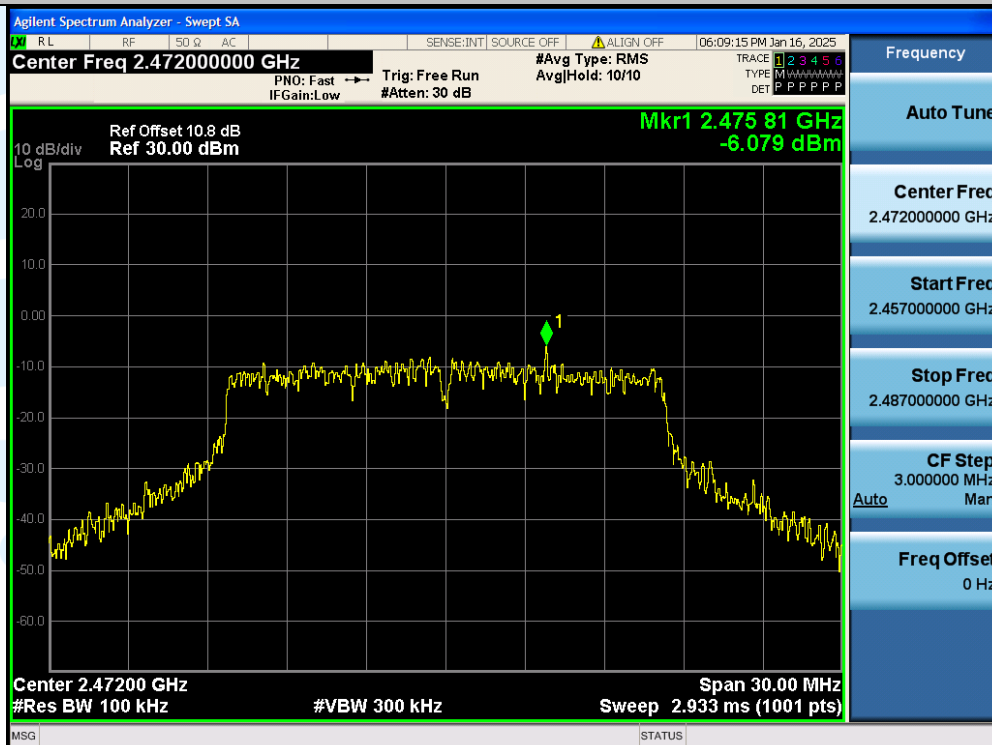
11G-Ant1-2472MHz-0~Reference-PASS
