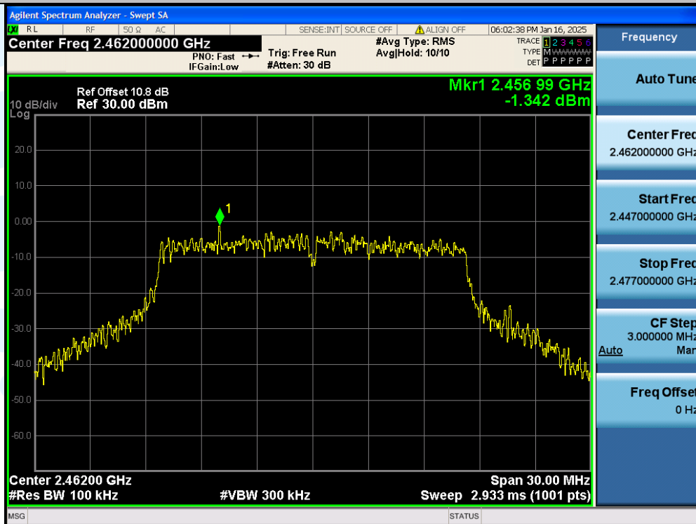
11G-Ant1-2462MHz-0~Reference-PASS
