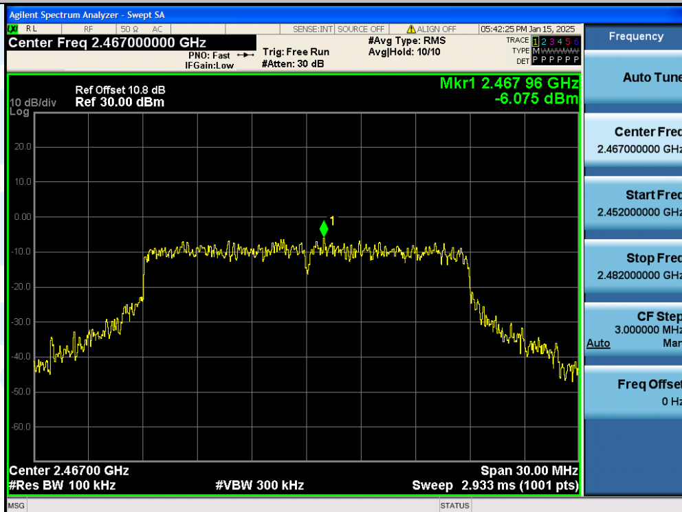
11N20SISO-Ant1-2467MHz-0~Reference-PASS
