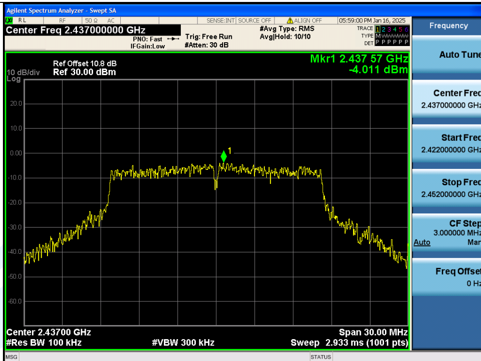
11G-Ant1-2437MHz-0-Reference-PASS
