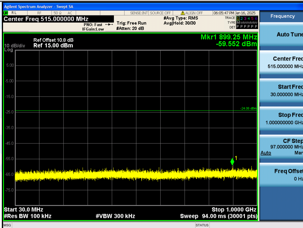
11G-Ant1-2467MHz-30~1000 MHz-PASS
