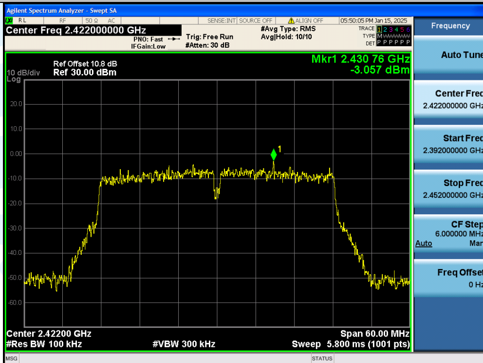
11N40SISO-Ant1-2422MHz-0~Reference-PASS
