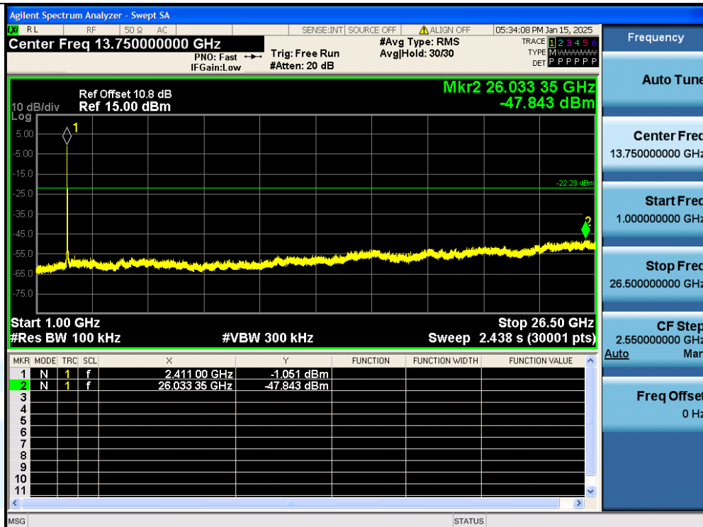
11N20SISO-Ant1-2412MHz-1000~26500MHz-PASS
