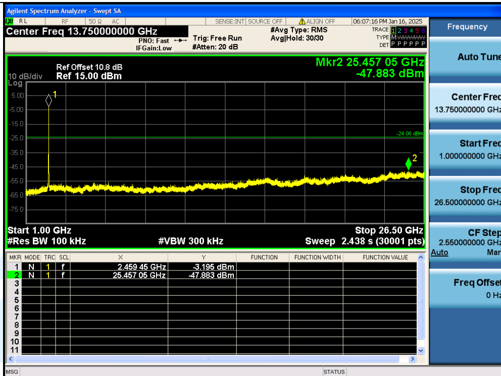
11G-Ant1-2467MHz-1000~26500MHz-PASS
