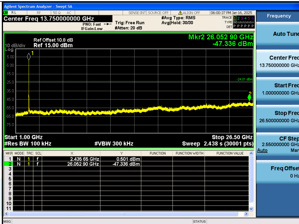
11G-Ant1-2437MHz-1000~26500MHz-PASS
