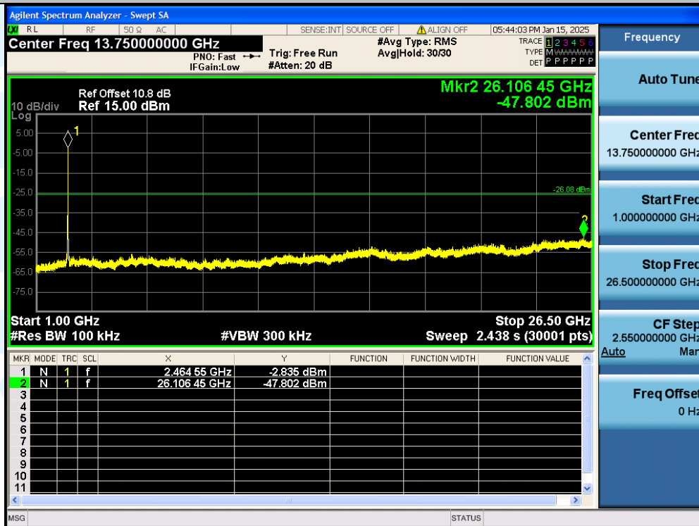
11N20SISO-Ant1-2467MHz-1000~26500MHz-PASS
