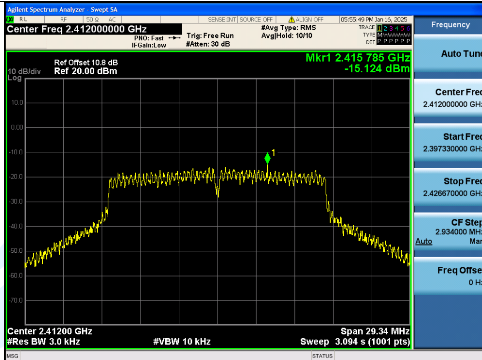
11G-Ant1-2412MHz-PASS
