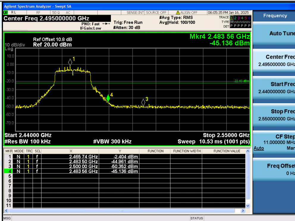
11G-Ant1-2467MHz-PASS
