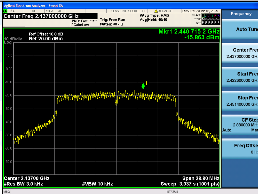
11G-Ant1-2437MHz-PASS
