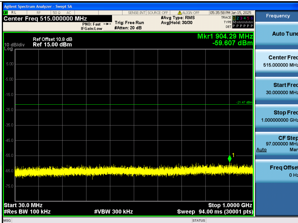
11N20SISO-Ant1-2437MHz-30~1000 MHz-PASS
