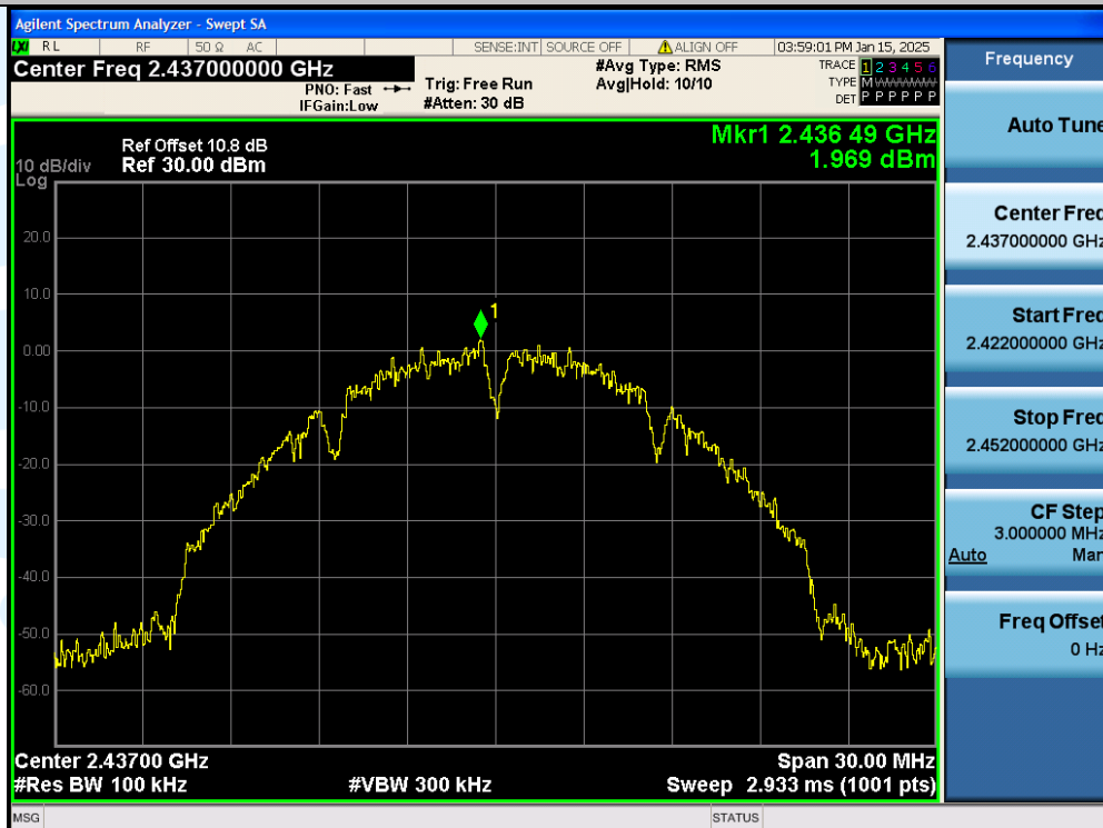
11B-Ant1-2437MHz-0~Reference-PASS
