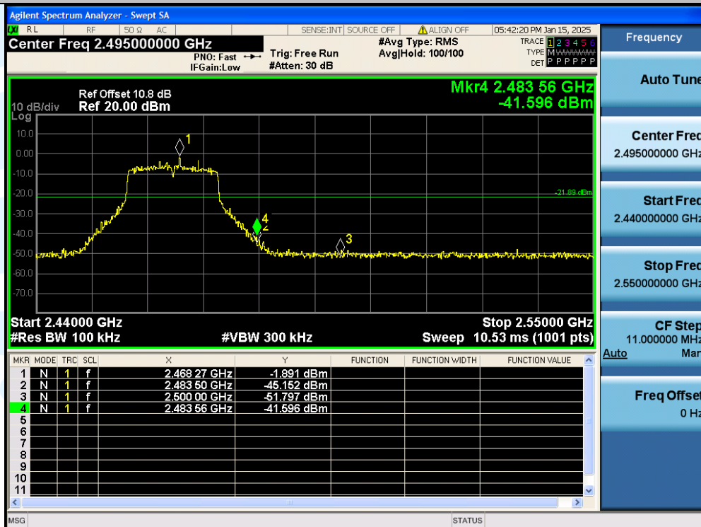
11N20SISO-Ant1-2467MHz-PASS
