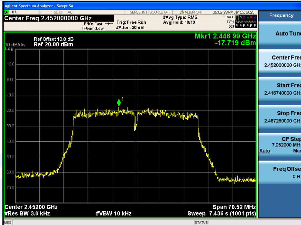
11N40SISO-Ant1-2452MHz-PASS
