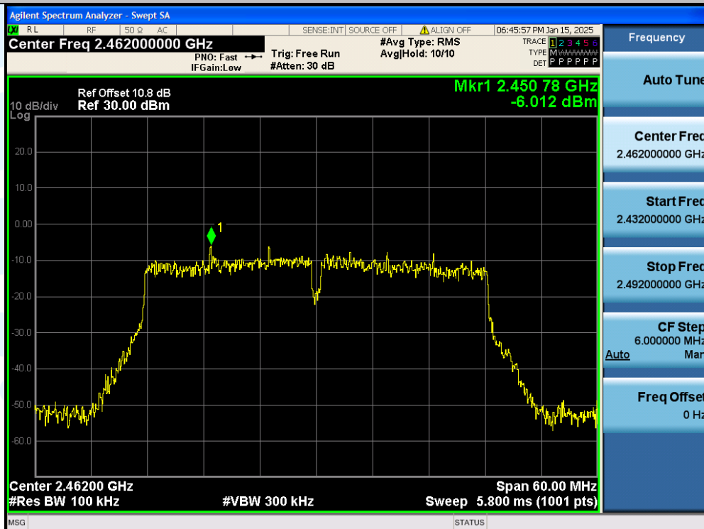
11N40SISO-Ant1-2462MHz-0~Reference-PASS
