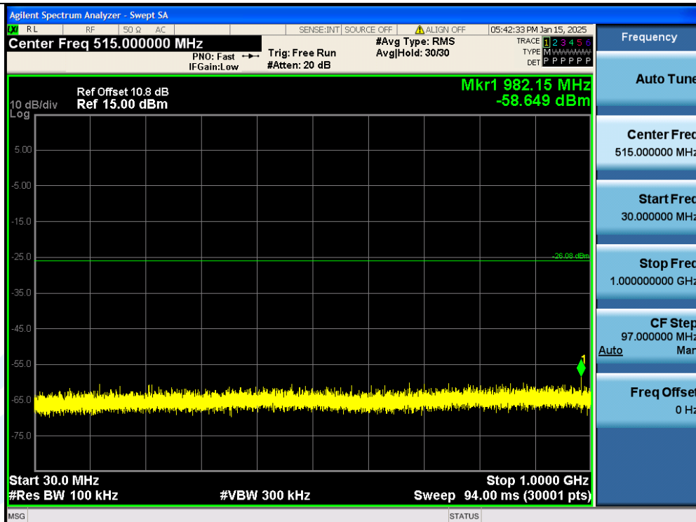
11N20SISO-Ant1-2467MHz-30~1000 MHz-PASS
