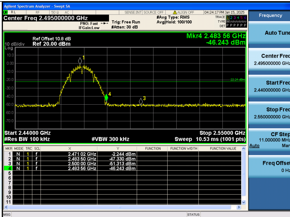
11B-Ant1-2472MHz-PASS
