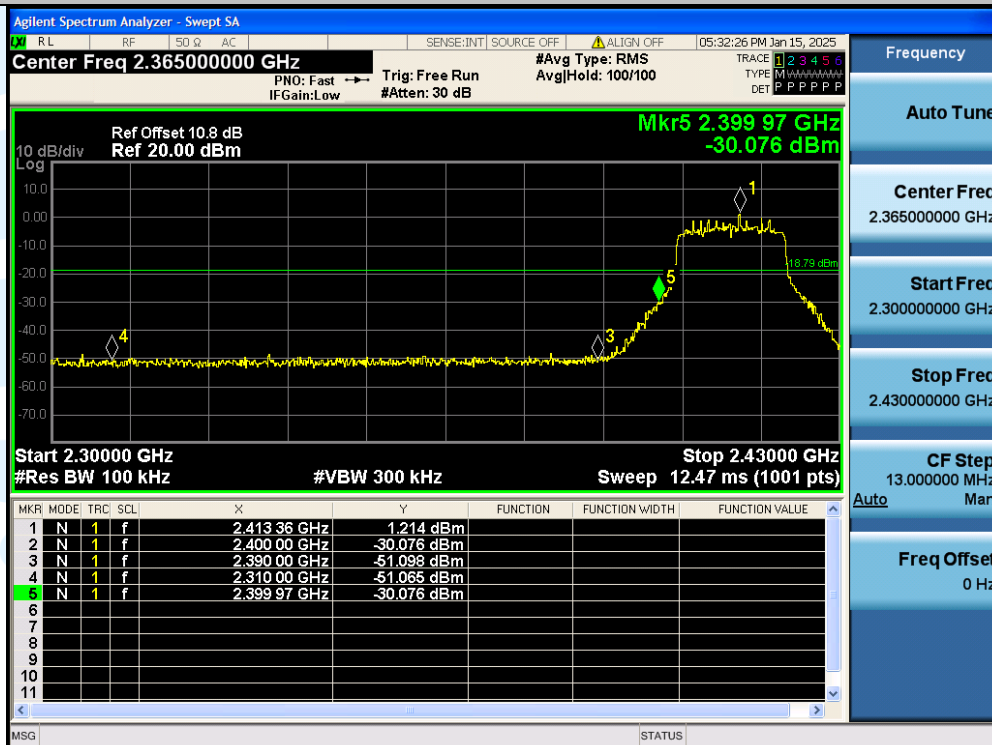
11N20SISO-Ant1-2412MHz-PASS
