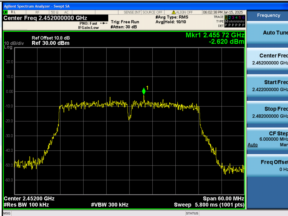
11N40SISO-Ant1-2452MHz-0~Reference-PASS
