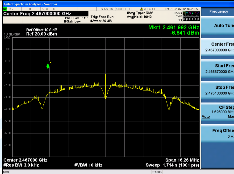
11B-Ant1-2467MHz-PASS
