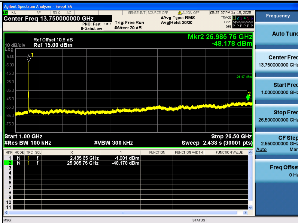
11N20SISO-Ant1-2437MHz-1000~26500MHz-PASS
