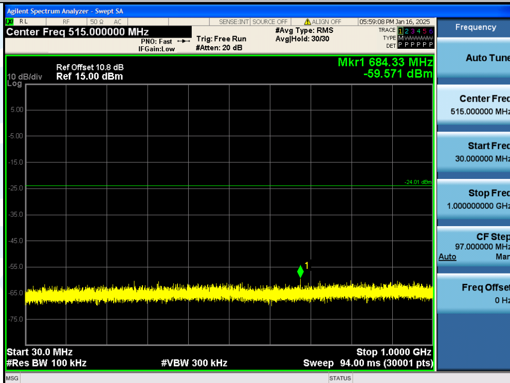
11G-Ant1-2437MHz-30~1000 MHz-PASS
