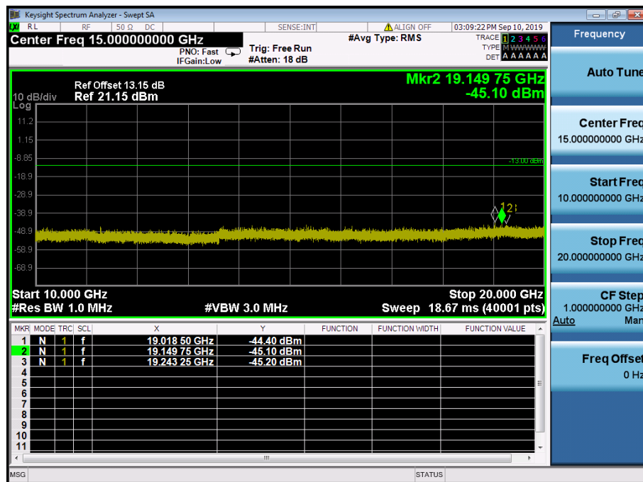
LTE Band 2 / 1.4MHz / QPSK - RB Size/Offset (1/2) – Mid Channel
