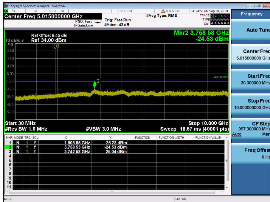
LTE Band 2 / 3MHz / QPSK - RB Size/Offset (8/7) – High Channel
