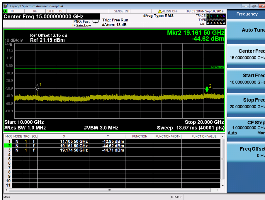
LTE Band 2 / 1.4MHz / QPSK - RB Size/Offset (3/3) – Low Channel
