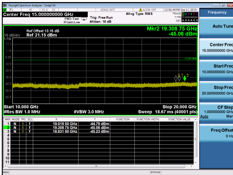
LTE Band 2 / 15MHz / 16QAM - RB Size/Offset (1/0) – Mid Channel
