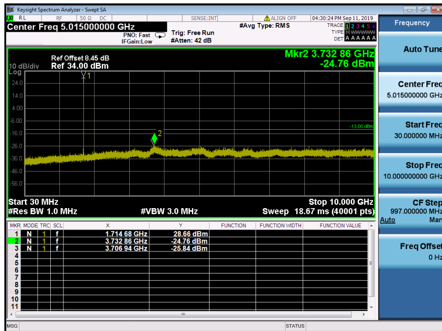
LTE Band 4 / 5MHz / QPSK - RB Size/Offset (1/24) – Low Channel
