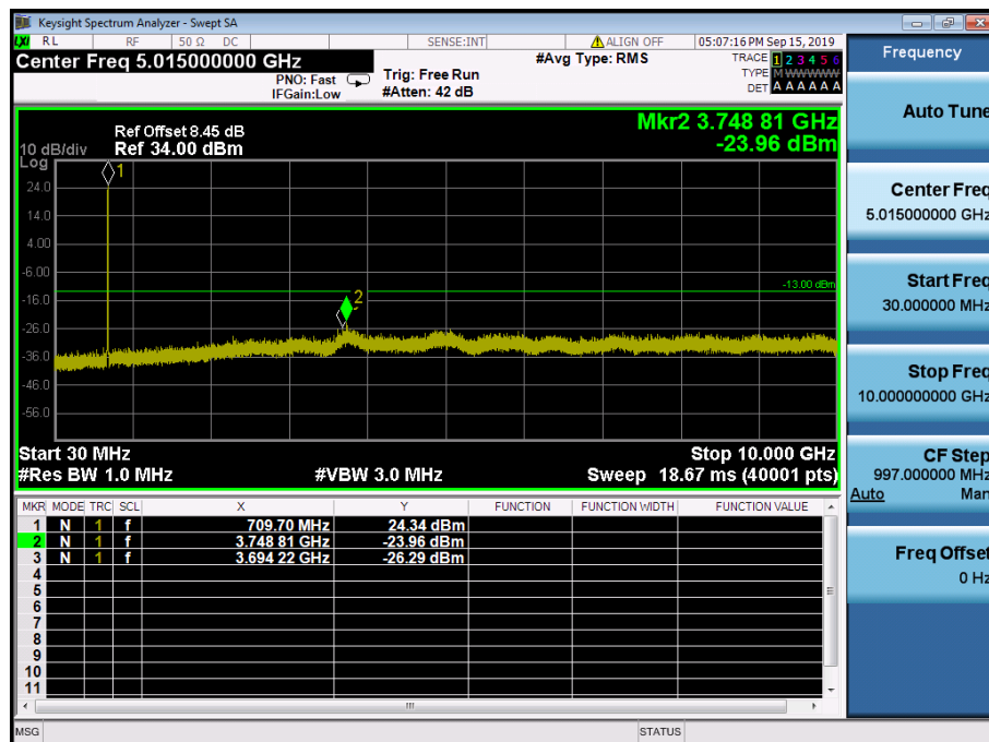
LTE Band 12 / 10MHz / 16QAM - RB Size/Offset (25/0) – High Channel
