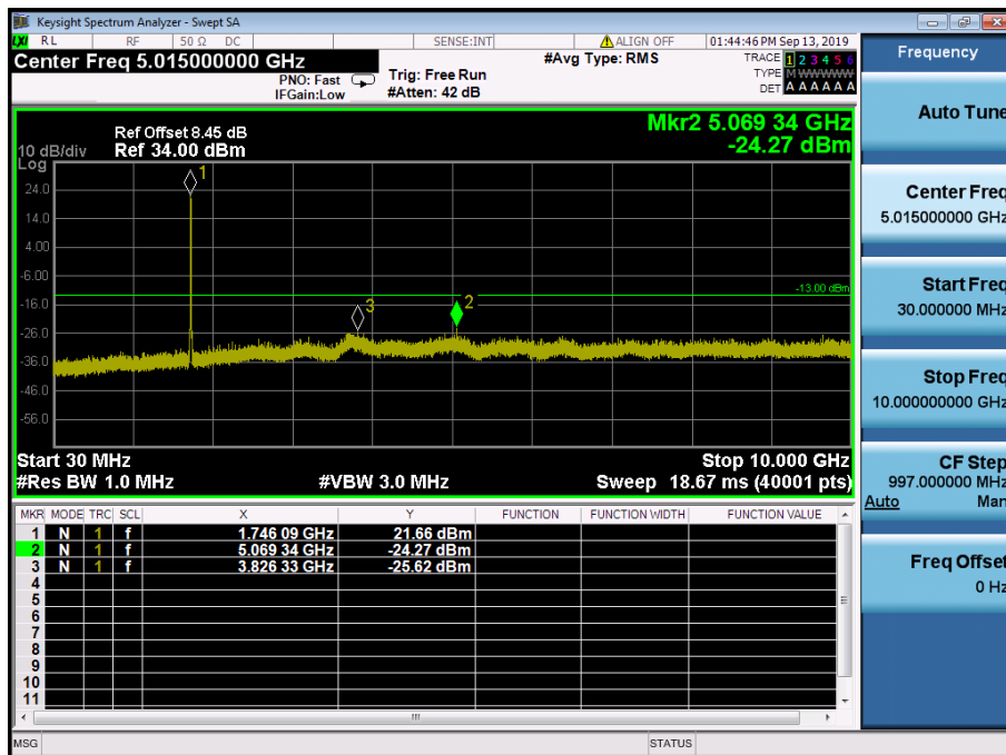
LTE Band 4 / 20MHz / 16QAM - RB Size/Offset (50/50) – High Channel
