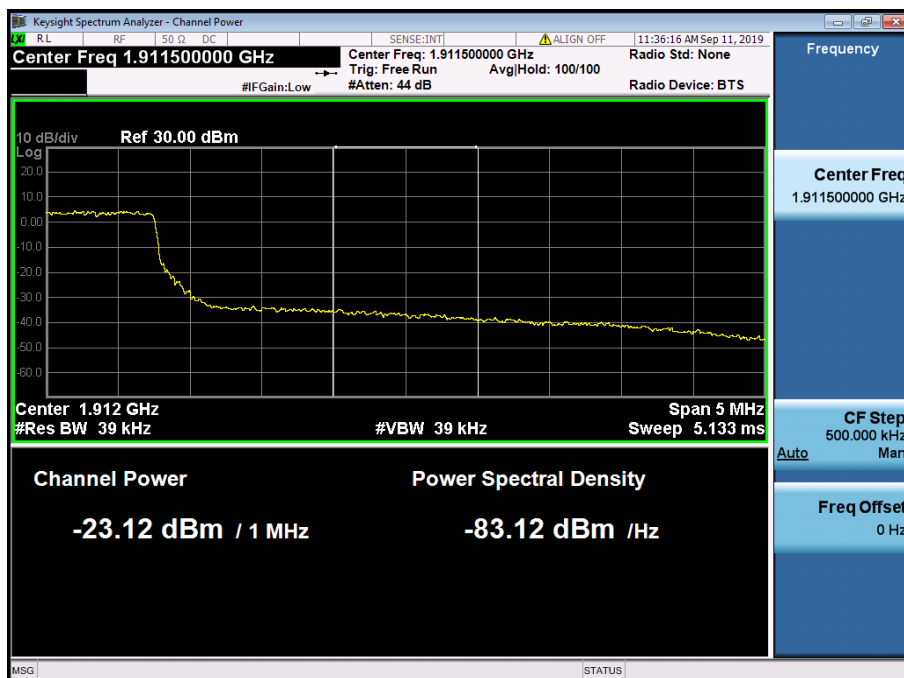
LTE Band 2 / 5MHz / 16QAM - RB Size/Offset (12/13)
