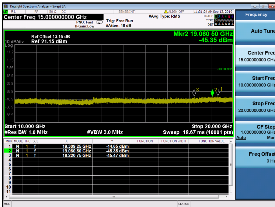
LTE Band 4 / 10MHz / 16QAM - RB Size/Offset (25/25) – Low Channel
