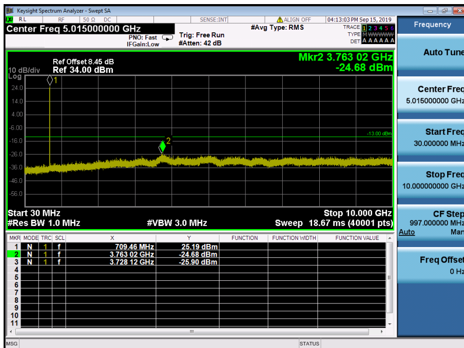
LTE Band 12 / 5MHz / 16QAM - RB Size/Offset (12/13) – Mid Channel
