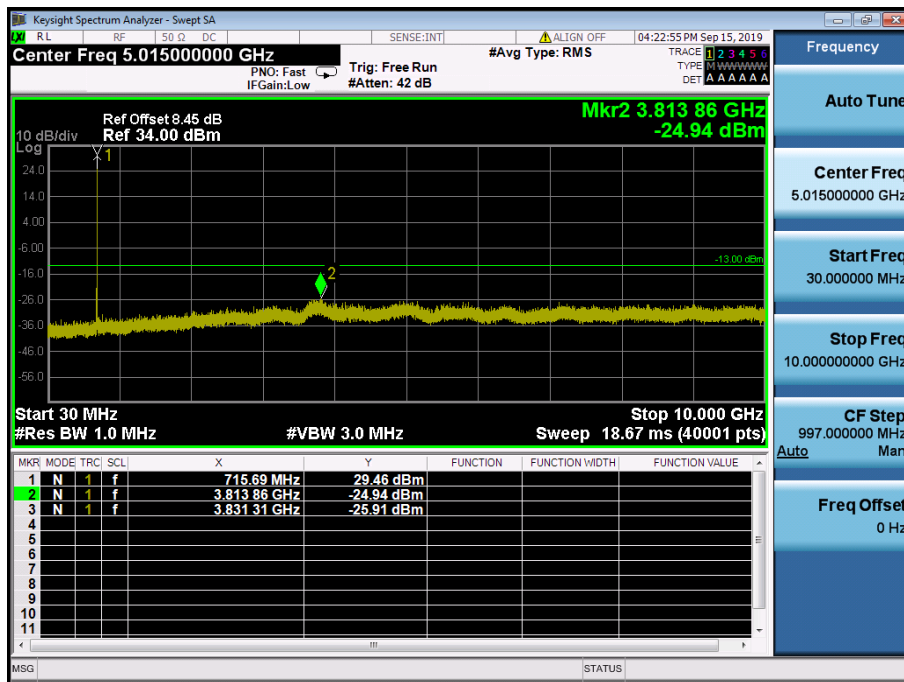
LTE Band 12 / 5MHz / 16QAM - RB Size/Offset (1/24) – High Channel
