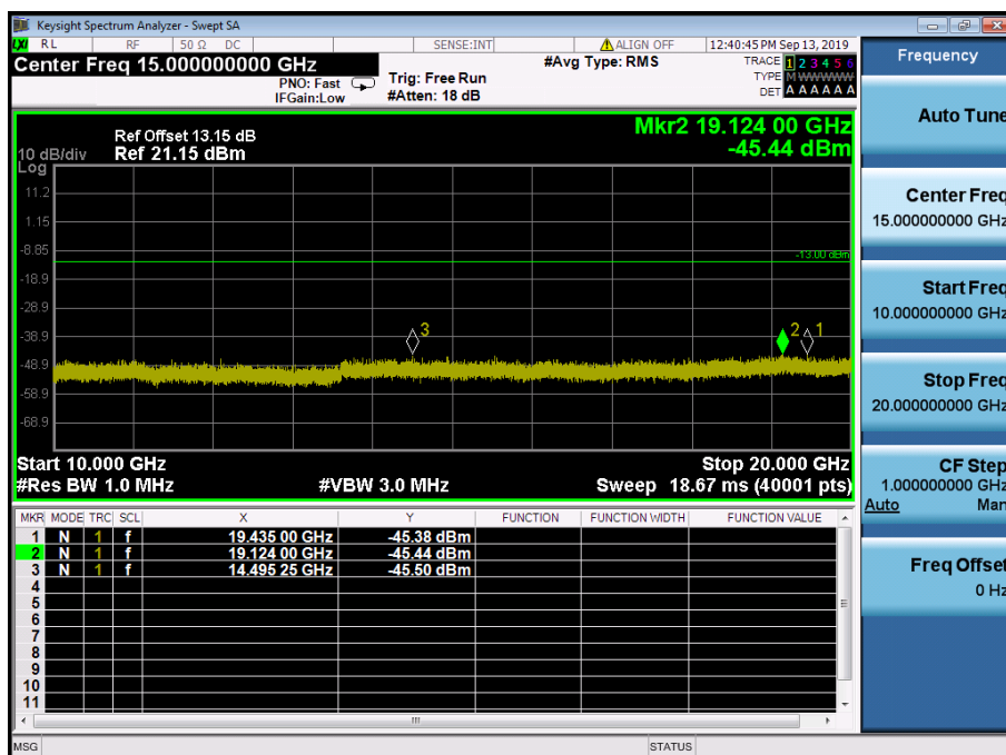
LTE Band 4 / 15MHz / 16QAM - RB Size/Offset (1/36) – High Channel
