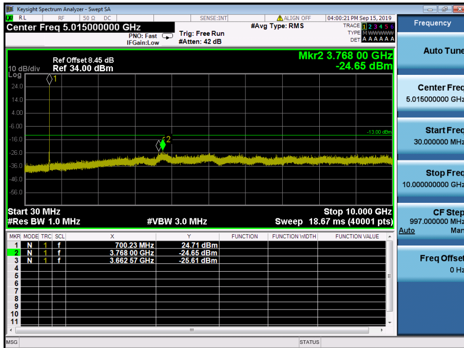
LTE Band 12 / 5MHz / 16QAM - RB Size/Offset (12/0) – Low Channel
