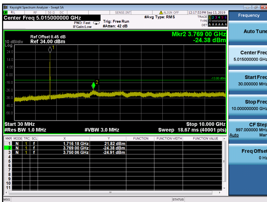
LTE Band 4 / 15MHz / 16QAM - RB Size/Offset (36/0)–Low Channel
