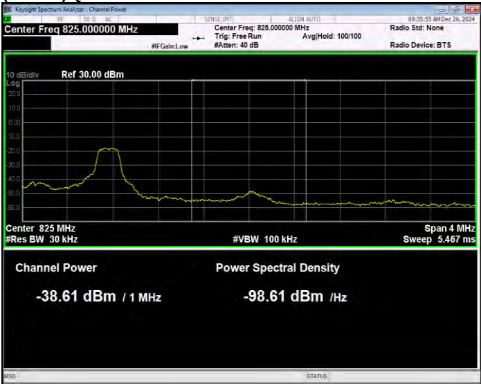
Band26(814-824) QPSK BW=3MHz Channel=26775 RB Size=1 Position=#0 Normal
