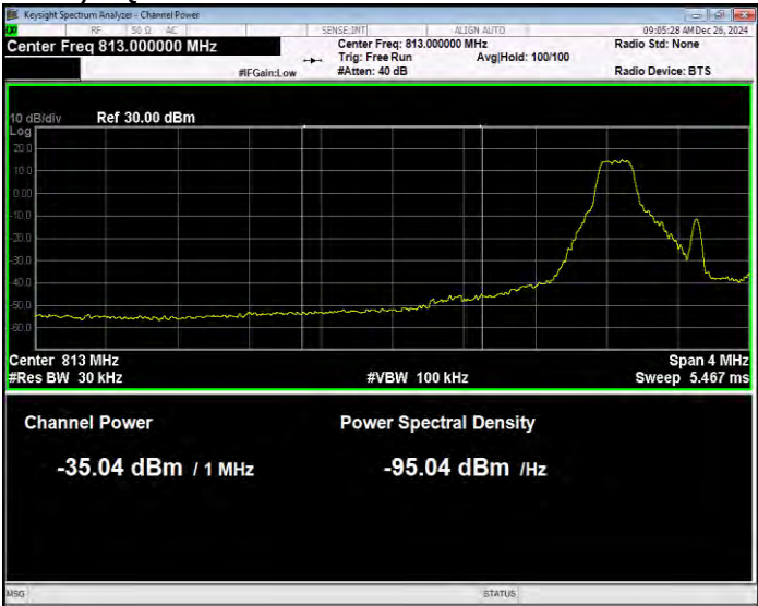
Band26(814-824) 16QAM BW=1.4MHz Channel=26697 RB Size=1 Position=#0 Normal
