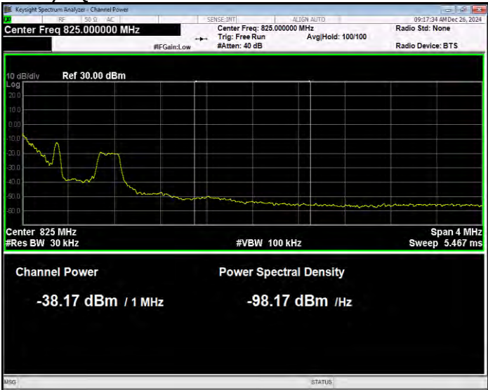
Band26(814-824) 16QAM BW=1.4MHz Channel=26783 RB Size=1 Position=#0 Normal
