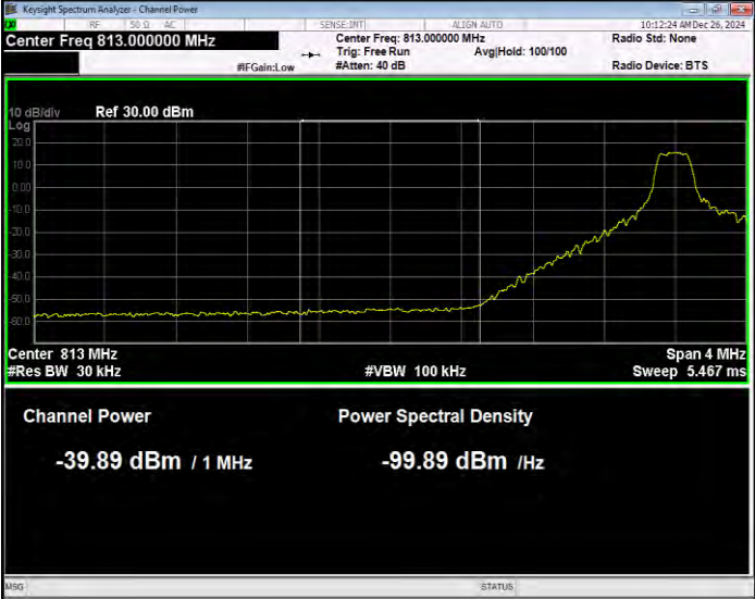
Band26(814-824) QPSK BW=10MHz Channel=26740 RB Size=1 Position=#0 Normal
