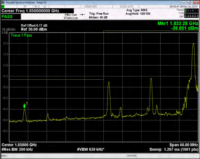
Band25 16QAM BW=20MHz Channel=26140 RB Size=100 Position=#0 Extended
