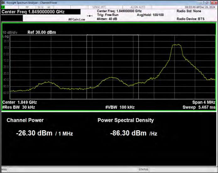
Band25 QPSK BW=3MHz Channel=26055 RB Size=1 Position=#0 Normal
