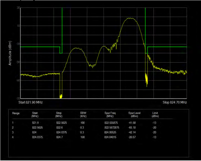
Band26(814-824) 16QAM BW=1.4MHz Channel=26783 RB Size=6 Position=#0 Extended
