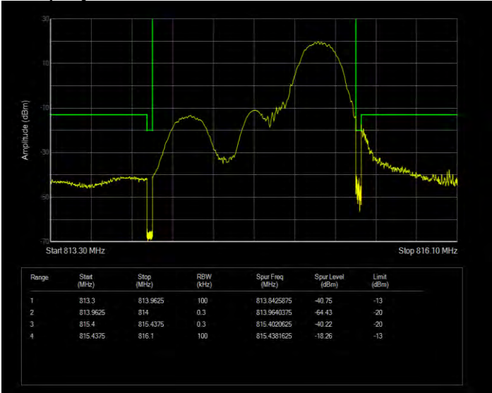
Band26(814-824) 16QAM BW=1.4MHz Channel=26697 RB Size=6 Position=#0 Extended
