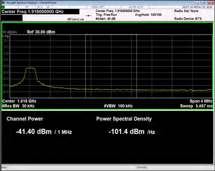
Band25 16QAM BW=10MHz Channel=26640 RB Size=1 Position=#0 Normal
