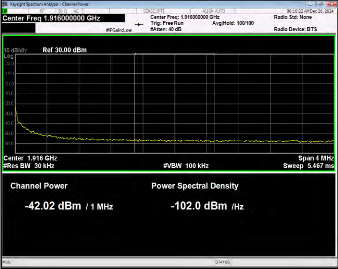
Band25 16QAM BW=20MHz Channel=26590 RB Size=1 Position=#0 Normal
