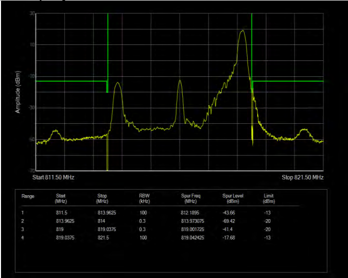
Band26(814-824) 16QAM BW=5MHz Channel=26715 RB Size=25 Position=#0 Extended
