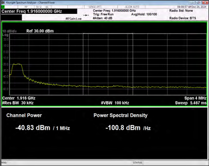
Band25 16QAM BW=15MHz Channel=26615 RB Size=1 Position=#0 Normal
