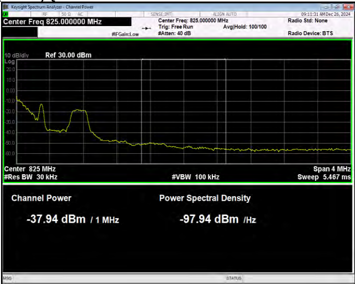
Band26(814-824) QPSK BW=1.4MHz Channel=26783 RB Size=1 Position=#0 Normal
