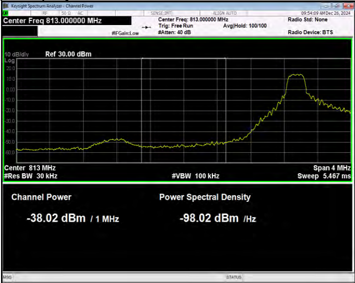
Band26(814-824) 16QAM BW=5MHz Channel=26715 RB Size=1 Position=#0 Normal
